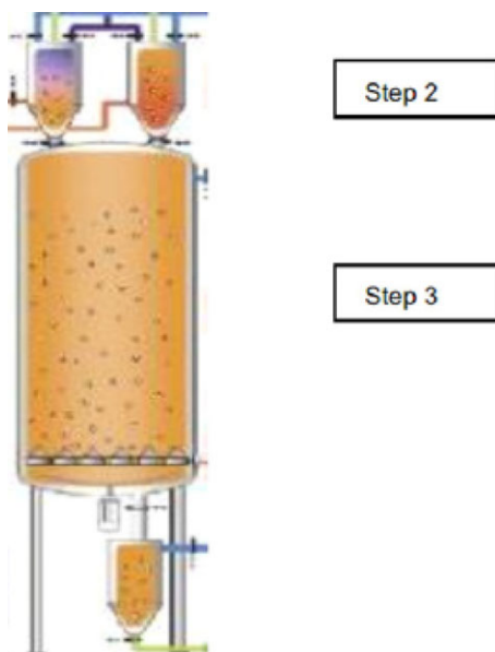
Figure 1: General scheme of the Starlinger Decon technology
