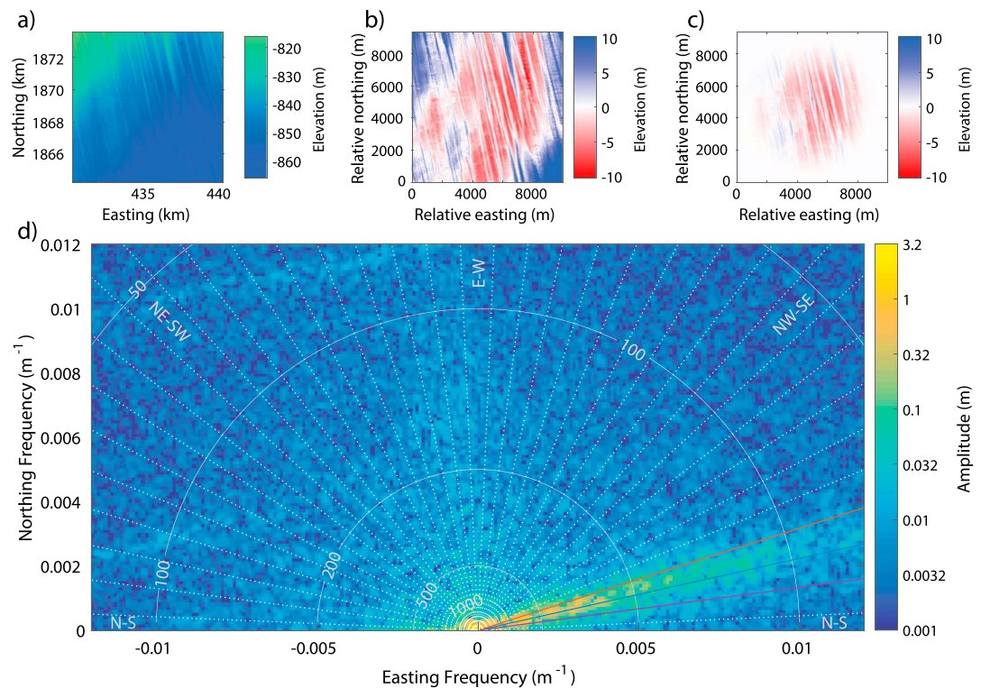
Figure 2. Example data and 2-D Fourier spectrum from the Pine Island (Antarctica) dataset, PI_MSLG_1. (a) Raw input data (elevation relative to the sea surface) sampled within a 10 × 10 km window. Raw depth observations have a resolution of 1 m. (b) Detrended data. (c) 2-D Hann-windowed and detrended data. (d) Frequency domain depiction of the data in Figure 2c. In Figure 2d, the background colors illustrate the average amplitude of topographic variations with specific easting and northing frequencies. The semicircular lines of equal wavelength (labeled in m) contour the frequency space. The lines extending radially from the bottom center at 5° increments represent features in the data with specific orientations. Cardinal and intermediate directions (e.g., NW-SE) for corrugation orientations are labeled. Most orientations are dotted white, whereas orientations with the largest amplitudes are colored for consistency with Figure 3. For this case, our quantitative approach (Figure 3) identifies that these MSGs trend 12.6°W of N, with maximum normalized wavelength \lambda (i.e., lateral spacing) of 690 m.
