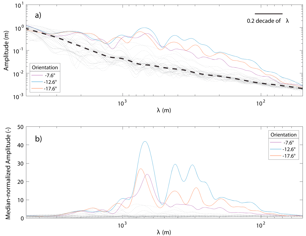
Figure 3. Topographic amplitude as a function of wavelength for orientations spaced every 5° for PI_MSGL_1. Each orientation is represented by a colored or gray dotted line. (a) Unnormalized amplitudes, with the median of all orientations shown by the black dashed line. Amplitudes are smoothed with a span of 1/5th decade of \lambda . (b) Amplitudes normalized by the median, demonstrating how much larger than the background spectra a certain feature (the MSGSLs, in this case) is. For Figures 3a and 3b, as well as in Figure 3, orientations with the largest normalized amplitudes are colored and labeled by their trends in the legend (orientations relative to north), whereas smaller normalized amplitudes are dotted gray. This representation shows that the MSGSLs with a -12.6^\circ W of N trend reach amplitudes up to 42 times higher than the median amplitude at a wavelength of 690 m.
