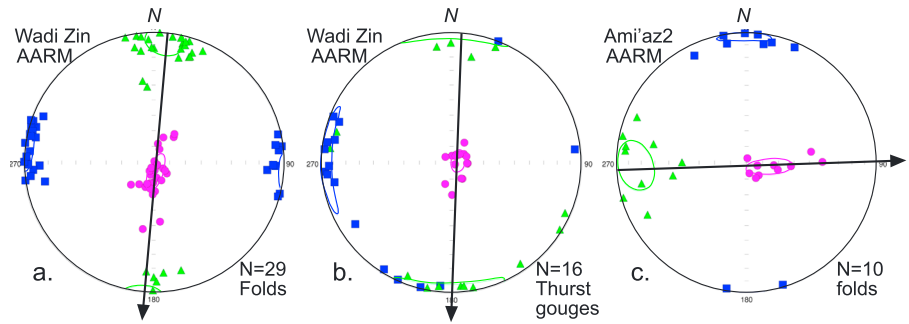
Figure 3. (a–c) Lower hemisphere, equal-area projection stereoplots of AARM principal axes, and the 95% confidence ellipses. The K_{R1} , K_{R2} , and K_{R3} axes are denoted by blue squares, green triangle, and pink circles, respectively. Stereoplot in Figure 3a is from the footwall syncline and hanging wall anticline in Wadi Zin. Stereoplot in Figure 3b is from gouge zone along thrusts in Wadi Zin. Stereoplot in Figure 3c is from the slump in Almog. The inferred transport direction is indicated by black arrows (see text).
