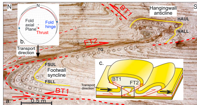
Figure 2. (a) Photo of fold-thrust systems in Wadi Zin (Figure 1b), showing the sampling scheme for the magnetic study. Specimens seen as circles in this cross section were taken from the footwall syncline (FSUL—upper limb; FSLL—lower limb), fault gouge zone (TG), and hanging wall anticline (HAUL—upper limb; HALL—lower limb) of the fold-thrust system. Dashed red lines mark the location of fore thrust (FT2) and back thrust (BT1). (b) Lower hemisphere, equal-area stereonet showing structural data from the fold-thrust system, and the inferred transport direction. (c) Three-dimensional cartoon illustrating the studied slump and the sequential relationships between the BT1 and the FT2 in this site. Black rectangle schematically represents the studied area in Figure 2a.
