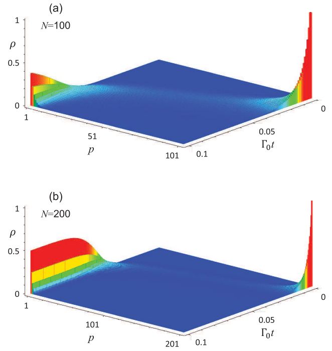
FIG. 2. Simulations with N atoms using the master equation (1) with the quantum dissipator (37) for the correlated two-level atoms and negligible matter interaction H_{\text{int}} . From Eq. (45), the relaxation time is approximately given by \tau_N = (N\Gamma_0)^{-1} . The initial state of the forms (32) and (33) at t = 0 is given by |0, N\rangle = |p = N + 1\rangle with all N atoms occupying the excited atomic level. During the dynamical evolution, the density matrix remains diagonal of the form (39) and relaxes into an inverse exponential profile represented by Eq. (48), yielding the asymptotic height of \rho_{p=1} = [N_{\text{gw}}(\omega_0)(1 - e^{-N/N_{\text{gw}}(\omega_0)})]^{-1} . The stochastic gravitational wave distribution function evaluated at the atomic transition frequency \omega_0 is chosen to be N_{\text{gw}}(\omega_0) = 1 . Accordingly, in plot (a) with N = 100 atoms, the initial state corresponding to the spike of height 1 at (p, \Gamma_0 t) = (101, 0) relaxes into an inverse exponential profile peaked at (p, \Gamma_0 t) = (1, 0.1) on a time scale of \tau_N = 0.01/\Gamma_0 . Similarly, in plot (b) with N = 200 atoms, the initial state corresponding to the spike of height 1 at (p, \Gamma_0 t) = (201, 0) relaxes into an inverse exponential profile similarly peaked at (p, \Gamma_0 t) = (1, 0.1) but on a halved time scale of \tau_N = 0.005/\Gamma_0 .
