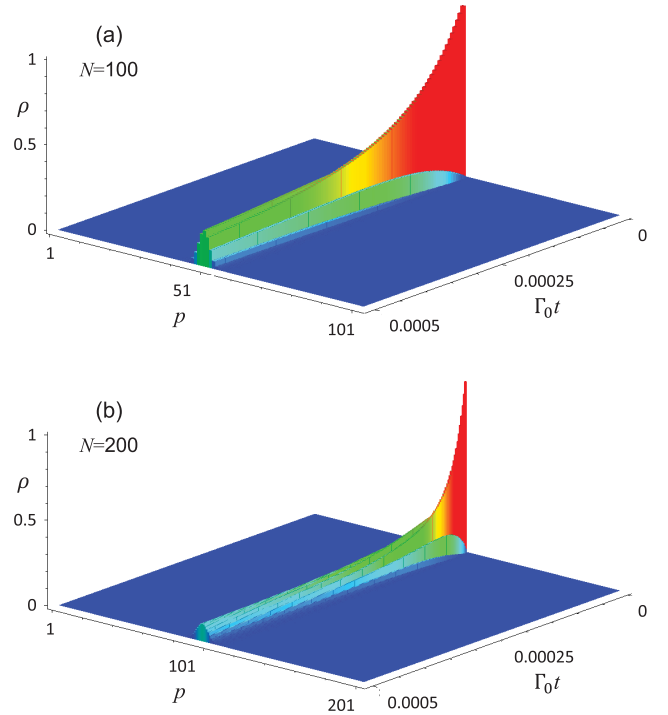
FIG. 4. Simulations of short-time collective transitions due to vacuum fluctuations of spacetime and additional stochastic gravitational waves with a chosen N_{\text{gw}}(\omega_0) = 1 . In plot (a) with N = 100 atoms, the initial state corresponds to the spike of height 1 at (p, t) = (50, 0) . While this state decays similarly to the descriptions in Fig. 4, its adjacent higher state with p = 51 is excited with an initial time scale of \tau_{\text{gw}} = 4/(N^2\Gamma_0 N_{\text{gw}}(\omega_0)) = 0.0004/\Gamma_0 according to Eqs. (60) and (62). In plot (b) with N = 200 atoms, the initial state corresponds to the spike of height 1 at (p, t) = (100, 0) . For a doubled N , its adjacent higher state with p = 101 is excited with a quarter of the preceding initial time scale with \tau_{\text{gw}} = 4/(N^2\Gamma_0 N_{\text{gw}}(\omega_0)) = 0.0001/\Gamma_0 .
