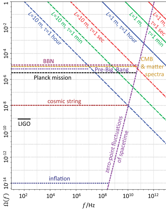
FIG. 1. Theoretical lower bounds for the spectral functions of stochastic gravitational waves \Omega(f) determined by Eq. (66) that could be detected using an ensemble of correlated two-level atoms contained in an off-resonant high- Q cavity of volume L^3 and measurement time \tau . Specifically, we consider helium-like atoms with atomic quantum numbers n_1 = n_2 = 2 , l_1 = l_2 = 1 , and -m_1 = m_2 = 1 , with a transition frequency induced by a Zeeman-type shift. For conventional stochastic gravitational waves, we have \Omega(f) = \Omega_{\text{gw}}(f) with \tau = \tau_{\text{gw}} , whereas for zero-point, i.e., vacuum, metric fluctuations, we have \Omega(f) = \Omega_{\text{vac}}(f) with \tau = \tau_{\text{vac}} introduced in this work by Eqs. (62) and (64). In both cases, we choose \tau = 1 sec, min, and h as possible (future) transition times for the atoms with L = 1 and 10 m in generating the above diagram. It suggests, for example, measuring the zero-point fluctuations of spacetime would require a 1 \text{ m}^3 cavity with a measurement time of 1 sec at f = 1 \text{ THz} approximately. Note that regions where the values of \Omega_{\text{gw}}(f) are below that of \Omega_{\text{vac}}(f) would present a less stochastic gravitational wave signal to the vacuum fluctuations “noise” ratio and hence the detection of the latter would be more likely using the discussed quantum methods. For comparison, we have superimposed the expected spectral functions of stochastic gravitational waves from various sources such as inflation, up to frequencies dominated by spacetime fluctuations, that may be detected by different methods such as LIGO from Ref. [21] and its references.
