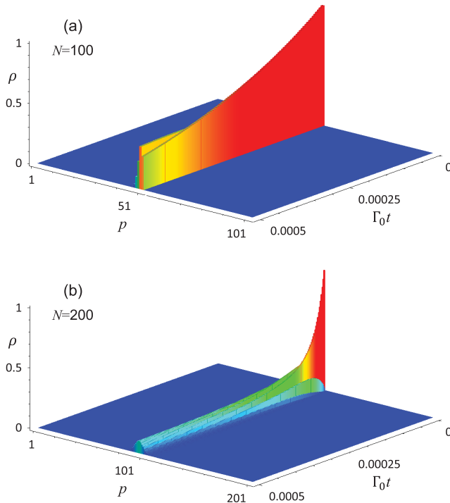
FIG. 3. Simulations of short-time collective spontaneous decays due to vacuum fluctuations of spacetime without additional stochastic gravitational waves so that N_{\text{gw}}(\omega_0) = 0 . In plot (a) with N = 100 atoms, the initial state corresponds to the spike of height 1 at (p, t) = (50, 0) . As shown, it decays into adjacent lower states with a relaxation time \tau_{\text{vac}} = 4/(N^2\Gamma_0) = 0.0004/\Gamma_0 according to Eqs. (61) and (62). In plot (b) with N = 200 atoms, the initial state corresponds to the spike of height 1 at (p, t) = (100, 0) . For a doubled N , this state decays into adjacent lower states with a quarter of the preceding relaxation time with \tau_{\text{vac}} = 4/(N^2\Gamma_0) = 0.0001/\Gamma_0 .
