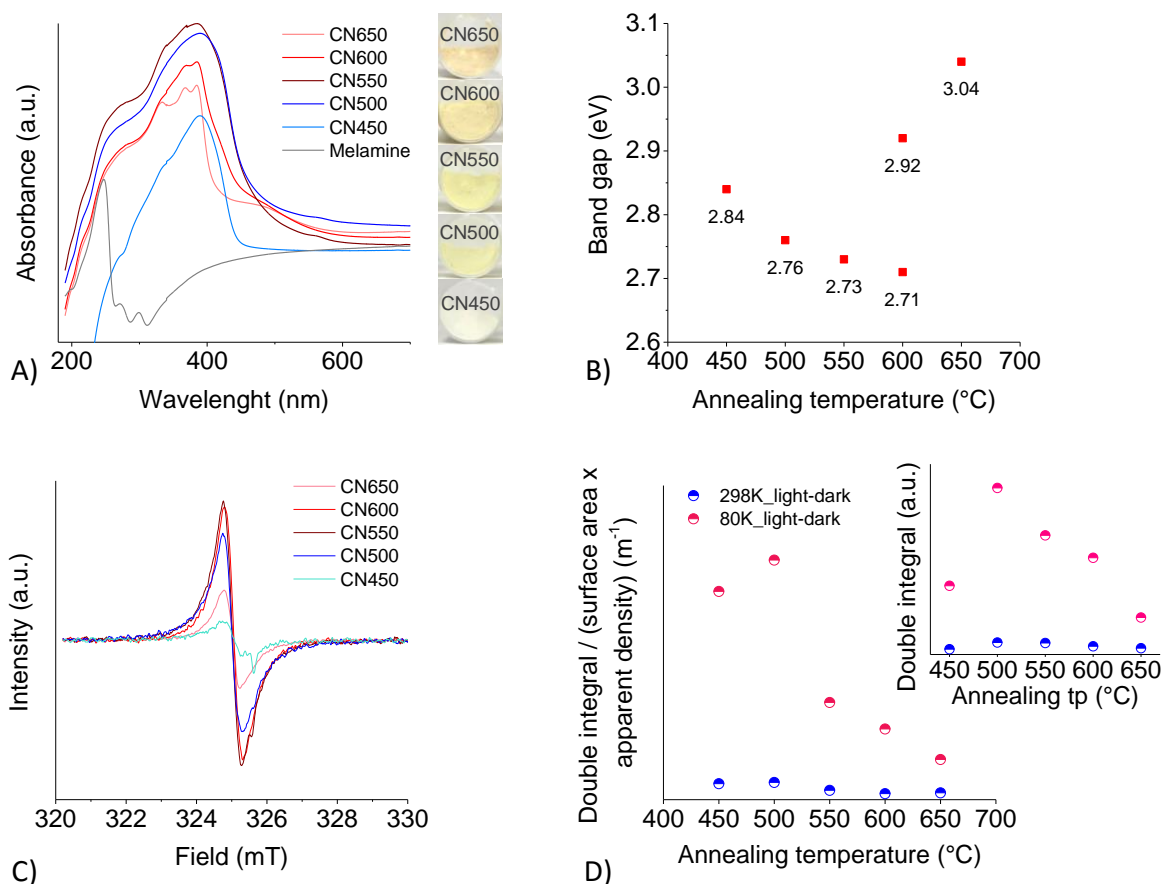
Figure 3 : A) UV-Vis Absorbance of the g-C 3 N 4 series. B) Extracted direct band gaps of the g-C 3 N 4 series. C) Lorentzian lines obtained by integration of electron paramagnetic resonance (EPR) absorption signal under 400nm light irradiation at room temperature. D) Doubly integrated EPR absorption signals under light irradiation at two different temperatures (80K and 298K), dark signal subtracted; data are normalized to the apparent density and the surface area of the samples.
