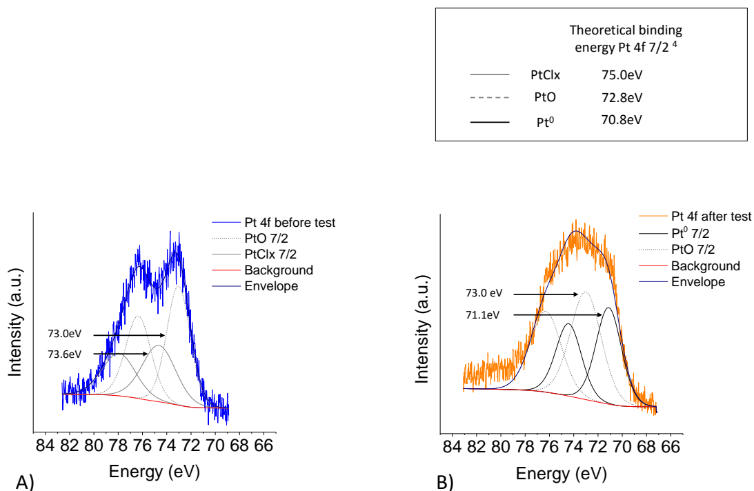
Figure S 2 :X-ray photoelectron spectroscopy of A) CN500 before photocatalytic test and B) CN500 after photocatalytic test using oxalic acid as sacrificial electron donor. A clear broadening of the Pt 4f peak towards lower binding energies is observed indicating the presence of Pt 0 after photocatalytic testing.
