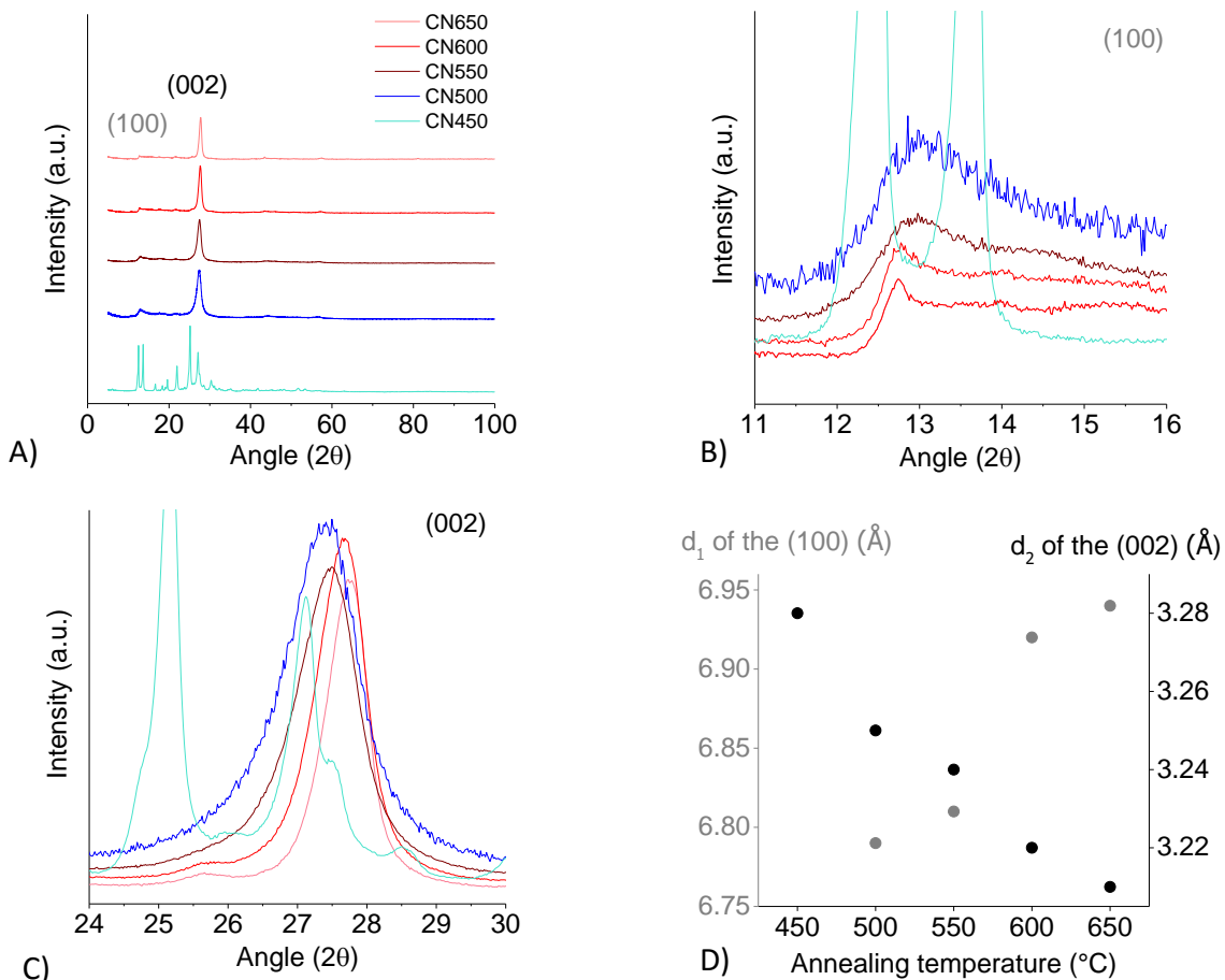
Figure 1: A) X-ray diffraction pattern of the g-C 3 N 4 samples synthesized at different temperatures, B) and C) Zoom in of the XRD pattern for the main reflections 2\theta_1 \sim 13^\circ and 2\theta_2 \sim 27^\circ and D) Evolution of the d-spacing for (100) and (002) with annealing temperatures
