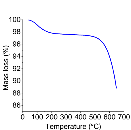
Figure S 1 : Thermogravimetric analysis of g-C 3 N 4 in air synthesized at 500 °C - CN500.
