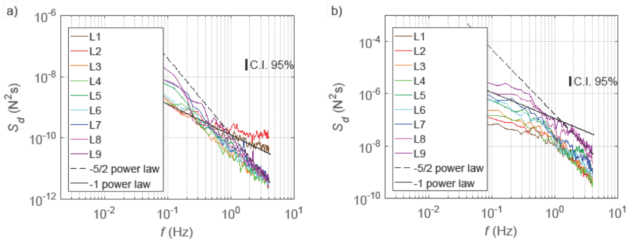
Fig. 4 The power spectral density functions of the drag force experienced by the seaweed blade models for flow scenarios ‘Run 1’ (a) and ‘Run 5’ (b). In both plots two slope lines (-5/2 and -1) are shown. The patterns displayed in (a) are representative of ‘Run 1’ and ‘Run 2’; the patterns displayed in (b) are representative of the remaining flow scenarios. The black rectangle at the top right corner of the plots represents the 95% confidence interval for the spectral magnitudes [3]
