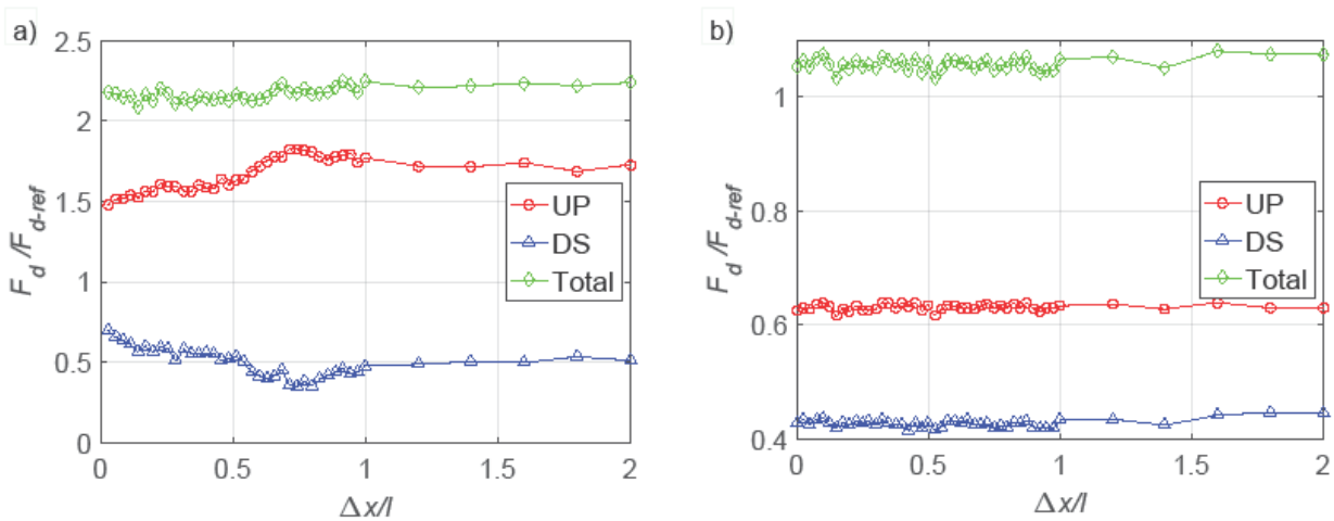
Fig. 11 Normalised mean drag force of a pair of blade models as a function of the nondimensional separation \Delta x / l between the blades: (a) scenario 'L1 Run 1P'; (b) scenario 'L7 Run 1P'. The plots display the normalised mean drag force experienced by the upstream blade ('UP'), the downstream blade ('DS') and the sum of these two quantities ('Total'); the patterns displayed in (a) and (b) are representative of flow scenario 'Run 2P' as well. Normalisation is achieved using the mean drag force F_{d-ref} experienced by a single (isolated) blade model at the same hydraulic conditions
