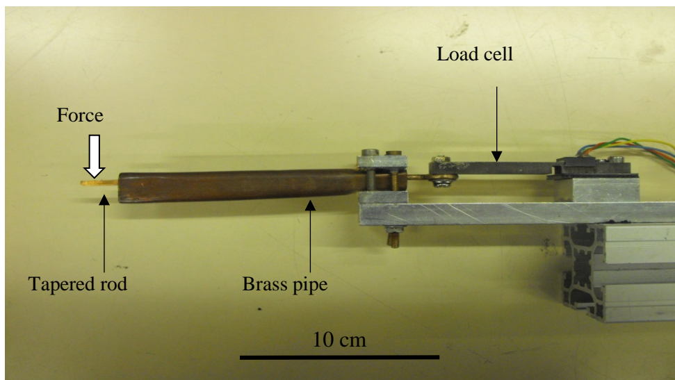
Fig. 2 Detail of the custom-made DMD displaying the tapered copper rod, protective brass pipe, and load cell mounted on the aluminium support. The tapered rod was connected to the load cell and mounted on the support so that it would not touch the protective pipe during the experiments
