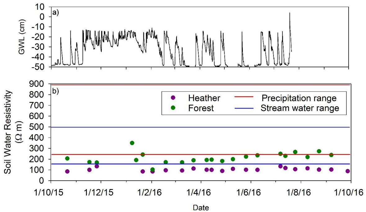
Fig. 3: a) Groundwater level (GWL) for the heather site, and b) estimated soil water resistivity values
