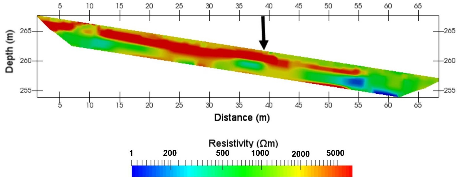
Fig. 4: Resistivity for the 72 m long transect through the forest hillslope, showing high resistivity scree material in the shallow subsurface. Black arrow indicates location of plot and transect.
