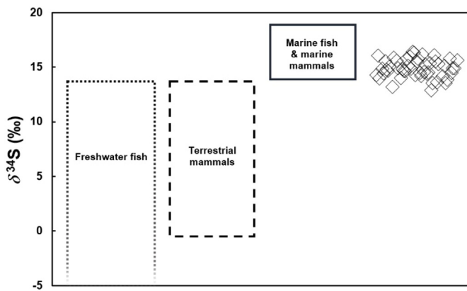
Fig. 4. Human sulphur isotope data from Nunalleq, plotted with general baseline approximations for freshwater, terrestrial and marine ecosystems (based on Nehlich and Richards, 2009; Nehlich, 2015). Measurement error was \pm 0.5\% ( 1\sigma ).
