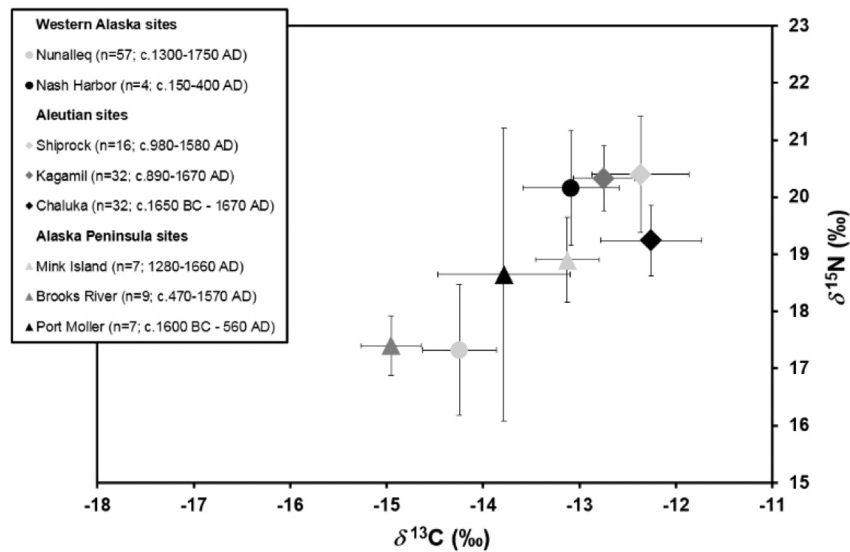
Fig. 8. Mean stable carbon and nitrogen isotope data ( \pm 1\sigma ) of bone collagen from a range of Aleutian and Alaskan sites/assemblages from previous publications (Coltrain, 2010a, b; Byers et al., 2011). Values from human hair from Nash Harbor (Britton et al., 2013) and Nunalleq (Britton et al., 2013, and this study) have been adjusted to a predicted mean bone collagen value (based on O’Connell et al., 2001) for comparative purposes.
