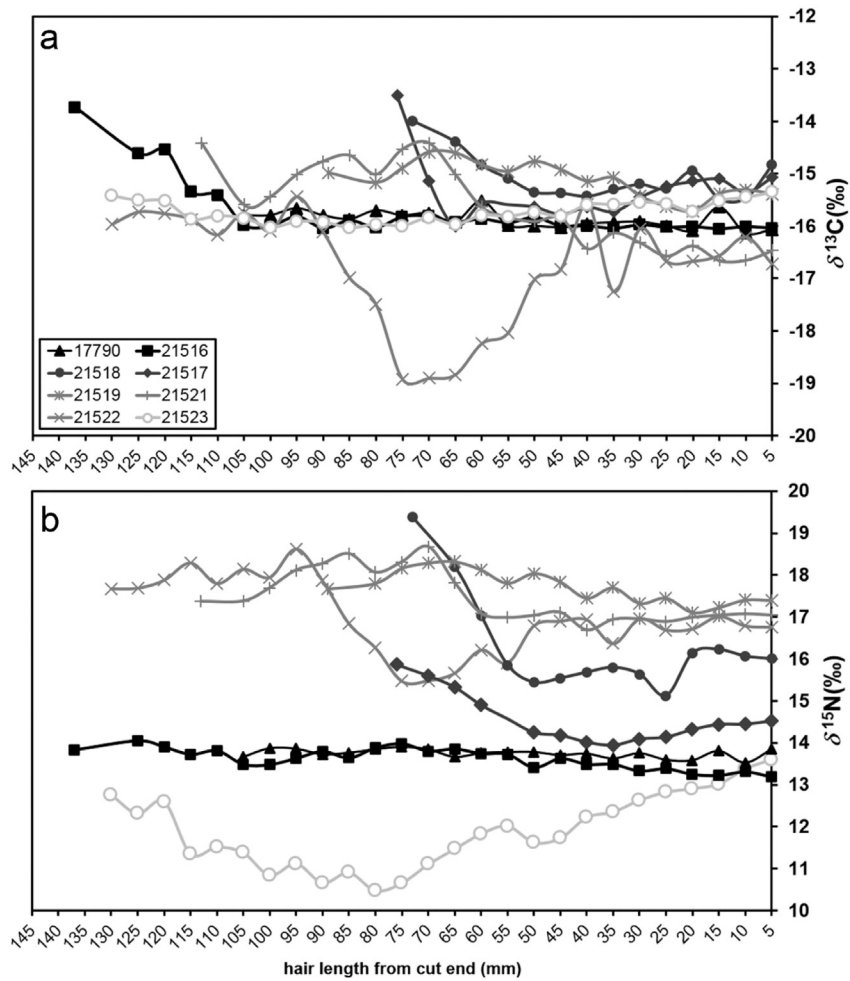
Fig. 7. a–b: Carbon (a) and nitrogen (b) isotope values of sequentially-sampled human hair from the Nunalleq site. Measurement error was 0.2‰ (1σ) or better.
