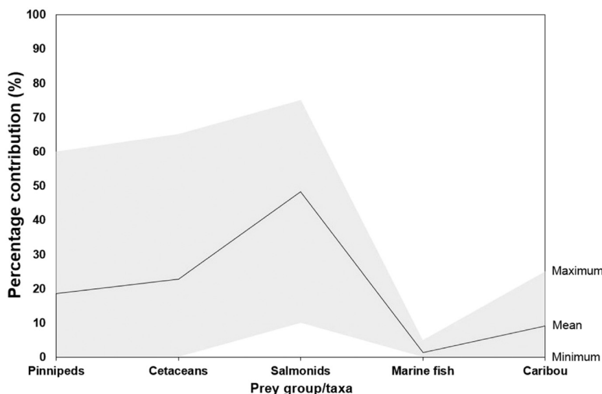
Fig. 3. Summary IsoSource mass balance data for Nunalleq, showing minimum, maximum and mean proportional contributions to the diet of major prey taxa groups.
