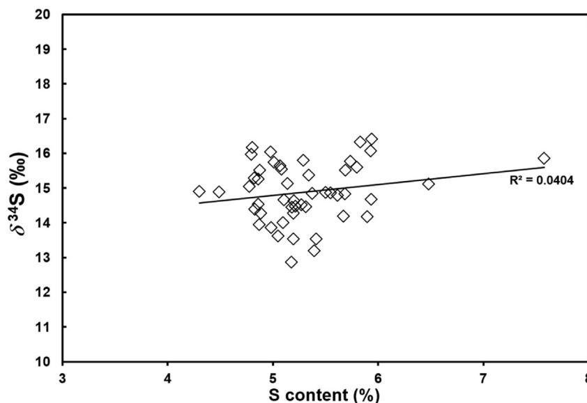
Fig. 5. Sulphur isotope ratios and sulphur content of human hair from the Nunalleq site. Measurement error was \pm 0.5\% ( 1\sigma ).
