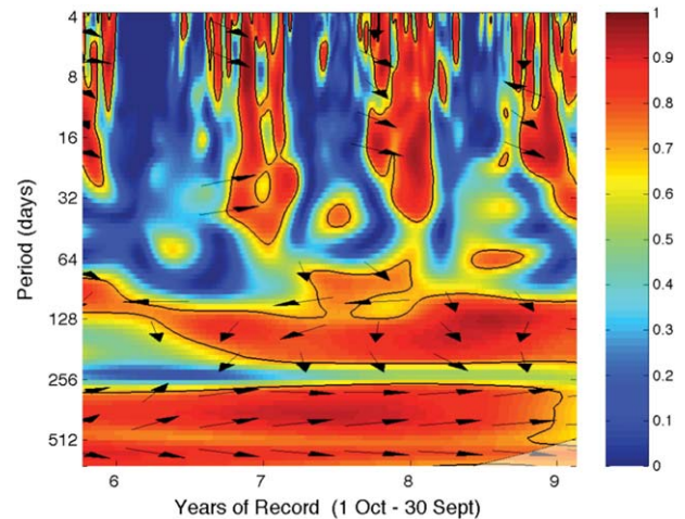
Figure 6. Close-up of squared wavelet coherence between precipitation and discharge for Krycklan for \sim 3 years of record. For interpretation of figure, see Figure 4.
