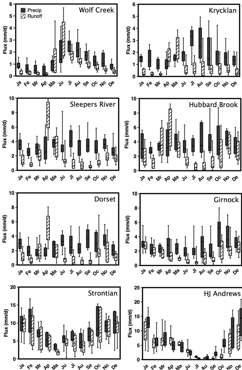
Figure 2. Ten year box-and-whisker monthly precipitation and runoff for the study sites. Whiskers extend to the 10th and 90th percentile. Precipitation is displayed as recorded at the site.
