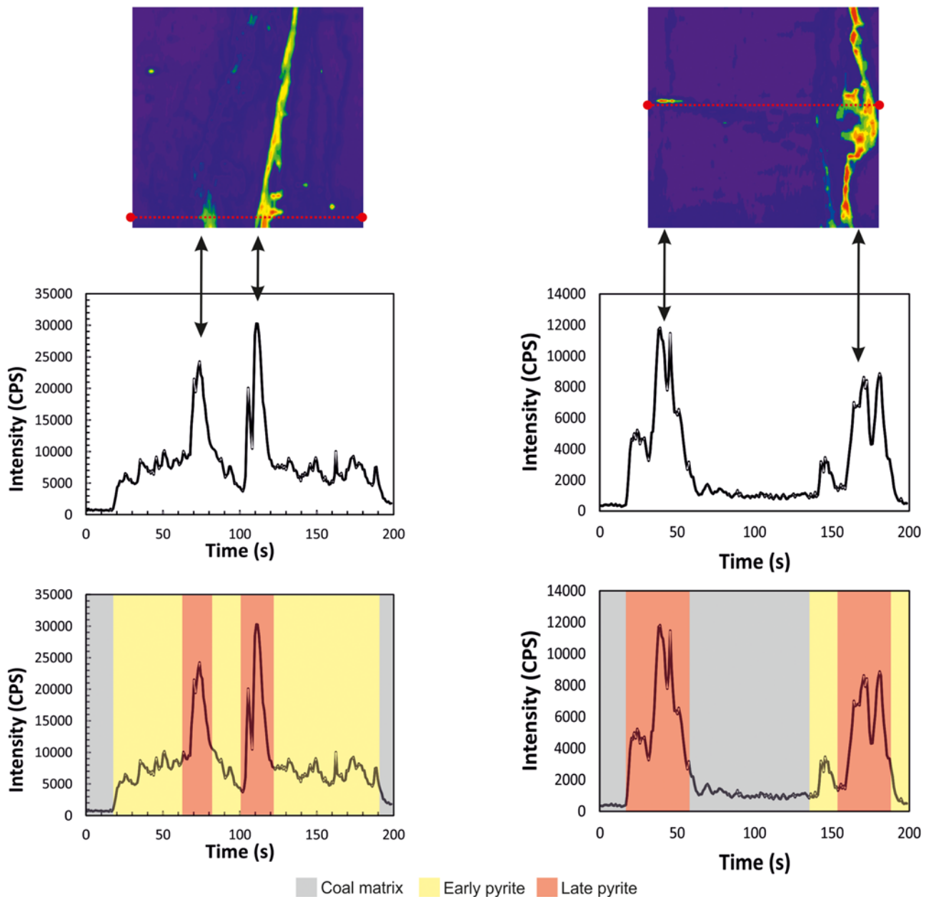
Fig. 5. Se LA-ICP-MS maps and corresponding line scan transects showing Se peak intensity. Large Se peaks correspond to cleat-filling pyrite perpendicular and parallel to banded pyrite.
