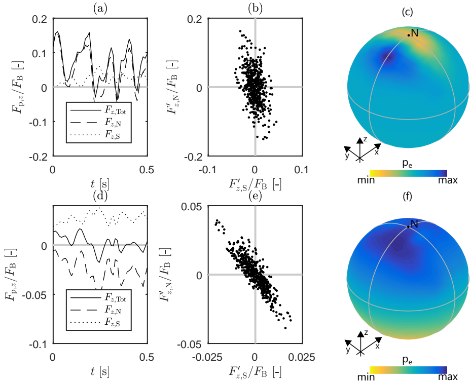
FIGURE 9. (a) Pressure lift signal for the top particle, with a decomposition of North and South hemisphere contributions. (b) North-South quadrant analysis. (c) Mean pressure on the particle surface. Analogous results for a reference particle located inside the bed are shown in panels (d,e,f).
