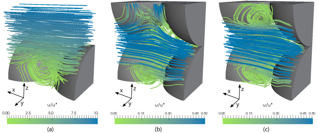
FIGURE 4. Structure of the average flow within and directly above the pores, shown from a section cutting halfway the pore in the xz plane. (a) Flow directly above the bed. (b) The first layer of pores, in direct communication with the ambient fluid. Note the streamlines coming in and out of the pore from above. (c) Deep pores.
