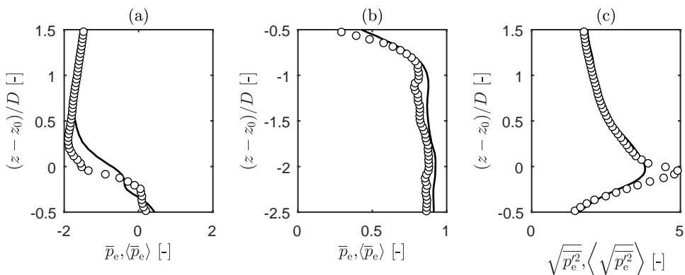
FIGURE 6. Mean dimensionless excess pressure \bar{p}_e (a) above the bed and (b) inside the first two layers of pores. (c) Pressure fluctuations at the surface-subsurface interface. Legend as in figure 3.
