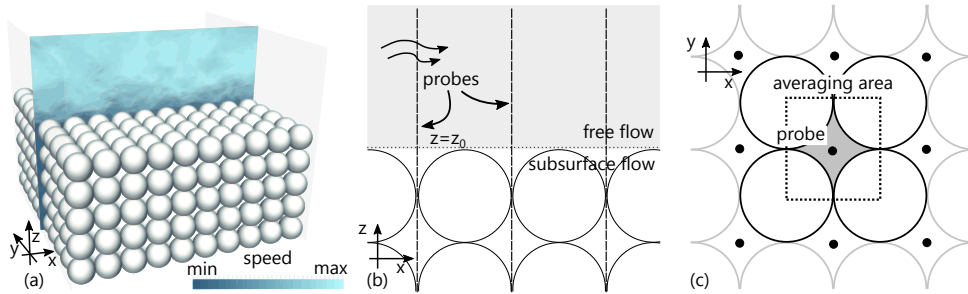
FIGURE 1. (a) Illustration of the study case. Description of the probe lines and of the averaging area viewed (b) from the side and (c) from the top.
