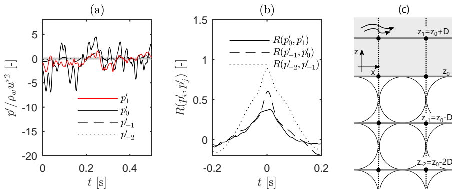
FIGURE 8. Pressure fluctuations: (a) Sample of pressure signals at different pore levels and in the surface flow. (b) Normalized cross-correlations between the signals at different pore levels, and between the pores and the surface flow. (c) Location of the pore levels and of the top central tracer.
