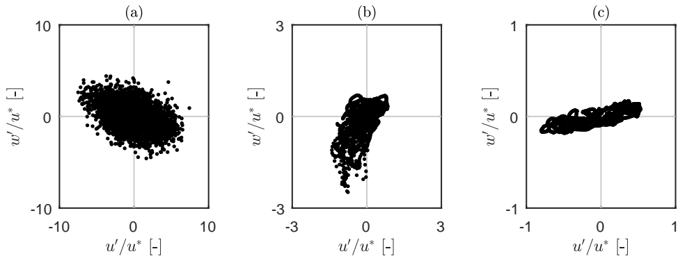
FIGURE 5. Quadrants analysis of turbulent events recorded (a) at the edge with the surface flow ( z = z_0 ), (b) at the center of the first pore ( z = z_0 - D ), and (c) at the center of the second layer of pores ( z = z_0 - 2D ). The graphs illustrate the events measured throughout 10^5 time steps ( \sim 7 s), but only one point every 200 time steps is shown for clarity.
