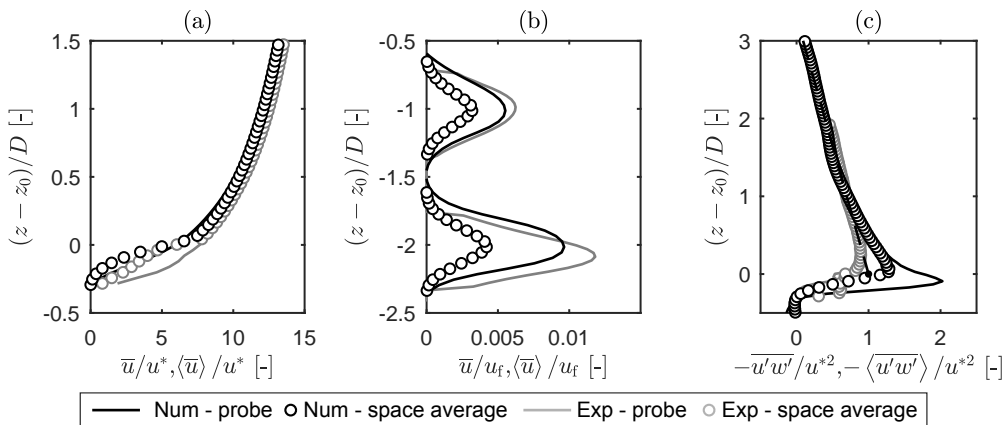
FIGURE 3. Mean streamwise velocity \bar{u} (a) above the bed and (b) inside the first two layers of pores. (c) Scaled Reynolds stresses above the bed, with the linear interpolation used to compute u^* . Black symbols in the plots show the numerical results, whereas gray lines and markers refer to the experiments of Pokrajac & Manes (2009).
