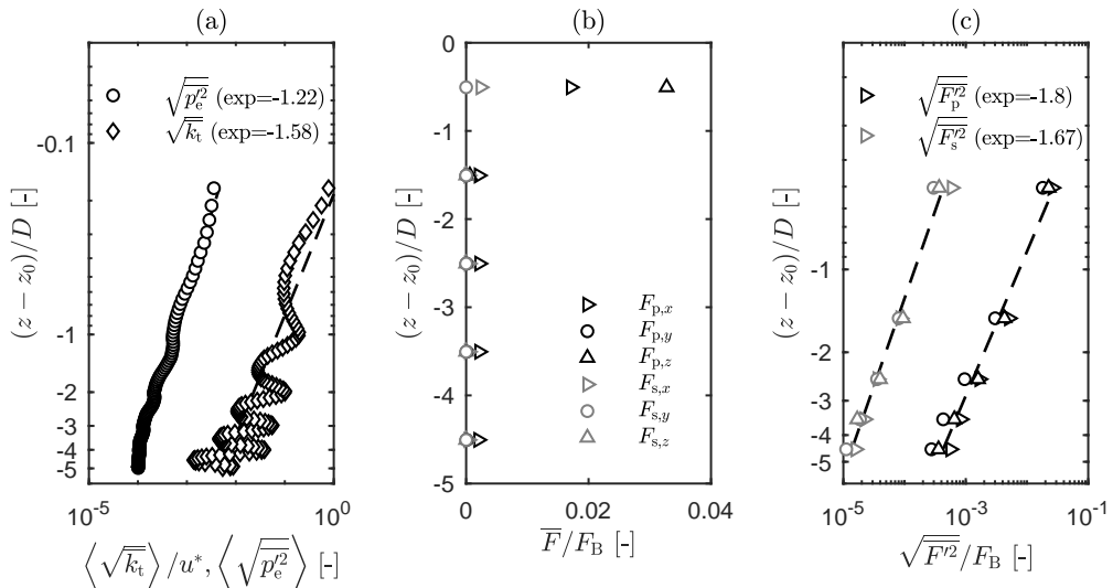
FIGURE 7. (a) Decay of mean turbulent kinetic energy \bar{k}_t and mean pressure fluctuations \sqrt{p^{\prime 2}} with depth. Both axis are in logarithm scale. (b) Mean shear force \bar{F}_s and pressure force \bar{F}_p exerted on the particles, as a function of depth. (c) Shear and pressure force fluctuation intensities on the particles, as a function of depth.
