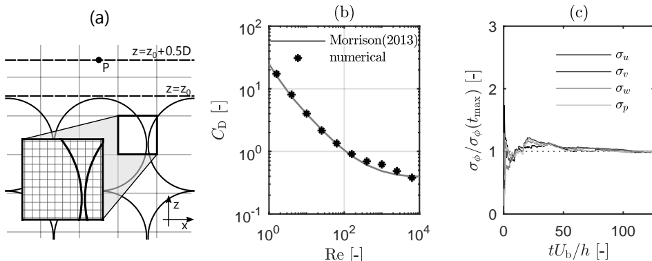
FIGURE 2. Details of the simulation procedure (a) The discretization grid, illustrated using 10 \times 10 element boxes for clarity. One box is magnified to show the actual grid. (b) Drag coefficients computed using the test simulation with a single particle immersed in a channel flow. (c) Convergence of second moments during the simulation, computed using Eq. 3.1 at point P, as shown in panel (a).
