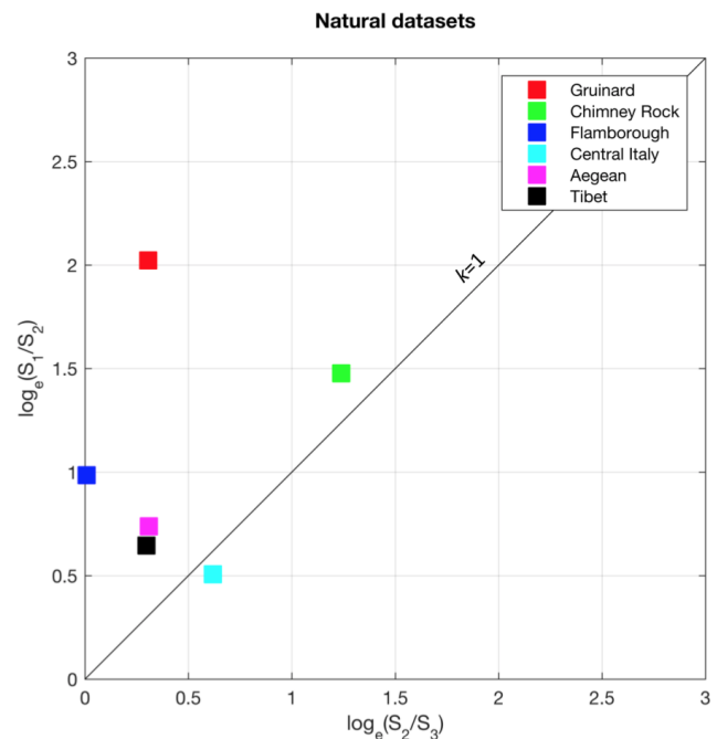
Figure 7. Eigenvalue ratio plot for the natural datasets shown in Fig. 5. All but one dataset (central Italy) lie above the line for k = 1 . The best-constrained quadrimodal fault dataset (Gruinard) has the highest ratio of \log_e(S_1/S_2) .
