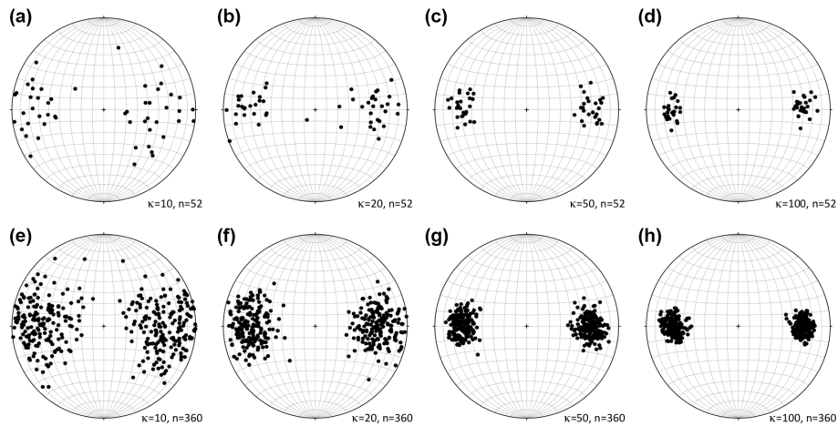
Figure 3. Stereographic projections (equal area, lower hemisphere) showing the eight synthetic datasets designed to model conjugate (bi-modal) fault patterns in this study. (a–d) Synthetic fault datasets derived from equal mixtures of two Watson distributions with mean pole directions separated by an inter-fault dip angle of 60^\circ . These models represent a “low fault count” scenario, with n = 52 and \kappa (the Watson dispersion parameter) varying from 10 to 100. (e–h) These models represent a “high fault count” scenario, with n = 360 and \kappa varying from 10 to 100.
