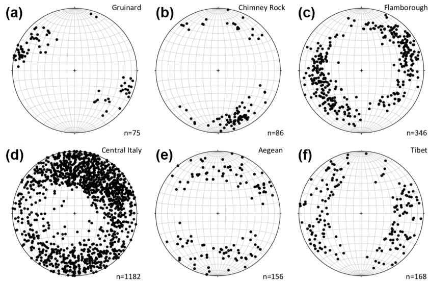
Figure 5. Stereographic projections (equal area, lower hemisphere) showing the six natural datasets used in this study. All plots show poles to faults, the majority of which are inferred to be normal. (a) Data from deformation bands measured in faulted Triassic sandstones at Gruinard Bay, Scotland (Healy et al., 2006a, b). (b) Data from faults and measured in sandstones at Chimney Rock in the San Rafael Swell, Utah, USA. Data digitised from Krantz (1989). (c) Data from faults measured in cliffs of Cretaceous chalk at Flamborough Head, NE England. Data digitised from Peacock and Sanderson (1992). (d) Data from faults measured in the Apennines of central Italy. Data digitised from Roberts (2007). (e) Data from focal mechanism nodal planes derived from the CMT catalogue for the Aegean region (Ekström et al., 2012). (f) Data from focal mechanism nodal planes derived from the CMT catalogue for the Tibet region (Ekström et al., 2012).
