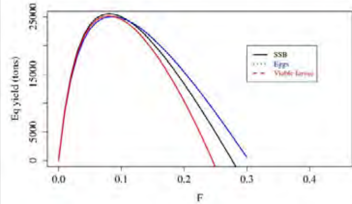
BSAI POP equilibrium yield graphs
