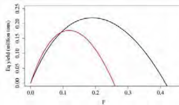
GOA walleye pollock example equilibrium yield graphs
