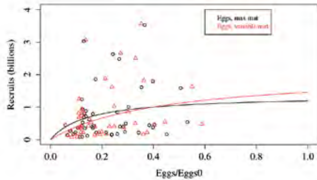
GOA walleye pollock example SR graphs
