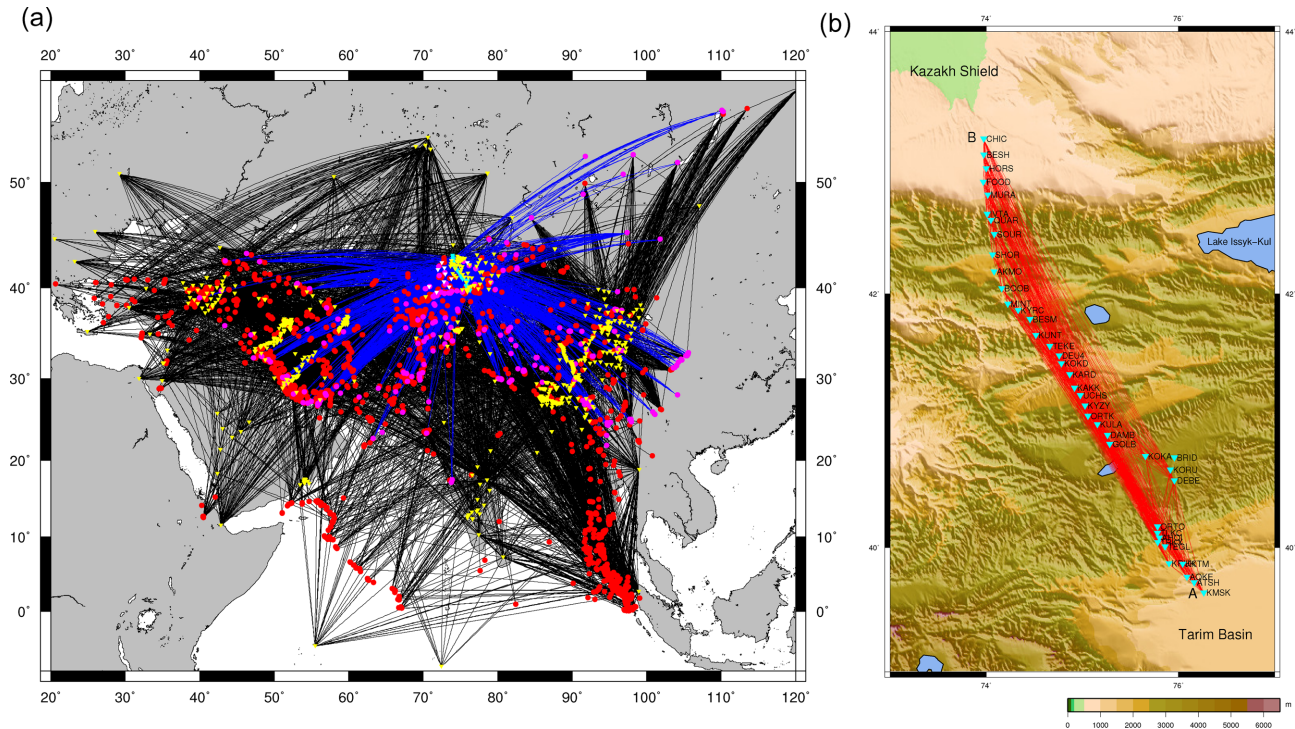
Figure 4. (a) Paths between stations and earthquakes used to generate path average Rayleigh wave dispersion curves. Blue lines are this study and black lines are from Nunn et al. (2014); Acton et al. (2010); Rham (2009). (b) Paths used to generate Rayleigh wave group velocity dispersion curves from the cross-correlations of ambient noise data between station pairs.
