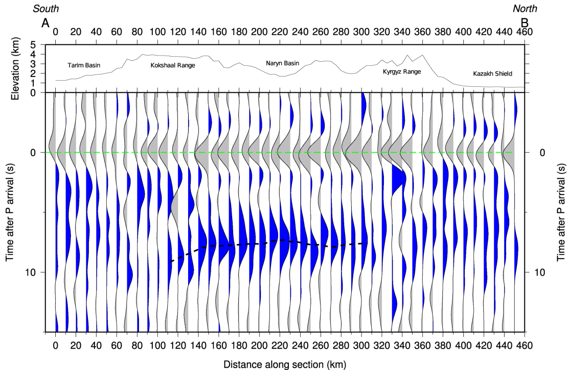
Figure 7. Stacked S receiver functions. Time and amplitude reversed to allow for easy comparison with PRFs. Coherent S -to- P conversion can be seen in the middle of the range at arrival times of 7 and 9 s which agree with conversion seen in the PRFs. These are likely to be conversions from the Moho.
