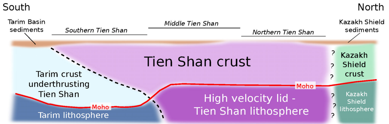
Figure 15. Cartoon summarizing the key interpretations of this study. The Tarim crust is underthrusting the Tien Shan from the south. The northward extent of the underthrusting of the the Tarim crust coincides with the boundary observed at the surface between the Southern and Central Tien Shan terranes. Underthrusting is responsible for thickened crust beneath the southern Tien Shan. A high velocity lid in the upper mantle is found beneath the central and northern Tien Shan. The depth of the Moho in this region does not vary significantly.
