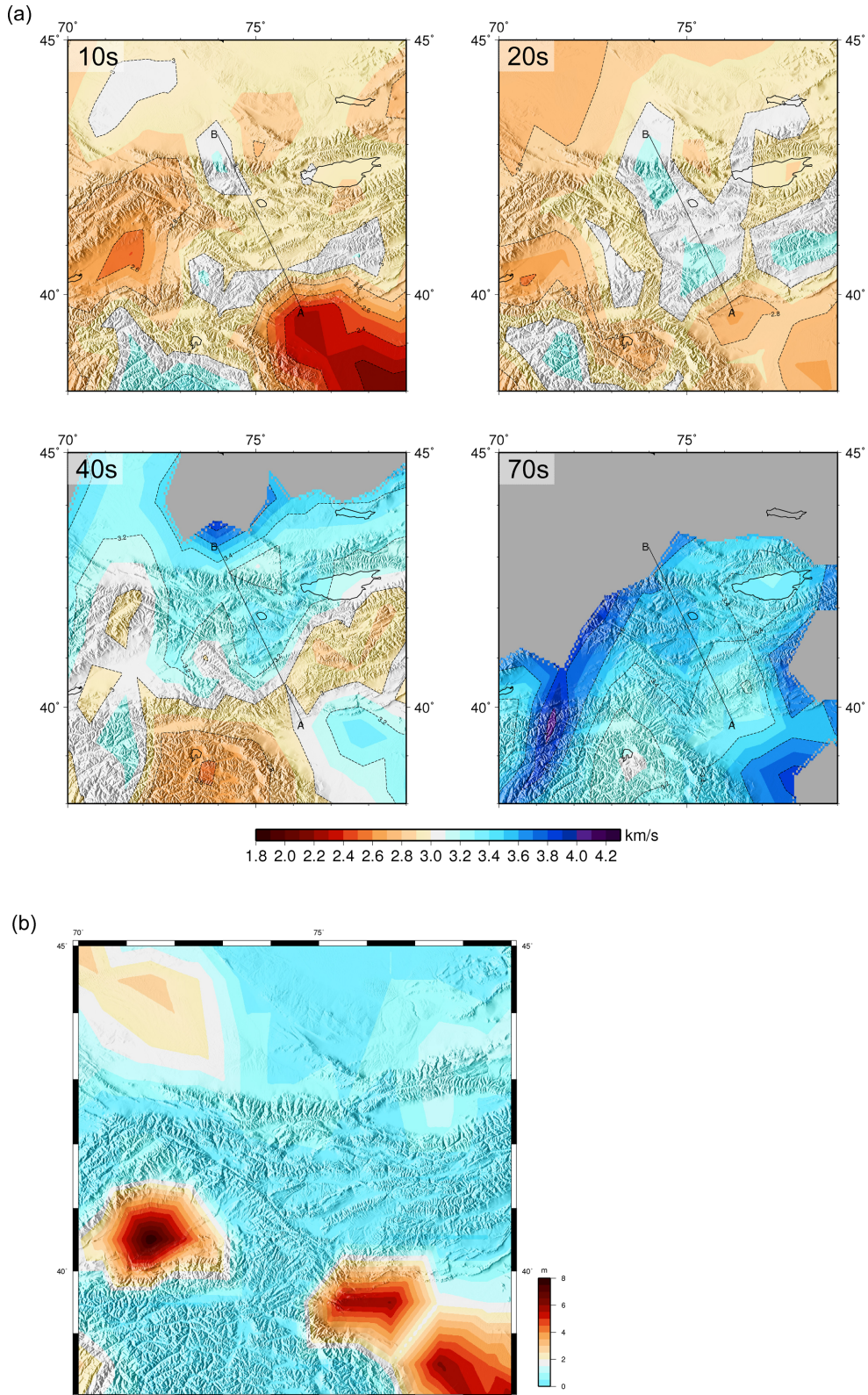
Figure 8. Fundamental mode Rayleigh wave group velocity maps for 10, 20, 40 and 70 s periods for the region around the MANAS array. The same scale is used in all of the maps. Grey areas are where the errors in the group velocities are greater than 0.3 \text{ km s}^{-1} . (b) Sediment thickness map showing the same area as (a) with data from the Global Map of Sediment Thickness, Laske & Masters (1997).
