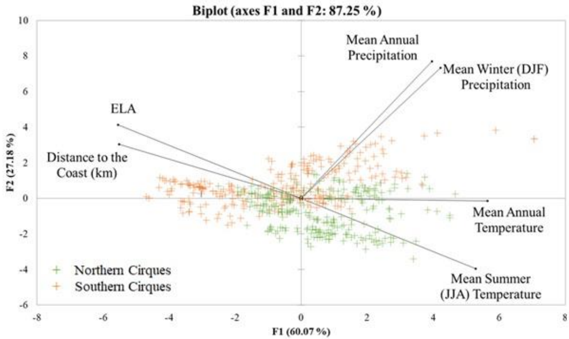
Figure 5: PCA of potential controls on Scandinavian cirque glacier ELAs. The orange crosses are the southern cirque glaciers and the green are the northern cirque glaciers. Northern cirque glaciers are distributed along the temperature component. Southern cirque glaciers are distributed along two components, precipitation and distance to coast, both reflecting the effect of continentality on southern cirque glacier distributions.
