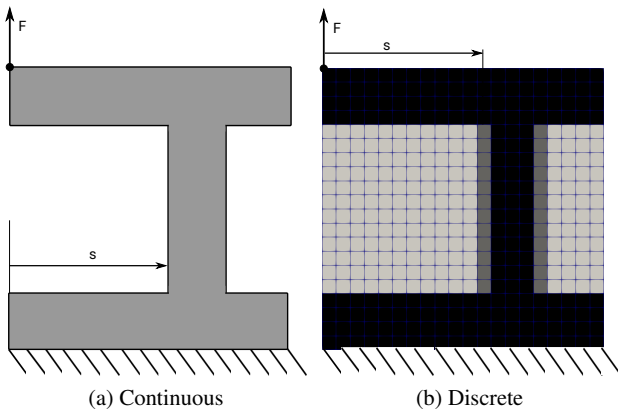
Fig. 4: H-shape test problem where the horizontal position of the vertical bar is given by the variable s . The force vector is applied on the upper left corner: (a) continuous setting; (b) discretized problem.
