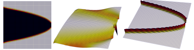
Fig. 9: For a smoothly mapped shape (left) the compliance sensitivity with respect to pseudo-density (22) is shown in the center. The element-wise summand of the sensitivity with respect to shape variables (24) is non-zero only where the pseudo-density has intermediate values (right). From Wein and Stingl (2018).
