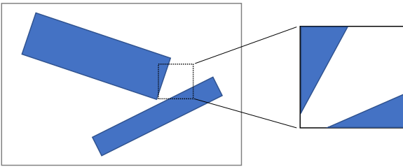
Fig. 13: Potential non-physical coupling in XFEM.
