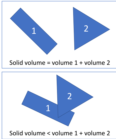
Fig. 21: Integral method for preventing component overlap.
