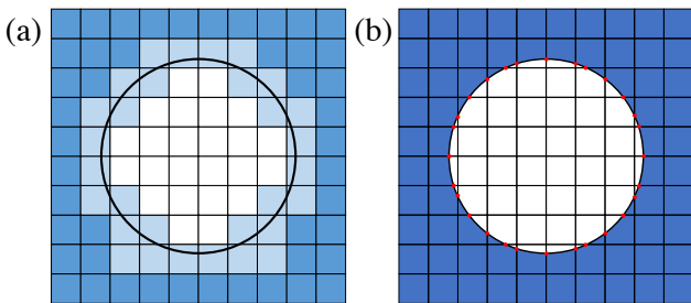
Fig. 1: Fixed-grid mapping methods: a) pseudo-density, and b) immersed-boundary based.
