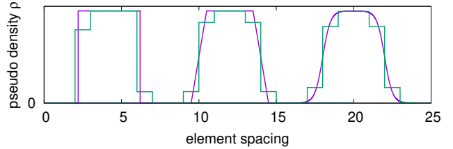
Fig. 6: 1D boundary modeling (in magenta): exact Heaviside function (left), piecewise linear (14) (center) and tanh smoothing (15) (right) and their element-constant pseudo-density values (in green).
