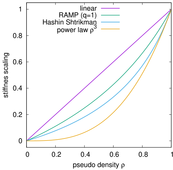
Fig. 3: Different material interpolation functions, see Sec. 3.1.1. Only the Hashin-Shtrikman bound and the common SIMP power law satisfy physical limits for an isotropic material with intermediate density
