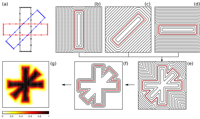
Fig. 16: Combination by conversion of explicit to implicit representation-then-mapping: (a) rectangular bars modeled with cubic B-splines, (b)–(d) signed distance of individual bars, (e) union of implicit signed-distance functions via maximum function, (f) smoothed Heaviside of implicit union, and (g) pseudo-density used for analysis.
