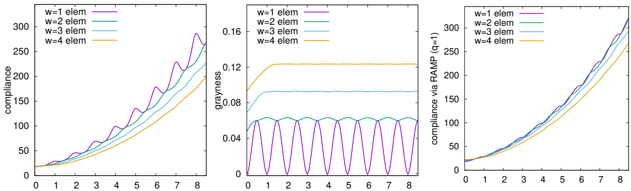
Fig. 12: We vary the polynomial smoothing (center in Fig. 10) by increasing the transition zone w = 2h from one to four elements, each time with midpoint integration. In the right figure RAMP interpolation (12) is applied. On the x -axis, the positional variable s is varied in element units.
