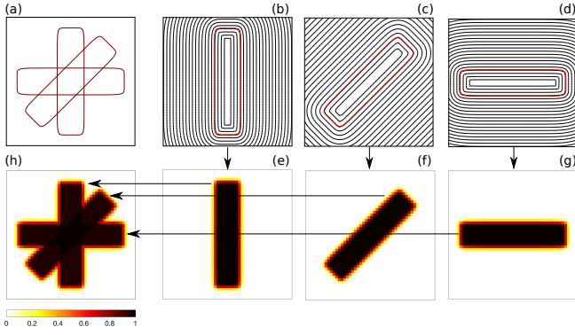
Fig. 17: Map-then-combine by union of offset surfaces: (a) bars modeled with offset surfaces (design variables are locations of endpoints of bars medial axes), (b)–(d) signed-distance field for each bar, computed directly from design parameters, (e)–(g) corresponding mapped pseudo-density for each bar, and (h) union of mapped densities using a smooth approximation of the maximum.
