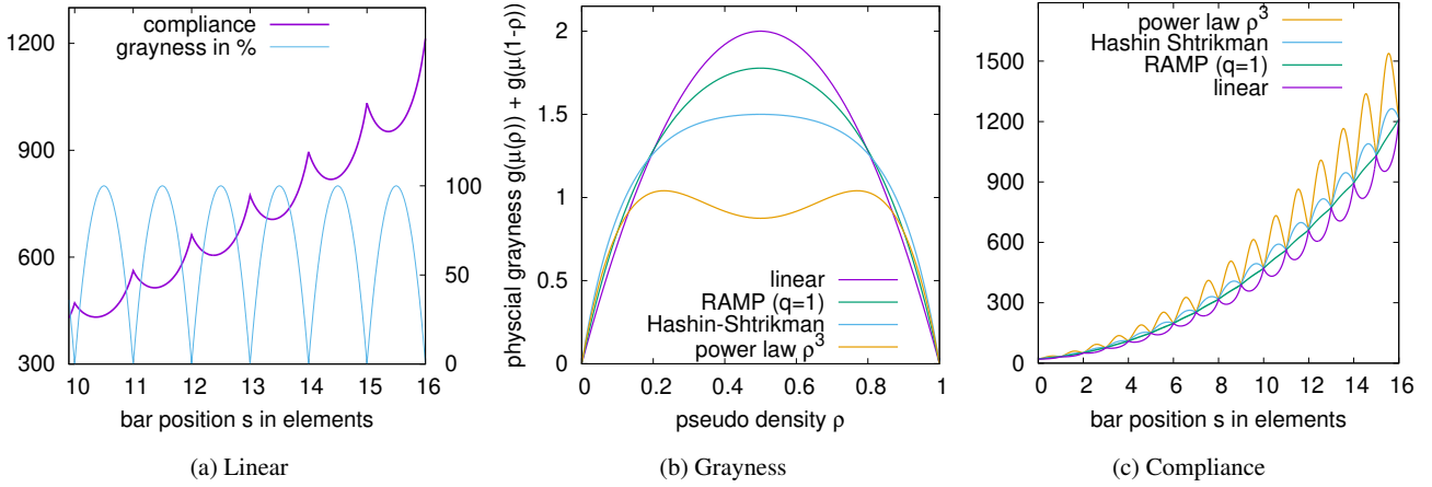
Fig. 5: (a) Compliance and grayness for the benchmark from Fig. 4 with linear material interpolation (where stiffness is scaled by the volume fraction covered by the bar); (b) sum of grayness values of the physical density g(\mu(\rho)) (13) for left and right edges of the vertical bar, corresponding to moving s by one element in Fig. 4 for different interpolation functions; and (c) their corresponding structural compliance values. See Sec. 3.1.1 for a detailed discussion.
