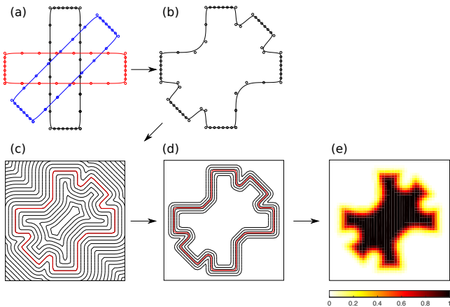
Fig. 15: Combination by union of explicit functions-then-mapping: (a) rectangular bars modeled with cubic B-splines, (b) union by deleting B-spline control points in the overlapping region, (c) signed-distance function of combined B-spline, (d) smoothed Heaviside of signed-distance function, and (e) pseudo-density used for analysis.
