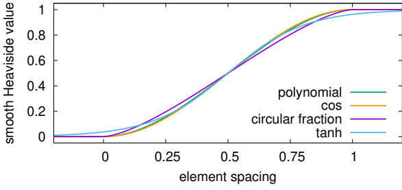
Fig. 8: Smooth boundary modelling by polynomial (18) (almost identical to cos (19)) and volume fraction with circular sampling window (20) with transition zone 2h equals one element width. The tanh-based function (15) is plotted with \beta = 6.5 . All functions are plotted assuming a signed-distance function.
