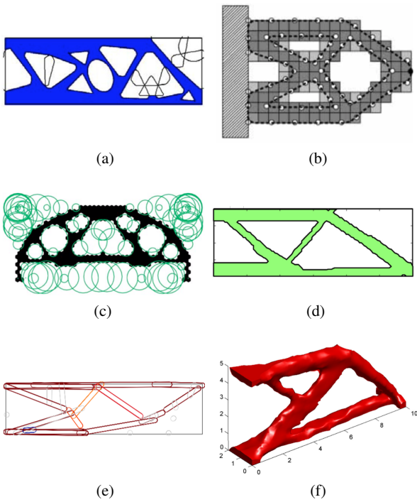
Fig. 24: Examples of different feature-mapping methods for topology optimization: a) feature-based method (Mei et al, 2008), b) smooth boundary method (Lee and Kwak, 2008), c) circular shaped masks method (Saxena, 2011), d) MMC method (Guo et al, 2014), e) geometry projection method (Norato et al, 2015) and f) MMV method (Zhang et al, 2017b).
