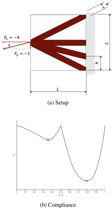
Fig. 19: Effect of combination on local minima. The crosses mark the locations of the local minima.
