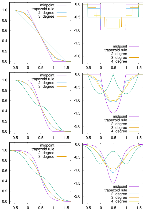
Fig. 11: For the first element [0 : 1] we perform numerical integration (9) by closed Newton–Cotes in the left column (the y -axis shows the integrated pseudo density \rho ) and numerically evaluate the shape sensitivity in the right columns (the y -axis shows \frac{\partial \rho}{\partial s} ). The x -axis gives the positional variable s . The boundary modeling functions are linear (first row), polynomial (second row) and tanh (last row).
