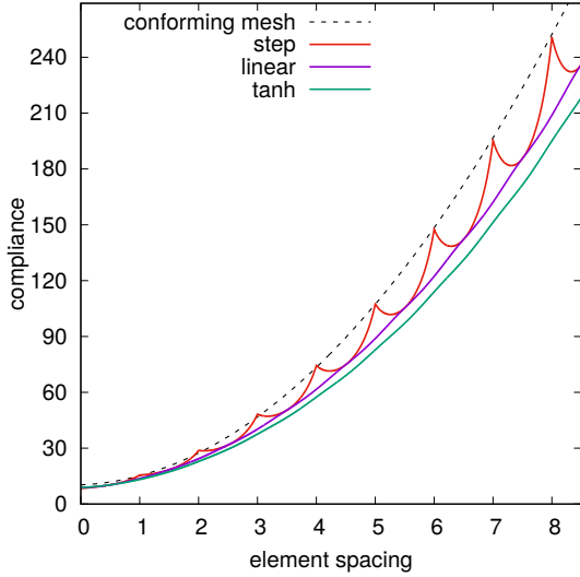
Fig. 7: Compliance values for the boundary modeling functions in Fig. 6 applied to the test problem in Fig. 4. Due to the linear density-to-stiffness interpolation the compliance is underestimated, see Fig. 5(c). The compliance for a conforming mesh is plotted for reference.
