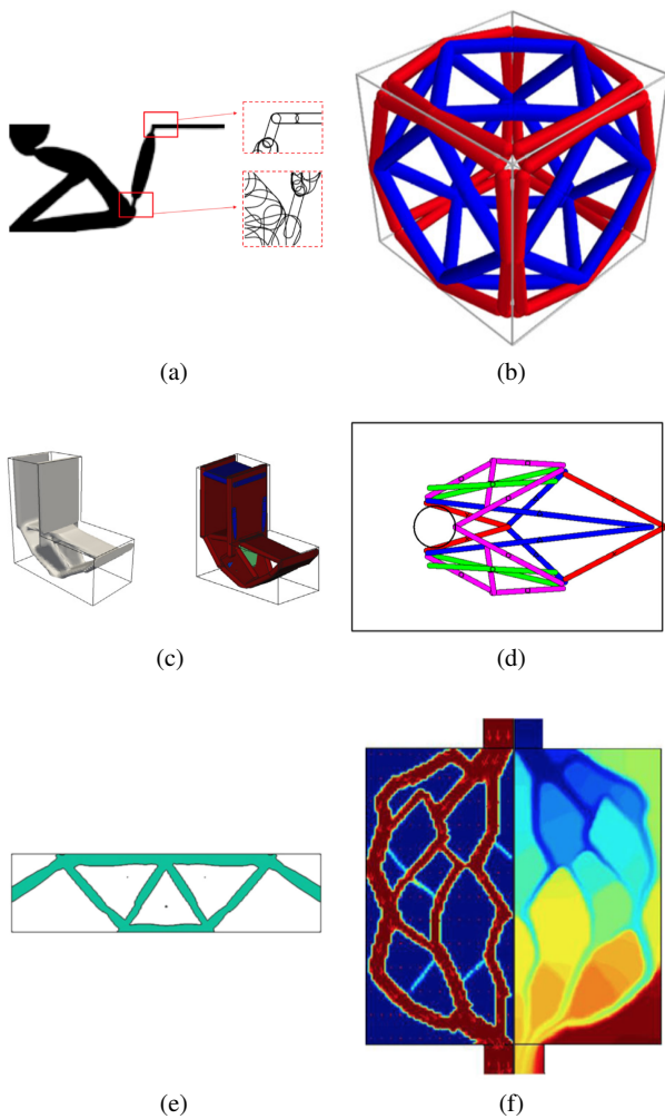
Fig. 25: Examples of different feature-mapping applications in topology optimization: a) compliant mechanism design (Hoang and Jang, 2017), b) material design (Watts and Tortorelli, 2017), c) stress constraints (Zhang et al, 2017a), d) multi-material structures (Kazemi et al, 2018), e) geometric nonlinearities (Zhu et al, 2018) and f) thermal-fluid problems (Yu et al, 2019).
