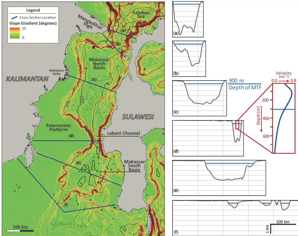
Fig. 3. Slope map extracted from the regional bathymetry RTM30_PLUS Global Bathymetry Data (Becker et al. 2009). Bathymetry contours at 250 m spacing. (a–f) Depth profiles across the Strait showing the main basin and channel features. Depth of Makassar Throughflow (MTF) indicated in blue. Velocity–depth profile shows average velocity profile for years 2004–09 (Susanto et al. 2012).
