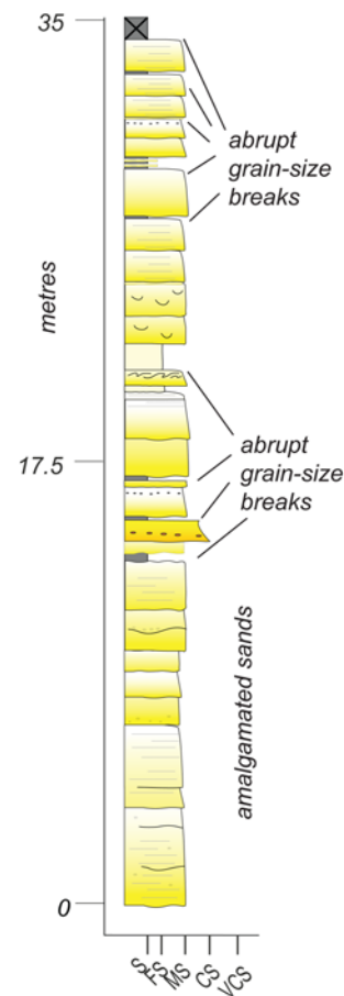
Fig. 12. Representative log of stacked bed-set in the Numidian at east of Colobraro village, Valsinni (UTM coordinates 621273.00 m E, 4449771.00 m N). Key as in Figure 8.
