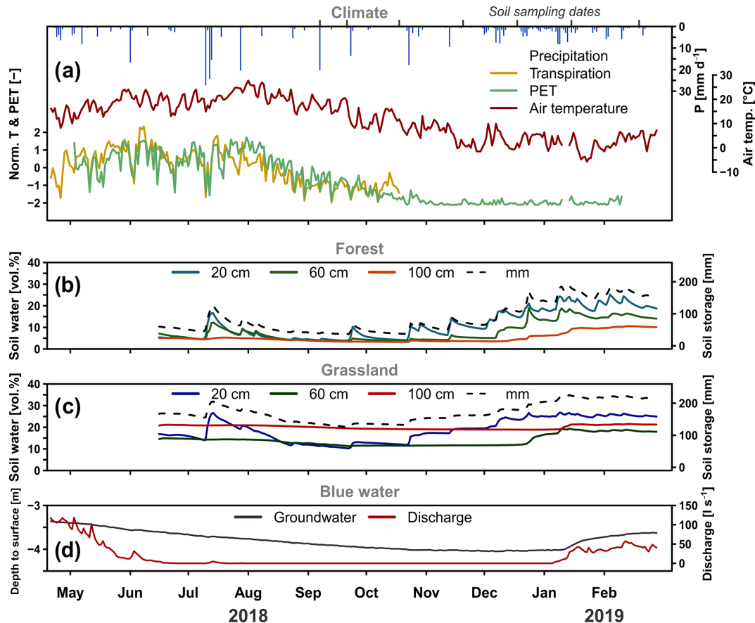
Figure 2. Daily precipitation, normalised transpiration (from sap-flow sensors), normalised PET (FAO Penman–Monteith) (a), volumetric soil moisture ( n = 6 per three depths of the forested plot) (b), and grassland site (c) with the total soil water in millimetres (dashed line) and groundwater elevation relative to surface and discharge at the Demnitz Mill (d) for the 2018 growing season and 2019 re-wetting.
