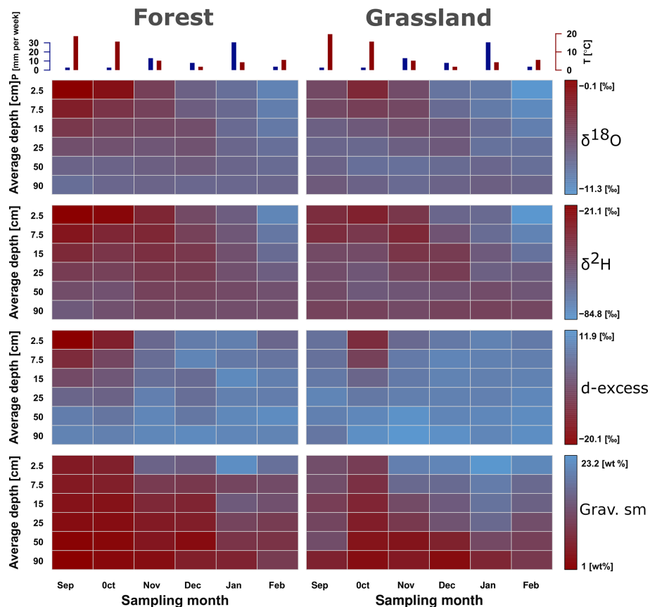
Figure 5. Heat map of soil depth profiles for mean \delta^2\text{H} , \delta^{18}\text{O} , d-excess and gravimetric (grav.) soil moisture of three replicates at both land use classes (forest and grassland) of six monthly sampling dates. Blue to red colours indicate more to less depleted \delta^2\text{H} and \delta^{18}\text{O} values, declining d-excess, and grav. soil moisture values. On top, antecedent conditions of mean daily air temperature and the sum of precipitation 7 d prior to sampling are displayed in the bar chart.
