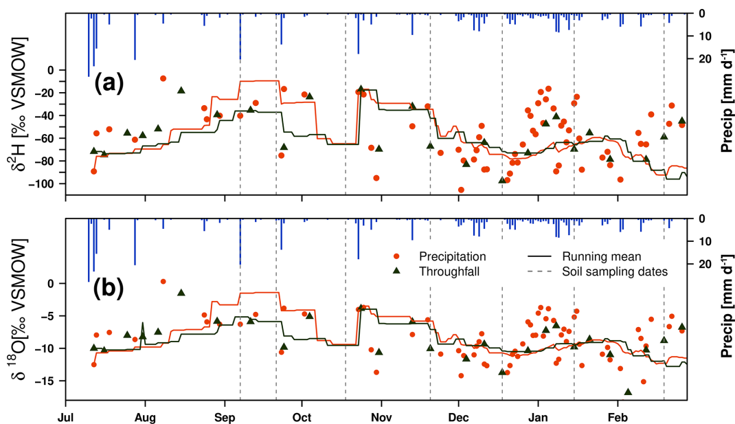
Figure 4. Time series of daily precipitation amount and isotopic signature of weekly throughfall at forest A and daily precipitation and their 30 d running (volume-weighted) mean for \delta^2\text{H} (a) and \delta^{18}\text{O} (b), with dotted lines indicating dates of bulk soil water sampling (dashed line).
