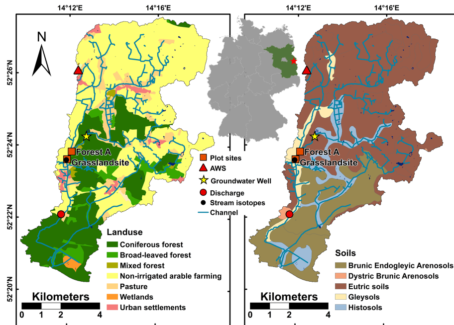
Figure 1. Study site location, sampling site locations, soils, and land use (source: © GeoBasis-DE/BKG 2018; data changed) of the DMC.
