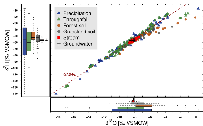
Figure 3. Dual-isotope plot of DMC precipitation, throughfall, forest and grassland soil bulk water samples, as well as stream water and groundwater.
