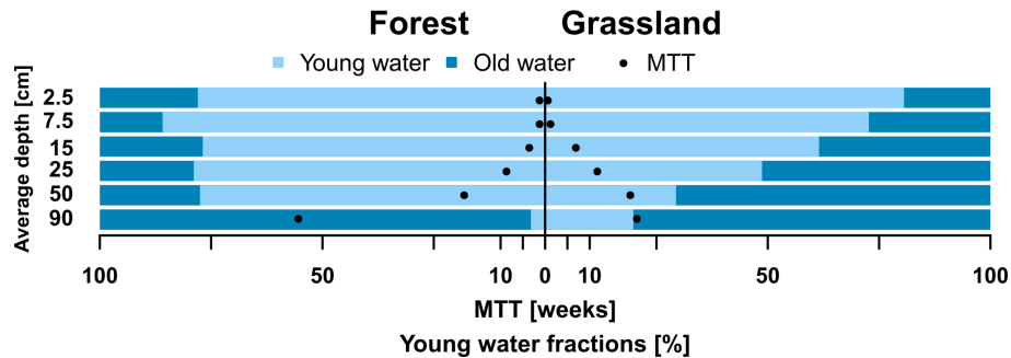
Figure 6. Young water fractions (bars) and MTT (dots) per soil depths at forested and grassland sites.
