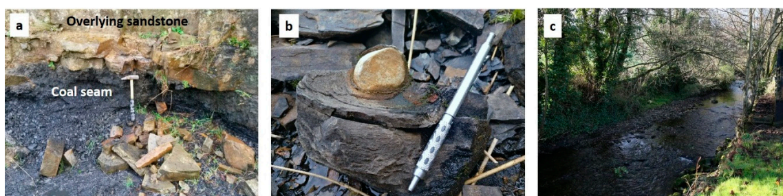
Figure 4. Sampling locations in the Castlecomer area of the Leinster Coalfield, County Kilkenny. (a) In situ coal seam and loose spoil at the abandoned Bilboa Quarry, Castlecomer. (b) Sideritic nodule hosted within coal (Bilboa Quarry). (c) The River Dinin, which flows through the former coal mining Castlecomer area, which hosts mineralised coal and siderite samples.
