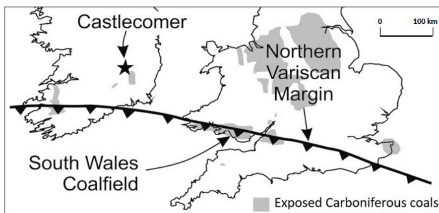
Figure 2. Setting of the Leinster Coalfield and South Wales Coalfield as basins north of the Variscan belt, modified from [33]. Gold associated with selenides, pyrite and siderite nodules have been previously recognised in the South Wales Coalfield [12,13,34], while Castlecomer coals of the Leinster Coalfield (sample area indicated by black star) are both pyritic and contain abundant siderite nodules [35].
