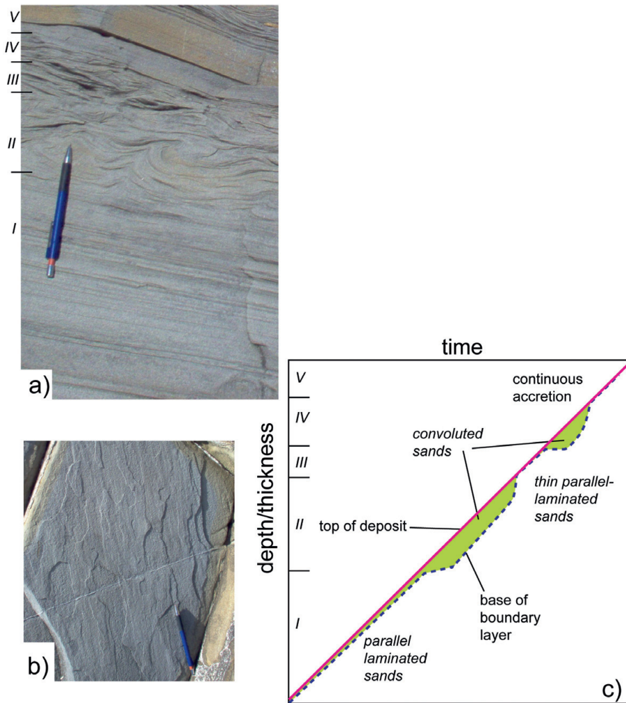
Fig. 4. Kinematic relationships between a turbidity current and its aggrading substrate recorded in Bouma Tb–Tc intervals within sandstones of the Oligo-Miocene Macigno Costieri Formation (Cornamusini et al. 2002; Eggenhuisen et al. 2010a) at Baratti (Tuscany coast, Italy). (a) View of parallel laminated turbidite sandstone (Tb interval) passing up into convolute lamination (Tc). (b) Plan view of planar lamination (Tb interval) with characteristic grain alignment fabric parallel to inferred direction of palaeoflow. (c) Unscaled co-plot of deposition and kinematic boundary layer evolution against relative time.
