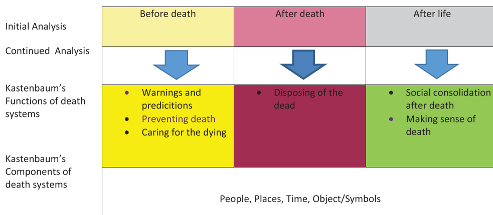
Figure 1. Analytic framework.
