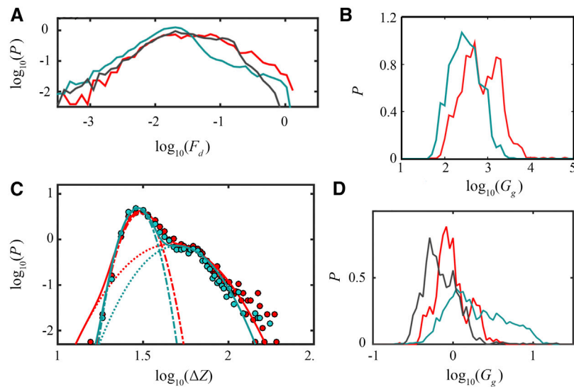
FIGURE 2 | (A) Probability distributions of the logarithm of the local force drops F_d (nN) estimated from local disruption events collected from sets of myoblasts (red), myotubes (blue) and ATP depleted myoblasts (black); (B) Probability distributions of the logarithm of shear relaxation modulus G_g (kPa) estimated by a parabolic fit of the Force-Indentation Curves (Sneddon model [71]), from healthy (blue) and leukemic (red) immature CD34_+ hematopoietic cells; (C) Distribution of the indentation lengths of the rupture events detected from healthy (blue) and leukemic (red) immature CD34_+ hematopoietic cells; (D) Probability distributions of the logarithm of shear relaxation modulus G_g (kPa) on the same sets of cells as in (A) . Note that plots (A) and (C) are in log-log scale and plots (B) and (D) are in semi-log scale. All the logarithms are here in base 10. Panels (A) and (D) are adapted from [67] (B) from [2] and (C) from [2].
