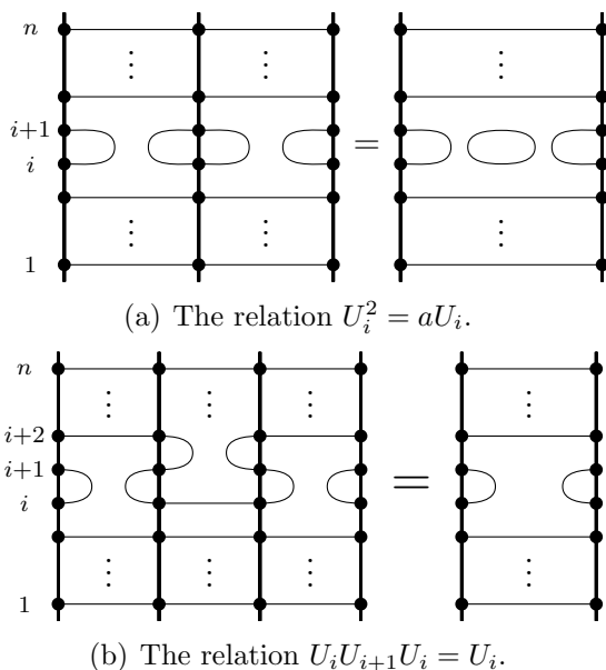
FIGURE 1. Diagrammatic relations in \mathrm{TL}_n(a) .
