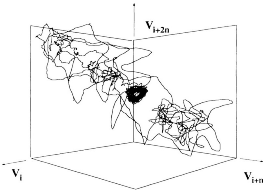
FIG. 15. Trajectory of a chaotic transient ending in a periodic attractor. From Ref. 184
