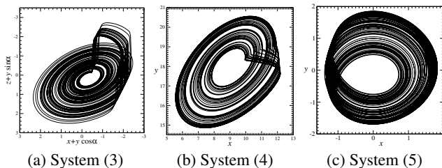
FIG. 4. The chaotic attractor obtained after some simplifications of the original equations. Parameter values for system (4): a = 0.2 , b = 0.2 , c = 5.7 . For system (5) b = 0.275 and c = 0.2 and initial conditions are x_0 = 1 , y_0 = -1.4 and z_0 = -0.4 .
