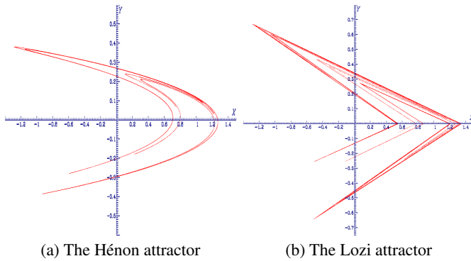
FIG. 6. Some simple mappings
