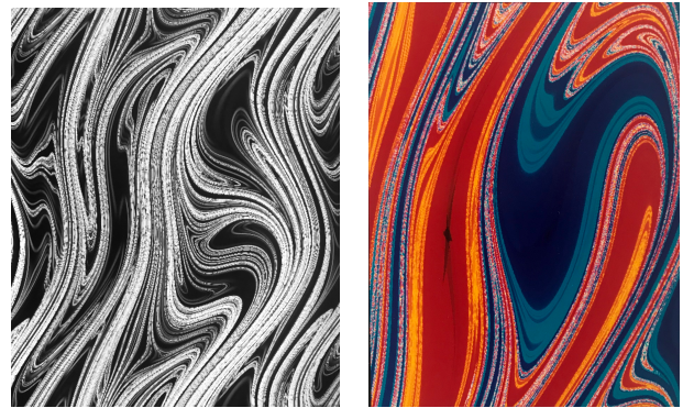
FIG. 12. Fractal basin boundary and the basins of attraction of the forced damped pendulum equation (14). Parameter values: \nu = 0.1 , \omega = 1 , and f = 2 . From Ref. 141
