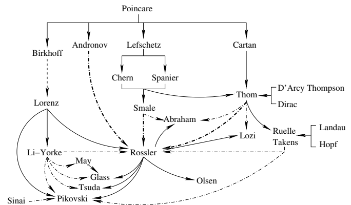
FIG. 16. Some influences between contributors based on some testimonies from the previous sections. The graph is organized for a sake of simplicity. The arrows (— · — ·) correspond to the introduction of numerical simulations. The three bold arrows to Rössler are influences — through direct meetings — before 1975.
