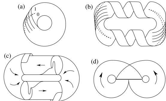
FIG. 14. Branched manifolds describing (a) Rössler, (b) periodically driven Duffing, (c) van der Pol attractors, and (d) Lorenz attractors and for particular parameter values. Redrawn from Ref. 181.
