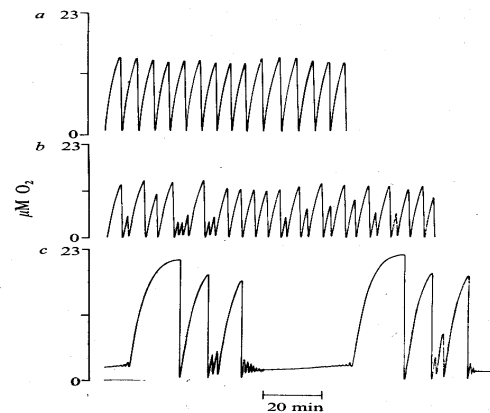
FIG. 9. Simple periodic (a), chaotic (b) and bursting (c) oscillations of O_2 in the peroxidase-oxidase reaction. Reproduced with permission from Ref.123.
