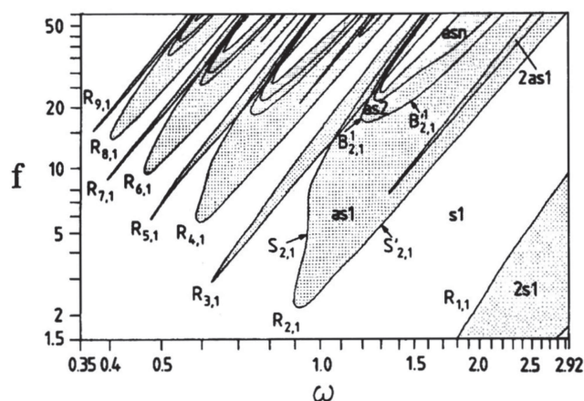
FIG. 13. Parameter space of the Duffing system (15). In the differently dotted domains, there are symmetrical period-1 limit cycle (s1), two coexisting symmetry-related period-1 limit cycle (as1), two pairs of asymmetry related period-1 limit cycles (2as1), a pair of period-2 symmetry-related limit cycles (as2), and pairs of period- n symmetry-related limit cycles (asn) with n = 4, 8, 16, \dots . Reproduced with permission from U. Parlitz and W. Lauterborn, Phys. Lett. A 107 , 351–355 (1985). Copyright 1985 Elsevier.
