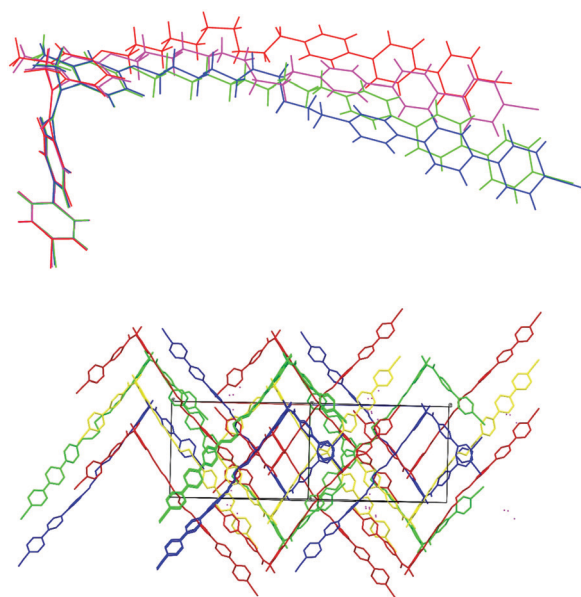
Fig. 13 Top: Overlay plot of the four molecules in the asymmetric unit of 5b . Below: The unit-cell packing for 5b viewed approximately down [101] with the four asymmetric molecules and their symmetry-generated clones shown in red, blue, green and yellow (H atoms omitted for clarity).
