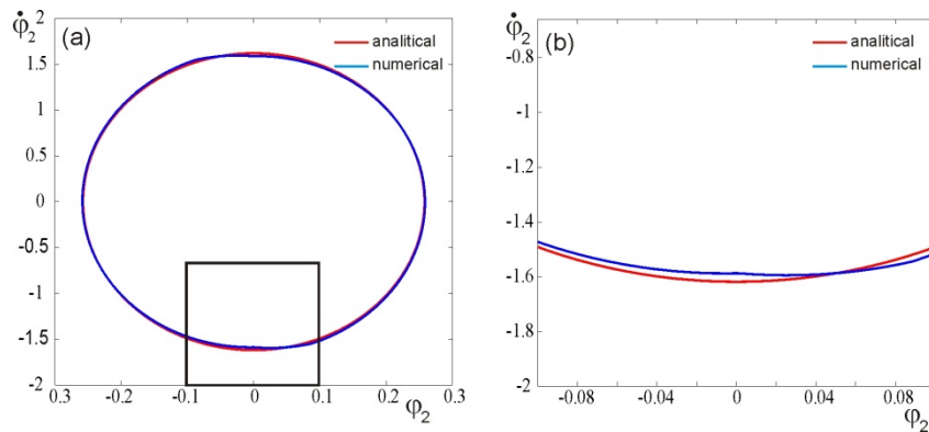
Figure 13. Comparison of the numerical solution of discontinuous eq. (13) with the harmonic assumption (14).
