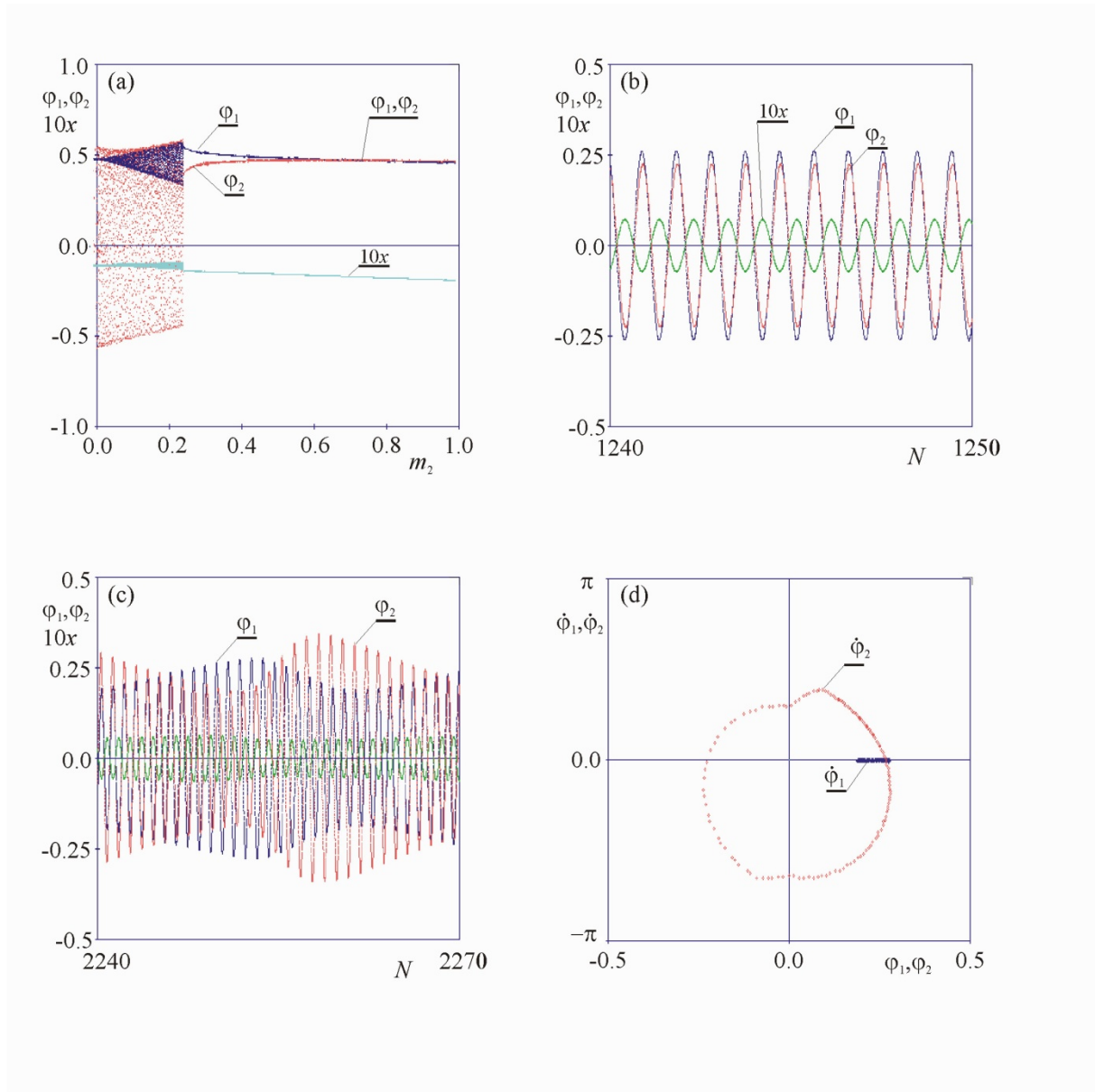
Figure 28: Evolution from complete synchronization to quasiperiodic oscillations; (a) bifurcation diagram for increasing values of m_2 , (b) time series of almost complete synchronization for m_1=1.0 [kg] and m_2=0.3 [kg], (c) time series of quasiperiodic oscillations for m_1=1.0 [kg] and m_2=0.2 [kg], (d) Poincare map showing quasiperiodic oscillations for m_1=1.0 [kg] and m_2=0.2 [kg].
