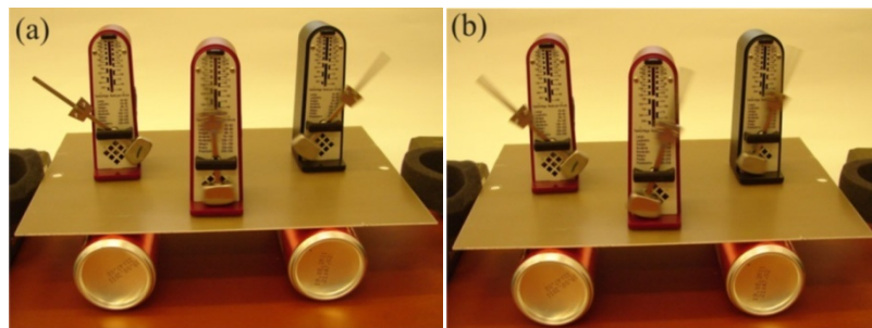
Figure 46: Three metronomes located on the plate which can roll on the base: (a) symmetrical synchronization with phase shift \beta_{II}=\beta_{III}=120^\circ , (b) antiphase synchronization of the left metronome with the cluster of the center and right metronomes (the mass of the left pendulum is equal to the sum of the masses of the center and right pendula).
