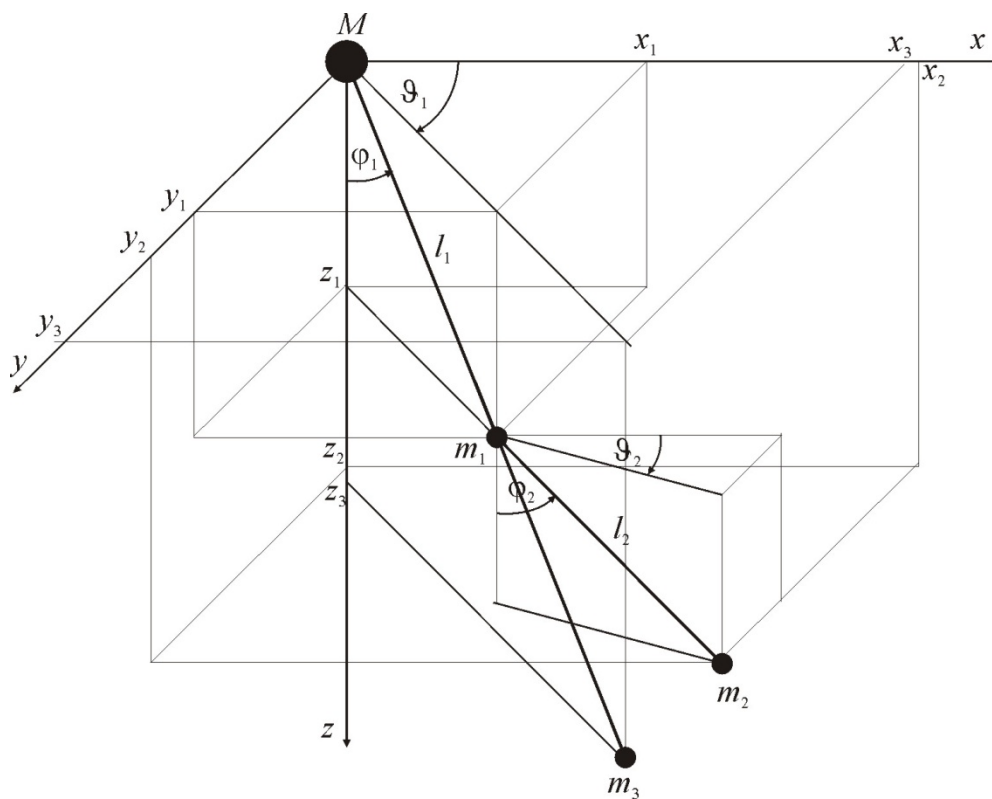
Figure 17: Coordinates describing the oscillations of the double pendulum.
