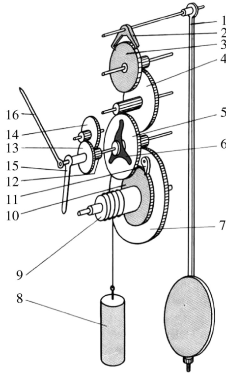
Figure 6: The sketch of the basic components of a pendulum clock with anchor escapement. (after [70]: (1) pendulum; (2) anchor escapement arms; (3) escape wheel; (4–7) gear train; (8) gravity-driven weight; (9-11) energy supply mechanism, (12-14) transition mechanism, (15,16) clock's hands.
