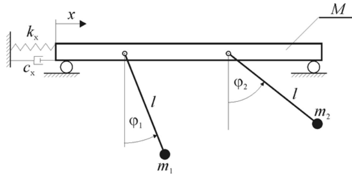
Figure 18: The model of the system – two pendulum clocks are mounted to the beam which can move horizontally.
