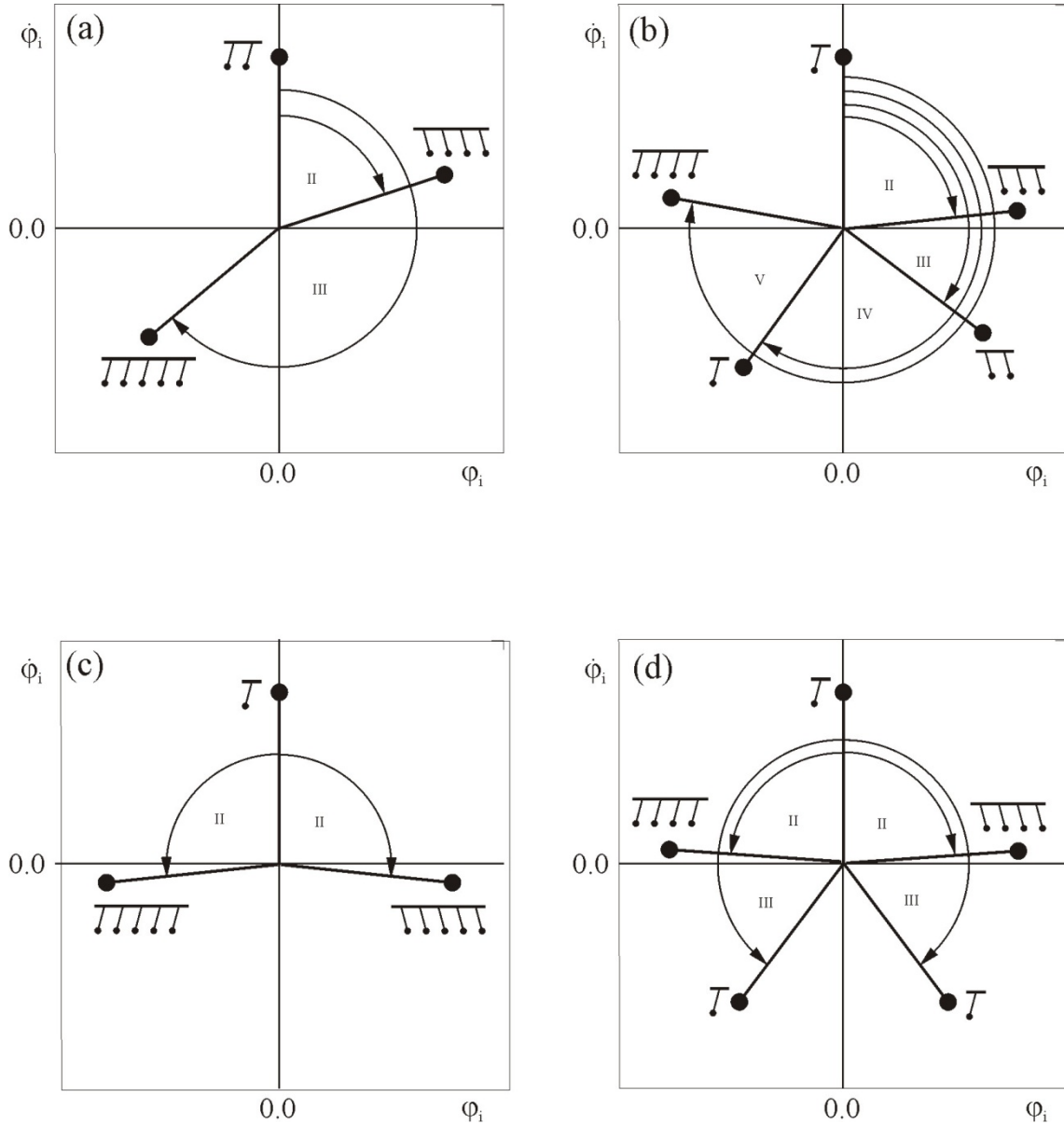
Figure 52: Cluster configurations for n=11 pendula; m=1 [kg], l=g/4\pi^2 [m], c_\phi=0.01 [Nsm], M=1 [kg], c_x=0.1 [Ns/m], k_x=1 [N/m], M_N=0.075 [Nm], \gamma_N=\pi/36 : (a) three cluster configuration; n_I=2 , n_{II}=4 , n_{III}=5 , (b) five cluster configuration; n_I=1 , n_{II}=3 , n_{III}=2 , n_{IV}=1 , n_V=4 , (c) symmetrical three cluster configuration; n_I=1 , n_{II}=5 , and n_{III}=5 , (d) symmetrical five cluster configuration; n_I=1 , n_{II}=4 , n_{III}=1 , n_{IV}=1 , and n_V=4 .
