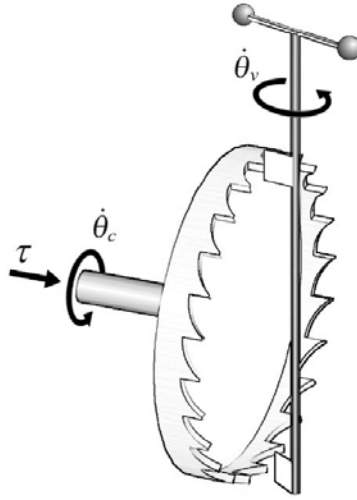
Figure 7: Verge-and-foliot escapement mechanism (after [94]).
