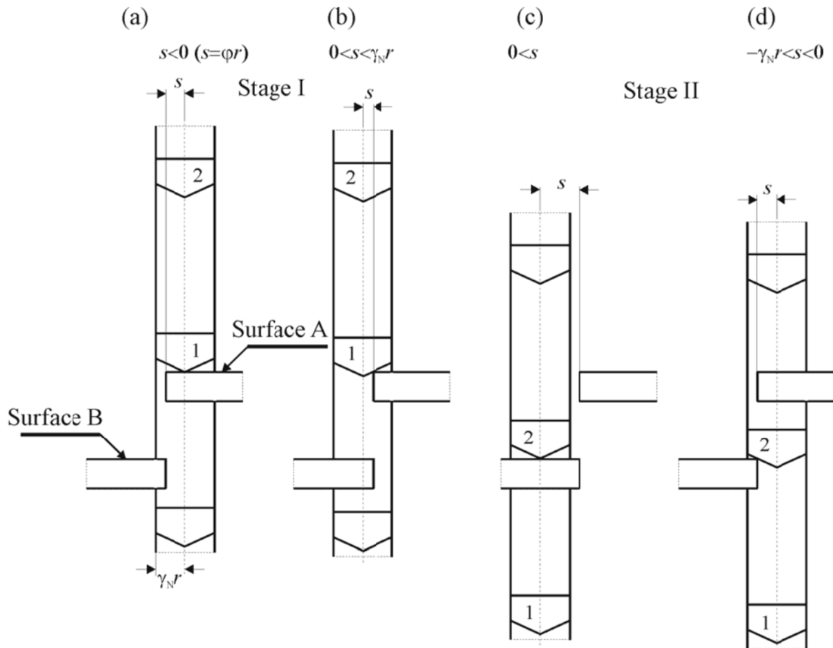
Figure 11. Acting of the escapement mechanism.
