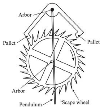
Figure 9: Deadbeat escapement mechanism.
