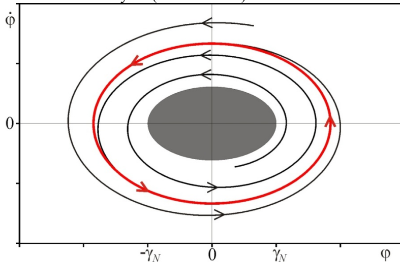
Figure 12. An autonomous model of the clock.
