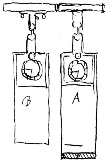
Figure 2: Details of the Huygens' experiment; it is clearly visible that the clocks used in the experiment have not been identical, D denotes the weight used to stabilize the clock case.
