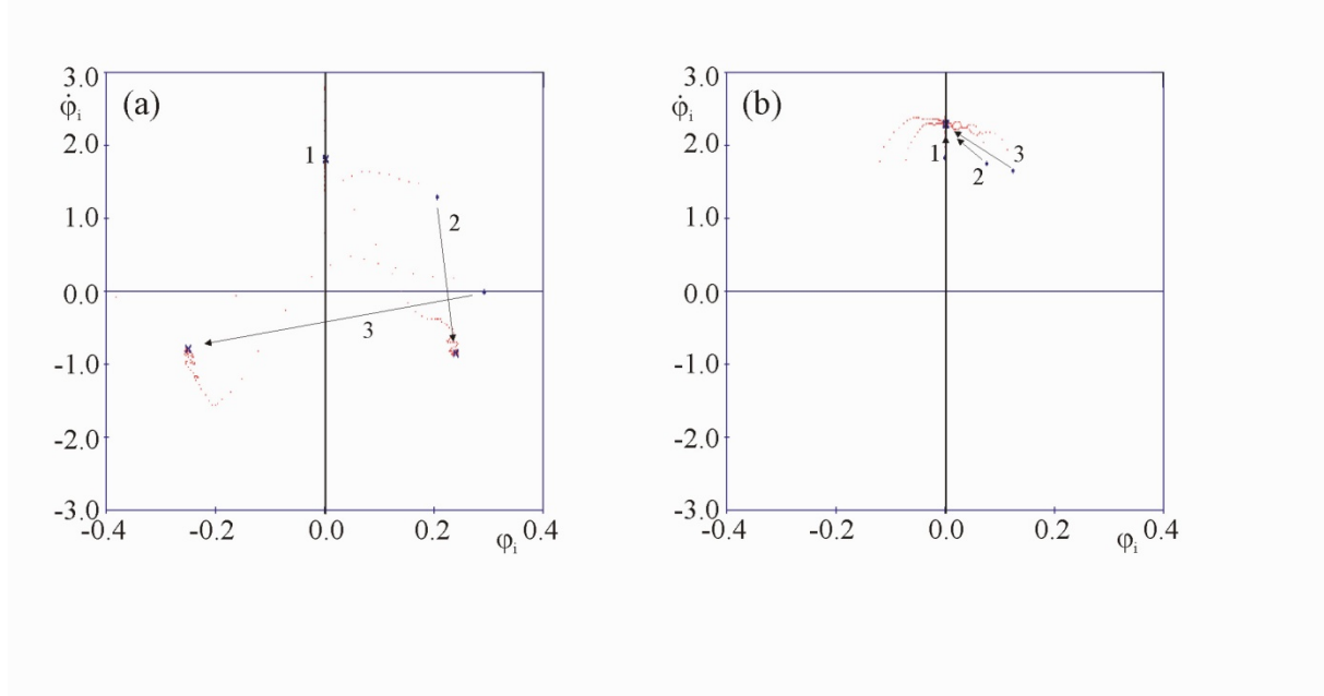
Figure 48: The synchronization configurations for three pendula; m=1 [kg], l=g/4\pi^2 [m], c_\phi=0.01 [Nsm], M=1 [kg], c_x=0.1M [Ns/m], k_x=M [N/m], M_N=0.075 [Nm], \gamma_N=\pi/36 : (a) (SS) with phase difference \Delta\beta=2\pi/3 ; \beta_{10}=0 , \beta_{20}=2\pi/8 , \beta_{30}=2\pi/4 (b) (CS): \beta_{10}=0 , \beta_{20}=2\pi/24 , \beta_{30}=2\pi/18 .
