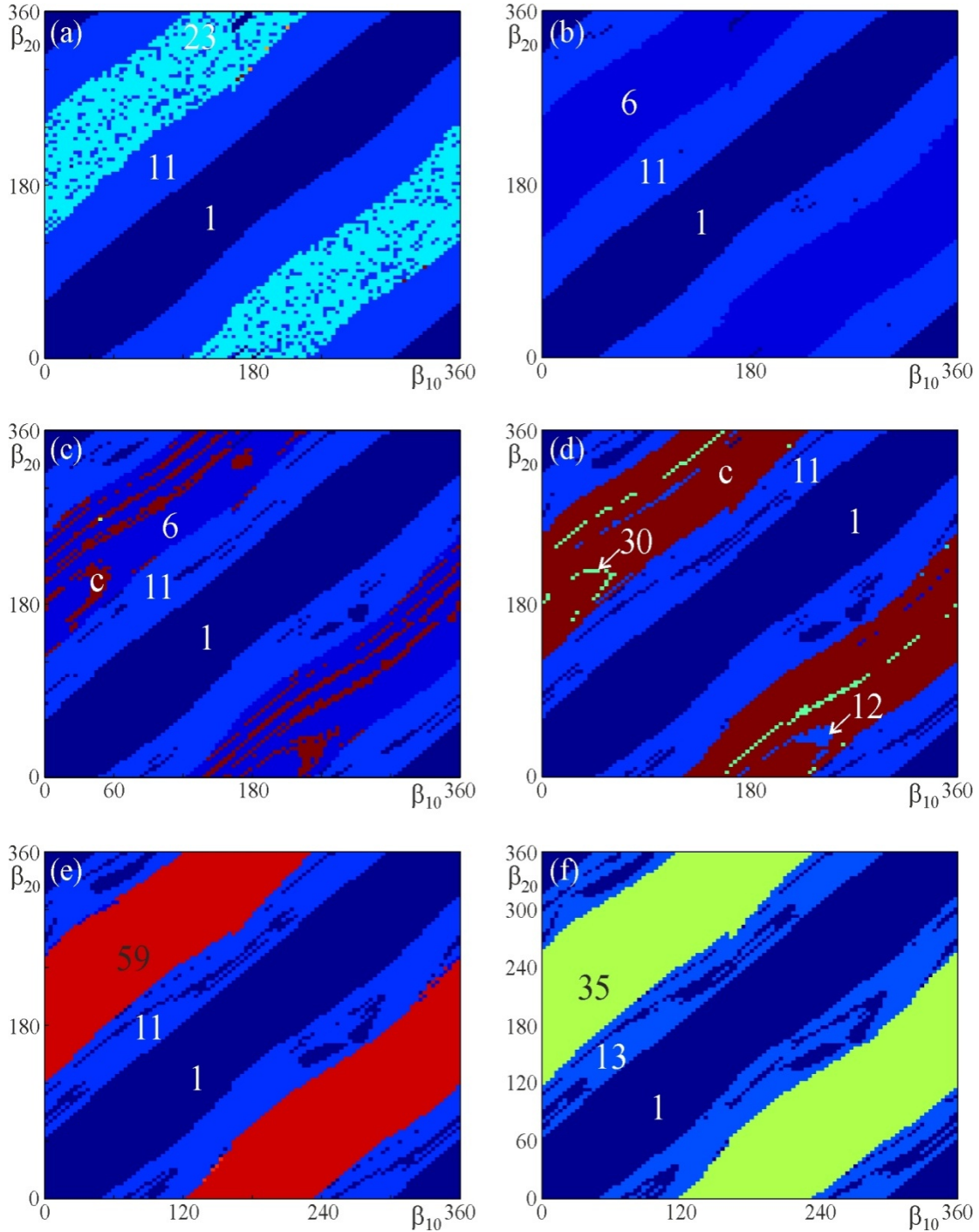
Figure 40: Basins of attraction of different types of synchronous states for m_2=3.105 ; the numbers indicate the period of the (LPS), (C) shows chaotic behavior. Parameters: \gamma_N=4.5^\circ (a); \gamma_N=4.8^\circ (b); \gamma_N=5.0^\circ (c); \gamma_N=5.05^\circ (d); \gamma_N=5.1^\circ (e); \gamma_N=5.2^\circ (f). other parameters are the same as in Figure 39, initial values: x(0)=0.0 , \dot{x}(0)=0.0 , \varphi_{i0} = \Phi \sin \beta_{i0} , \dot{\varphi}_{i0} = \alpha \Phi \cos \beta_{i0} .
