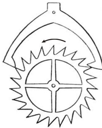
Figure 8: Anchor escapement.
