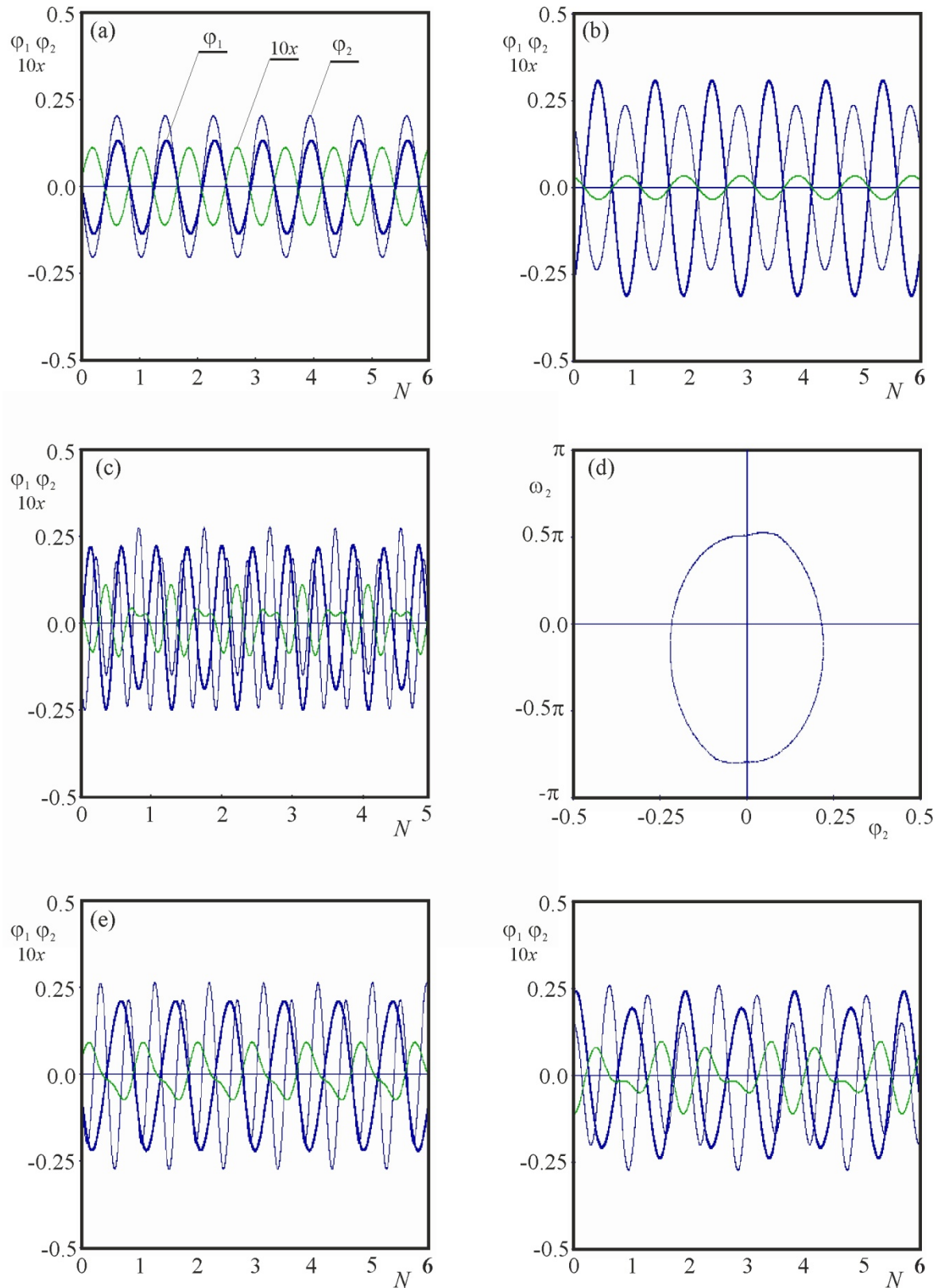
Figure 37: Different types of synchronization of the clock pendula; (a) in-phase synchronization 1/1 for \xi=0.95 ; (b) antiphase synchronization 1/1 for \xi=0.95 ; (c) time series of quasiperiodic oscillations for \xi=0.6871 , (d) Poincare map for \xi=0.6871 , (e) synchronization 1/2 for \xi=0.51 ; (f) synchronization 2/3 for \xi=0.6887 .
