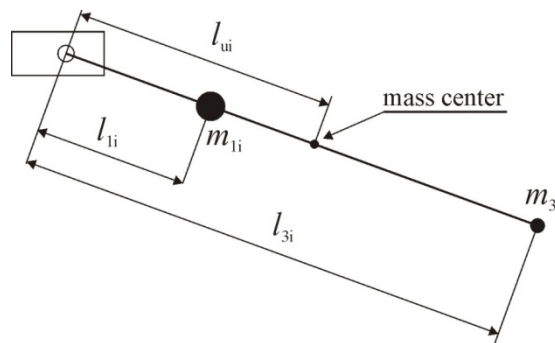
Figure 16: Geometry of the double-pendulum.
