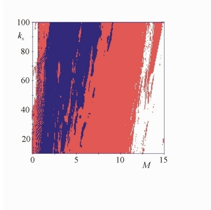
Figure 49: The steady states of eqs (96,97) for different values of parameters M and k_x ; m=1 [kg], l=g/4\pi^2 [m], c_\varphi=0.01 [Nsm], c_x=0.1M [Ns/m], M_N=0.075 [Nm], \gamma_N=\pi/36 , \beta_{10}=0 , \beta_{20}=\pi/8 , \beta_{30}=\pi/9 , x_0 = \dot{x}_0 = 0 . (SS), (CS) and (DSB) are indicated respectively in navy blue, white and red colors.
