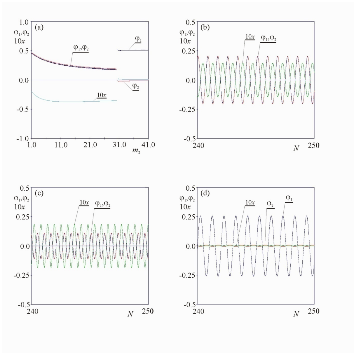
Figure 26: Evolution from complete to almost antiphase synchronization; (a) bifurcation diagram for increasing values of m_2 , (b) time series of almost complete synchronization m_1=1.0 [kg] and m_2=3.0 [kg]; (c) time series of almost complete synchronization m_1=1.0 [kg] and m_2=20.0 [kg]; (d) time series of almost antiphase synchronization for m_1=1.0 [kg] and m_2=35.0 [kg]— the escapement mechanism of pendulum 2 is switched off.
