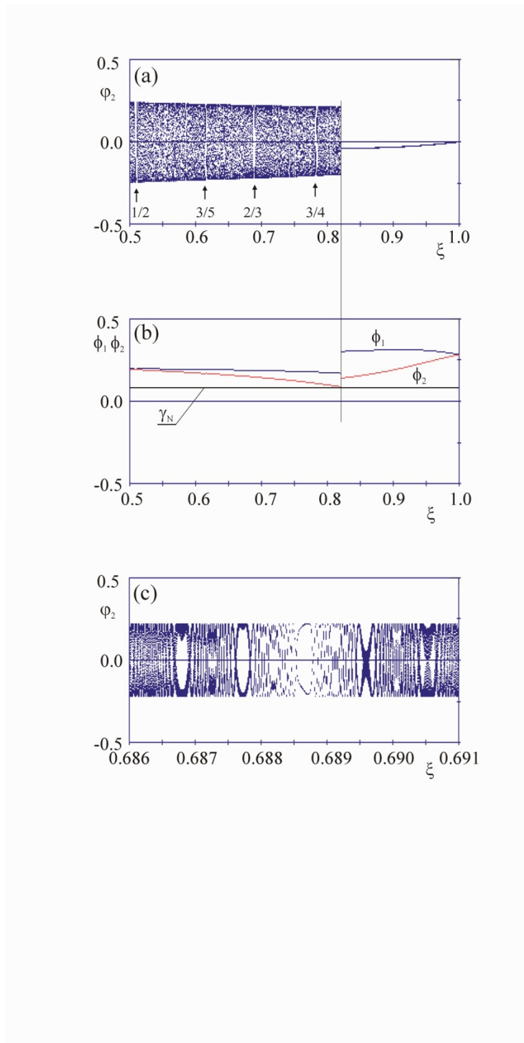
Figure 36: (a) Bifurcation diagram of system (27,28) for increasing \xi , (bifurcation diagram: starts with \xi=0.5 and \varphi_{10}=\varphi_{20}=0.26 and ends with \xi=1.0 ) (b) minima of amplitudes of pendula's oscillations; (c) enlargement of (a) in the neighborhood of synchronization 2/3 .
