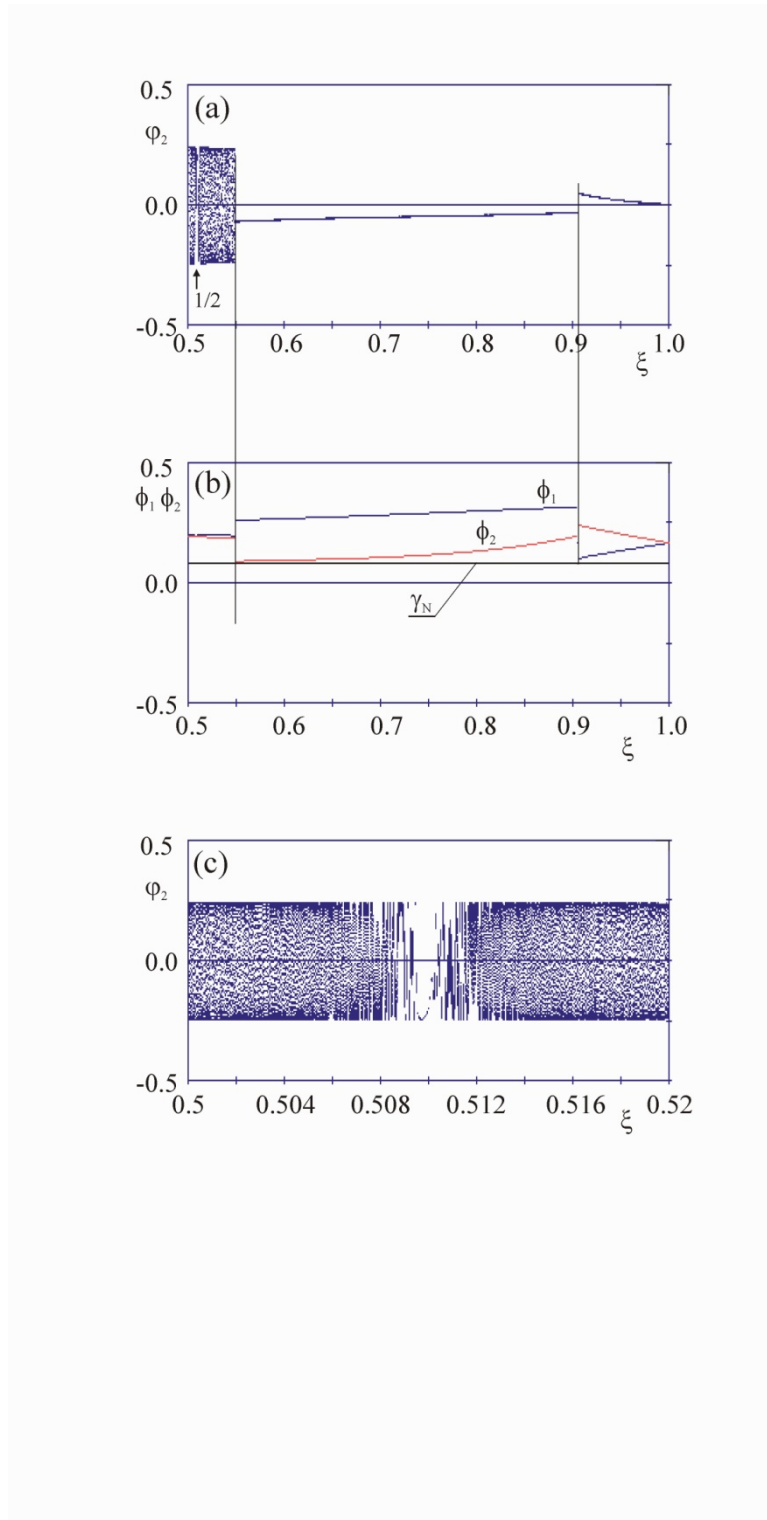
Figure 35: (a) Bifurcation diagram of system (27,28) for decreasing \xi ; (bifurcation diagram: starts with \xi=1.0 and \varphi_{10}=\varphi_{20}=0.26 and ends with \xi=0.5 ), (b) minima of amplitudes of pendula's oscillations, (c) enlargement of (a) in the neighborhood of synchronization 1/2 .
