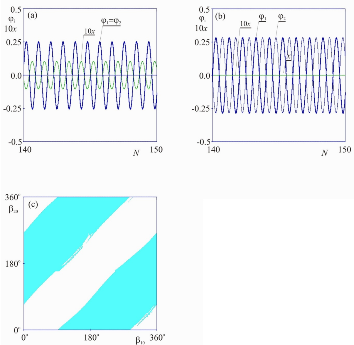
Figure 21: (Color online) Synchronization of two identical pendulum clocks 7 : m_1=m_2=1.0 [kg], l=g/4\pi^2=0.2485 [m], M=10.0 [kg], c_{\phi_1}=c_{\phi_2}=0.0083 [Nsm], c_x=1.53 [Ns/m], k_x=4.0 [N/m], \gamma_N=5.0^\circ , M_{N1}=M_{N2}=0.075 [Nm]; (a,b) time series of pendula \phi_1 , \phi_2 and beam x displacements, time on the horizontal axis is given in the following way t=NT , where N=1,2,3,\dots and T=1 [s], (a) complete synchronization ( \phi_1=\phi_2 ) pendula are in the antiphase to the oscillations of the beam M , (b) antiphase synchronization ( \phi_1=-\phi_2 ), beam M is at rest, (c) basins of attraction of complete synchronization (white color) and antiphase synchronization (gray/blue online color) in \beta_{10} - \beta_{20} plane, x(0)=0.0 , \dot{x}(0)=0.0 , \phi_{i0} = \Phi \sin \beta_{i0} , \dot{\phi}_{i0} = \alpha \Phi \cos \beta_{i0} .
