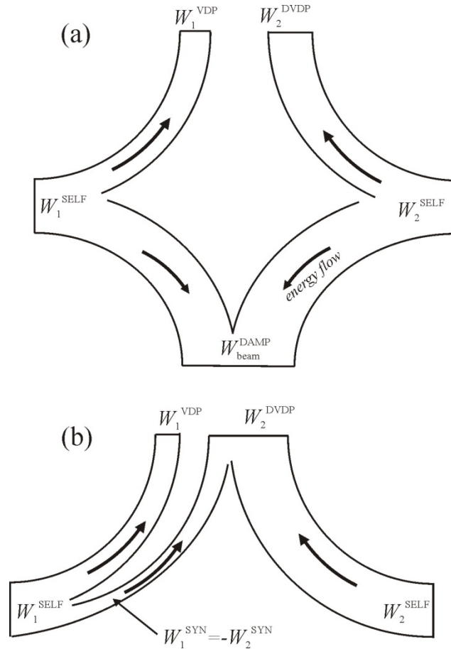
Figure 42. Energy balances of the system (1,2); (a) almost complete synchronization – both pendula drive the beam, (b) almost antiphase synchronization – pendulum 1 drives pendulum 2 via the beam.
