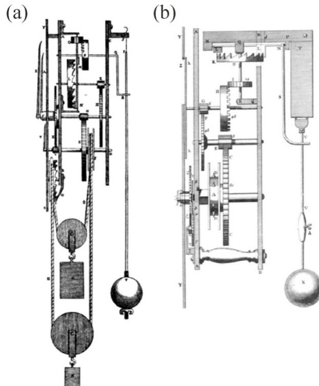
Figure 4: (a) The first pendulum clock, invented by Christiaan Huygens in 1656, (b) . The second verge pendulum clock built in 1673.
