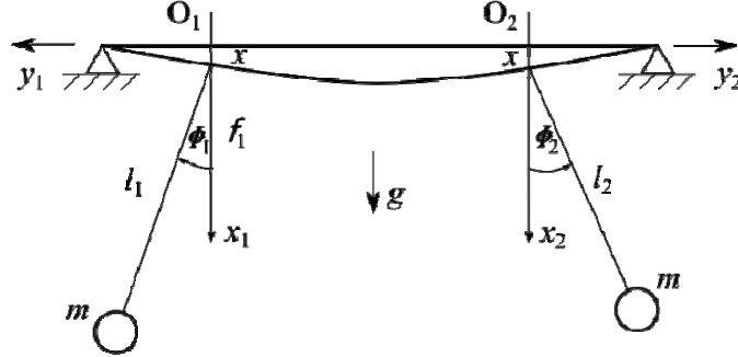
Figure 19: Two clocks suspended on the beam which can perform transversal oscillations (after [55]).
