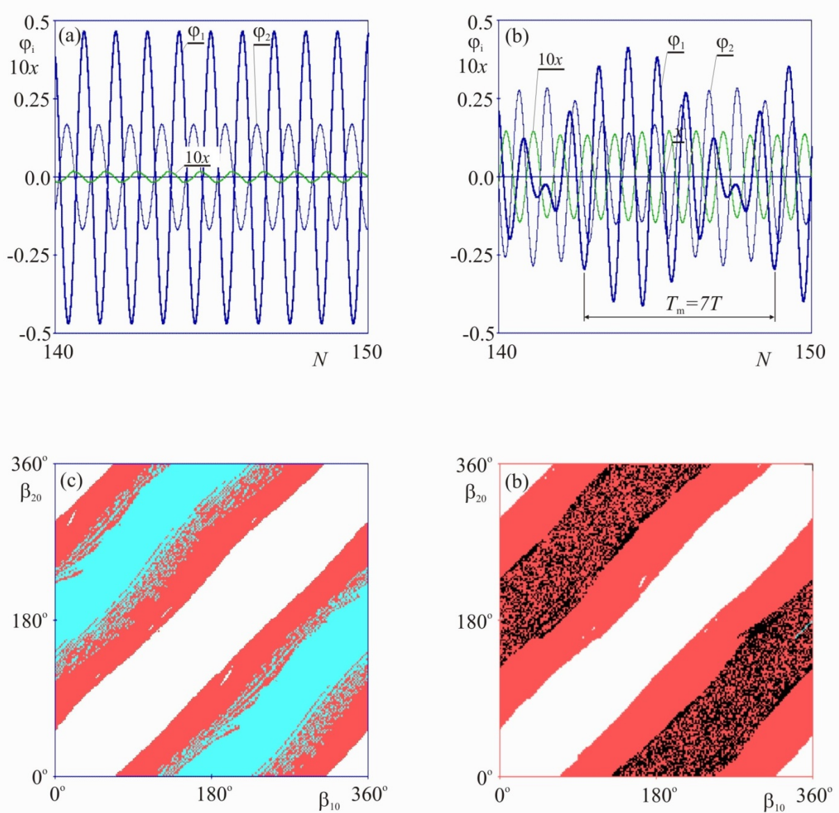
Figure 22. (Color online) Synchronization of two pendula with different masses: m_1=1.0 [kg], l=g/4\pi^2=0.2485 [m], M=10.0 [kg], c_x=1.53 [Ns/m], k_x=4.0 [N/m], \gamma_N=5.0^\circ , c_{\varphi l}=0.0083 [Ns], c_{\varphi 2}=0.0083 \times m_2 [Nsm], M_{Nl}=0.075 [Nm], M_{N2}=0.075 \times m_2 [Nm]; (a,b) time series of pendula \varphi_1 , \varphi_2 and beam x displacements, time on the horizontal axis is given in the following way t=NT , where N=1,2,3,\dots and T=1 [s], (a) phase synchronization: m_2=2.65 [kg], \beta_{10}=10^\circ , \beta_{20}=130^\circ ; (b) long period synchronization: m_2=2.65 [kg], T_m \approx 7T , \beta_{10}=1^\circ , \beta_{20}=90^\circ ; (c) basins of attraction of different types of synchronization: complete synchronization (white), phase synchronization (light grey, blue color online), long period synchronization (dark grey, red color online) in \beta_{10} - \beta_{20} plane: x(0)=0.0 , \dot{x}(0)=0.0 , \varphi_{i0} = \Phi \sin \beta_{i0} , \dot{\varphi}_{i0} = \alpha \Phi \cos \beta_{i0} , m_2=2.65 [kg], (d) basins of attraction of different types of synchronization: complete synchronization (white), long period synchronization (dark grey, red color online) chaotic behavior (black) in \beta_{10} - \beta_{20} plane: x(0)=0.0 , \dot{x}(0)=0.0 , \varphi_{i0} = \Phi \sin \beta_{i0} , \dot{\varphi}_{i0} = \alpha \Phi \cos \beta_{i0} , m_2=3.105 [kg].
