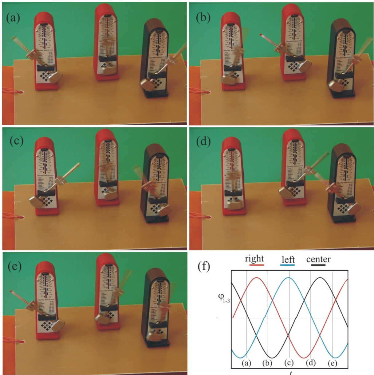
Figure 43: Three metronomes located on the plate which can roll on the base obtain a synchronous state with a phase difference \Delta\beta=|\beta_2-\beta_1|=|\beta_3-\beta_2|=|\beta_1-\beta_3|=2\pi/3 .
