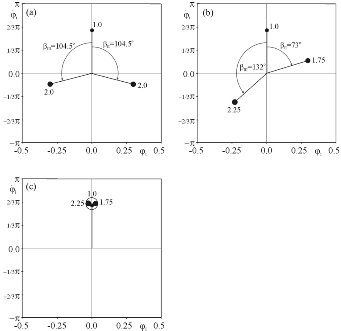
Figure 53. Synchronization configurations for three pendula; M=10.0 ; (a) symmetrical synchronization of three pendula m_1=1.0 [kg], m_2=m_3=2.0 [kg], \beta_{I0}=0^\circ , \beta_{II0}=60^\circ , \beta_{III0}=240^\circ , (b) unsymmetrical synchronization of three pendula m_1=1.0 [kg], m_2=1.75 [kg], m_3=2.25 [kg], \beta_{I0}=0^\circ , \beta_{II0}=60^\circ , \beta_{III0}=240^\circ , (c) full synchronization of three pendula m_1=1.0 [kg], m_2=1.75 [kg], m_3=2.25 [kg], \beta_{I0}=0^\circ , \beta_{II0}=25^\circ , \beta_{III0}=305^\circ .
