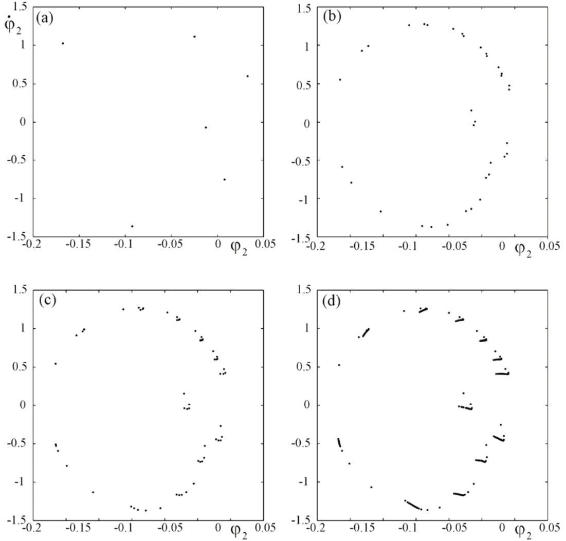
Figure 39: Poincaré maps (\varphi_2, \dot{\varphi}_2) for different (LPS) and chaotic attractors; m_1=1.0 [kg], m_2=3.105 [kg], l=g/4\pi^2=0.2485 [m], M=10.0 [kg], c_x=1.53 [Ns/m], k_x=3.94 [N/m], c_{\varphi 1}=0.0083 \times m_1 [Nsm], c_{\varphi 2}=0.0083 \times m_2 [Ns], M_{N1}=0.075 \times m_1 [Nm], M_{N2}=0.075 \times m_2 [Nm]: (a) \gamma_N=4.9^\circ , T=6 , (b) \gamma_N=5.2^\circ , T=35 , (c) \gamma_N=5.1^\circ , T=59 , (d) \gamma_N=4.9^\circ , chaotic behavior.
