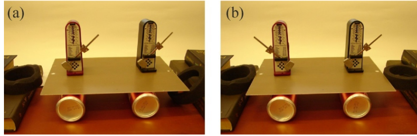
Figure 45: Two metronomes located on the plate which can roll on the base: (a) complete synchronization, (b) antiphase synchronization. Arrows indicate additional masses added to differentiate the total masses of the metronomes' pendula.
