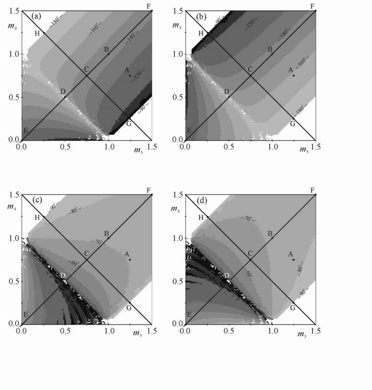
Figure 58. Contour maps of phase differences (a) \beta_{II} , (b) \beta_{III} , (c) \beta_{IV} , (d) \beta_V , versus pendula masses m_4 and m_5 ; m_1=m_2=m_3=1.0 [kg].
