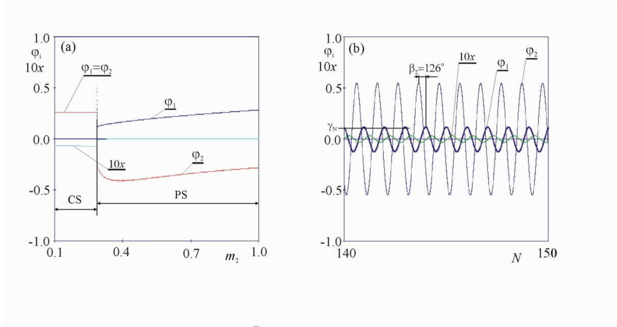
Figure 24: (Color online) (a) Bifurcation diagram of system (27,28): \varphi_1 , \varphi_2 and x versus control parameter m_2 ; m_2 decreases from 1.0 [kg] to 0.1 [kg], (b) time series of \varphi_1 , \varphi_2 and x during the phase synchronization: \Phi_1 \approx \gamma_N = 5.0^\circ , m_1 = 1.0 [kg], l = g/4\pi^2 = 0.2485 [m], M = 10.0 [kg], c_x = 1.53 [Ns/m], k_x = 3.94 [N/m], \gamma_N = 5.0^\circ , c_{\varphi_1} = 0.0083 [Nsm], c_{\varphi_2} = 0.0083 \times m_2 [Nsm], M_{N1} = 0.075 [Nm], M_{N2} = 0.075 \times m_2 [Nm].
