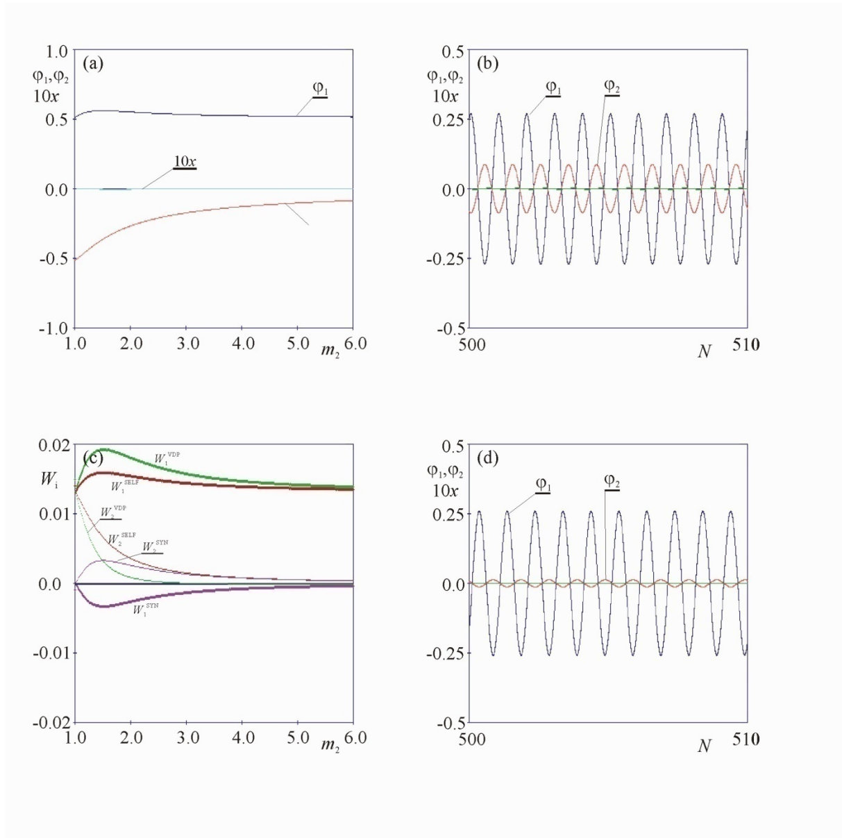
Figure 31: Evolution from antiphase to almost antiphase synchronization; (a) bifurcation diagram for increasing values of m_2 , (b) time series of almost antiphase synchronization for m_1=1.0 [kg] and m_2=1.5 [kg], (c) energy plots, (d) time series of almost antiphase synchronization for m_1=1.0 [kg] and m_2=20.0 [kg].
