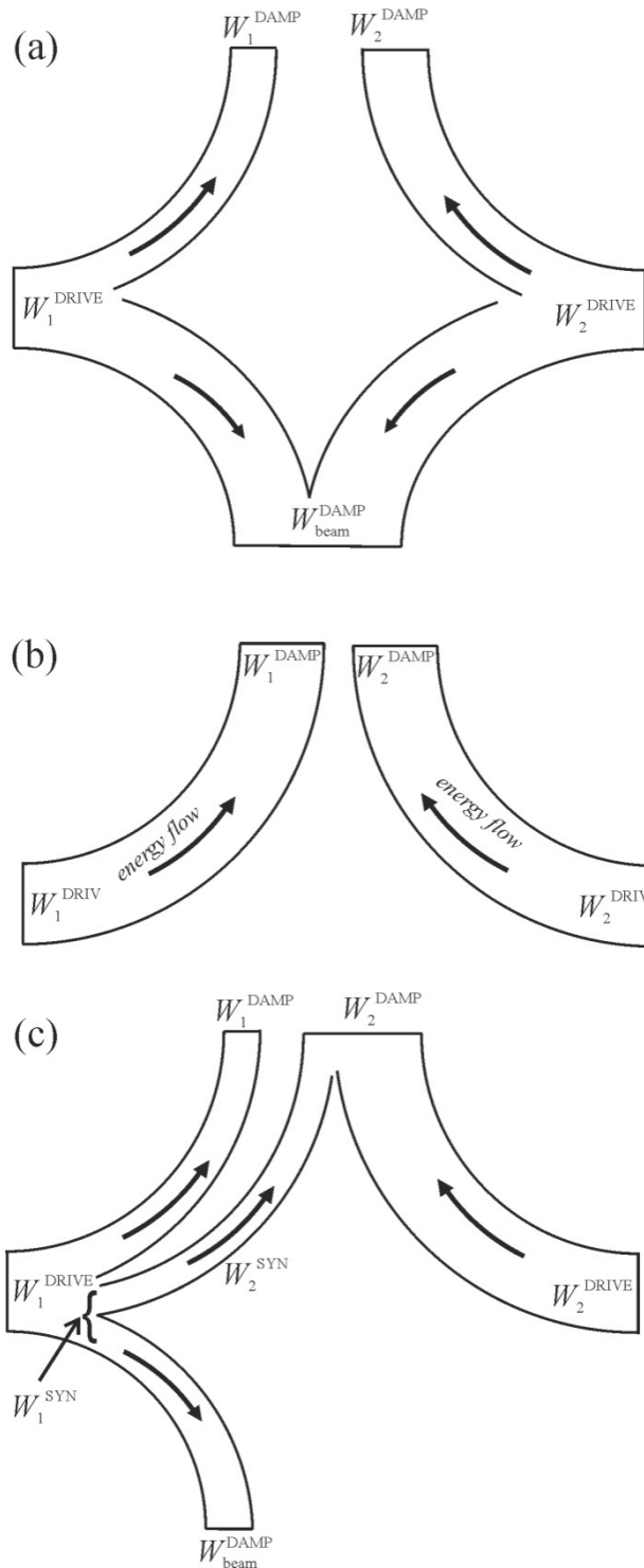
Figure 41. Energy balance schemes: (a) almost complete synchronization – both pendula drive the beam, (b) antiphase synchronization – beam at rest, (c) almost antiphase synchronization – pendulum 1 drives the beam and supplies energy to pendulum 2.
