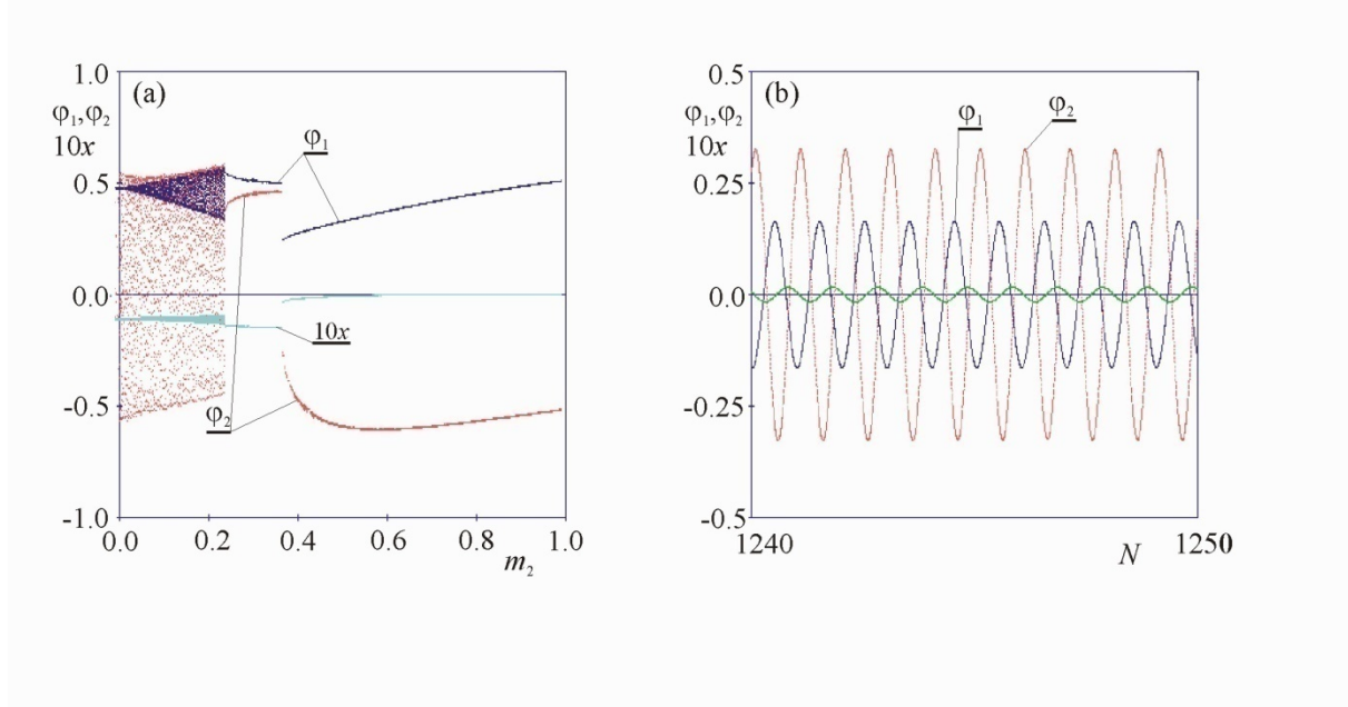
Figure 32: Evolution from antiphase synchronization to quasiperiodic oscillations; (a) bifurcation diagram of system (27,28) for decreasing m_2 , (b) time series of almost antiphase synchronization for m_1 = 1.0 [kg], m_2 = 0.5 [kg].
