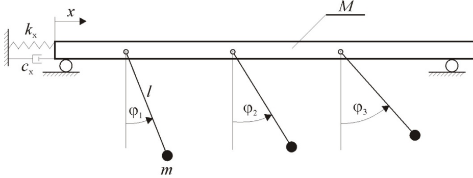
Figure 47: The model of n pendulum clocks hanging from an elastic horizontal beam.
