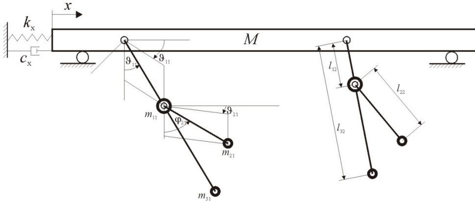
Figure 15: Huygens' experiment modeled with two coupled double spherical pendula.
