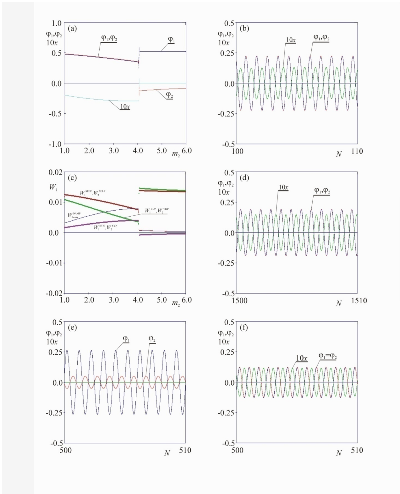
Figure 27: Evolution from complete to almost antiphase synchronization; (a) bifurcation diagram for increasing values of m_2 , (b) time series of almost complete synchronization m_1=1.0 [kg] and m_2=2.0 [kg]; (c) plots of system's energy; (d) time series of almost complete synchronization for m_1=1.0 [kg] and m_2=3.5 [kg]; (e) time series of almost antiphase synchronization: m_1=1.0 [kg], m_2=5.0 [kg]; (f) nonstationary complete synchronization: m_1=m_2=3.0 [kg].
