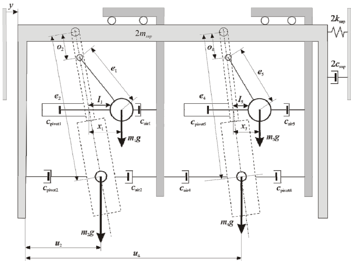
Figure 14: Senator's model of the Huygens experiment (after [96]).
