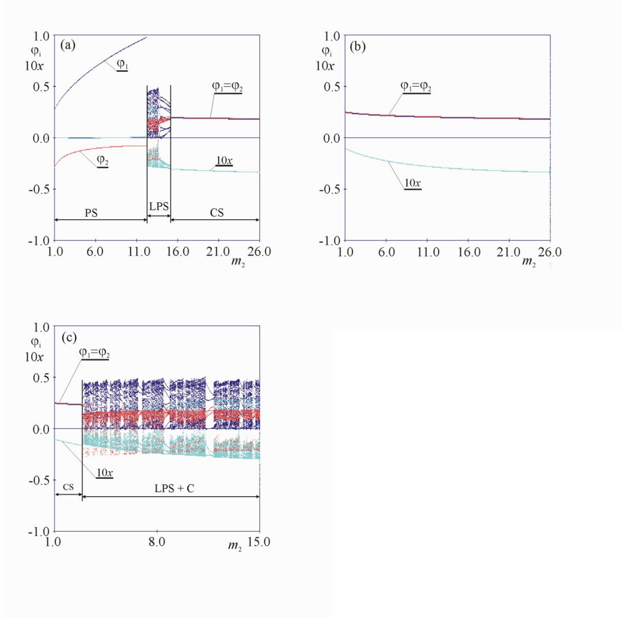
Figure 23: (Color online) Bifurcation diagrams of system (27,28): \phi_1 , \phi_2 and x versus control parameter m_2 : \Phi_1 \approx \gamma_N = 5.0^\circ , m_1 = 1.0 [kg], l = g/4\pi^2 = 0.2485 [m], M = 10.0 [kg], c_x = 1.53 [Ns/m], k_x = 3.94 [N/m], \gamma_N = 5.0^\circ , c_{\phi 1} = 0.0083 [Nsm], c_{\phi 2} = 0.0083 \times m_2 [Nsm], M_{N1} = 0.075 [Nm], M_{N2} = 0.075 \times m_2 [Nm]; (a) m_2 increases from 1 to 26.0, (b) m_2 decreases from 26.0 to 1.0, (c) m_2 decreases from 15.0 to 1.0.
