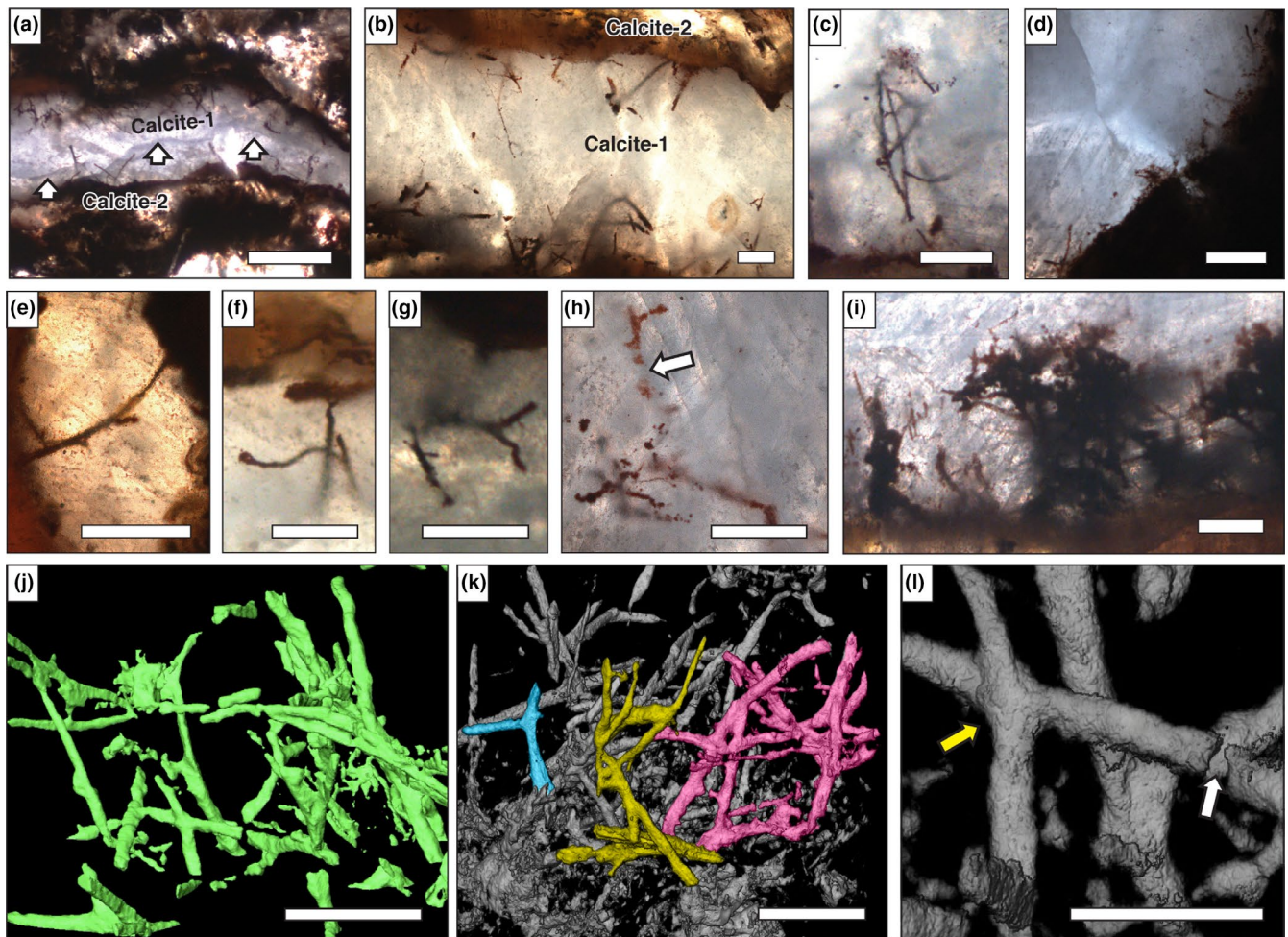
FIGURE 2 Photomicrographs (a–i) and synchrotron X-ray microtomography renderings (j–l) of filament assemblages in calcite veins. All photomicrographs were taken in plane-polarized transmitted light. (a) Calcite vein with filaments from Locality 1, showing somewhat blocky calcite with irregular median suture (arrowed). (b) Opaque filaments clustering on both sides of Calcite-1 within a vein mantled by brown, fibrous Calcite-2 (Locality 1). (c) Curving, connected filaments (Locality 1). (d) Filaments from Locality 2. (e) A curved, possibly branched filament spanning the thickness of Calcite-1 (Locality 1). (f) A branching filament that swells towards the tip (Locality 1). (g) A branching filament (Locality 1). (h) Branching filaments with patchy preservation; arrow indicates gap (Locality 1). (i) An unusually dense population of filaments (Locality 1). (j) A three-dimensional view of the filaments in I showing curved trajectories; image is a cropped still frame from the supplementary movie. (k) An alternative view of the same region as i and j, showing numerous branches and interconnections; three contiguous regions are highlighted in color. (l) Another view of the same region as i, j, and k; white arrow indicates a conspicuous gap in one filament. This field of view shows an “X”-shaped pseudo-junction (yellow arrow) where filaments grazing each other are cemented together (and/or merged by the process of computing a surface through the rather diffuse filament margins). Some apparent connections seen in panel 2K may also result from these effects. Scale bars: 500 \mu\text{m} (a); 100 \mu\text{m} (b–i); 50 \mu\text{m} (j, k); 20 \mu\text{m} (l)
