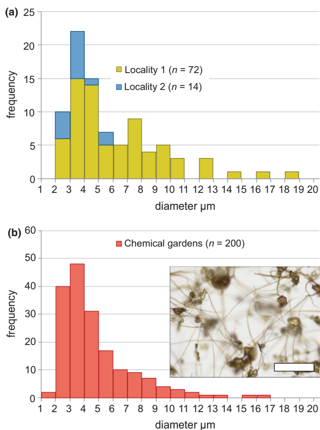
FIGURE 5 Histogram comparing diameters of Ligurian filaments and chemical gardens. (a) Diameters of filaments in calcite veins were similar at two localities ~4 km apart (for map positions see Figure 1). (b) Diameters of tubular filaments in abiotic chemical gardens produced by McMahon (2019) from seed particles <63 \mu\text{m} . Inset: photomicrograph of chemical garden filaments included in the population represented by the histogram. Scale bar: 200 \mu\text{m}
