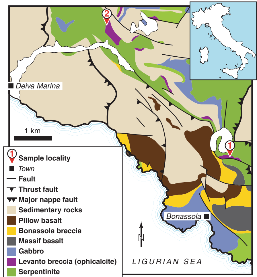
FIGURE 1 Geological map showing the localities of filament-bearing calcite vein samples collected inland from Bonassola (1) and Deiva Marina (2). Adapted from Strating and Wamel (1989)
