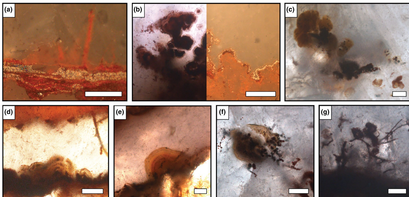
FIGURE 4 Photomicrographs of hematite +Mg-silicate microstructures. (a) Laminated cements lining the inner edge of Calcite-1, with attached red filaments (reflected light). (b) A ramifying growth structure somewhat similar to “Frutexites” in transmitted (left) and reflected (right) light; only the exterior of the structure appears to be laminated. (c) Globular, non-laminated growths (transmitted light). (d) Laminated domal growths (transmitted light). (e) Individual laminated dome (transmitted light). (f) Laminated irregular spheroid attached to filaments (transmitted light). (g) Blobs attached to filaments (transmitted light). All scale bars 50 \mu\text{m}
