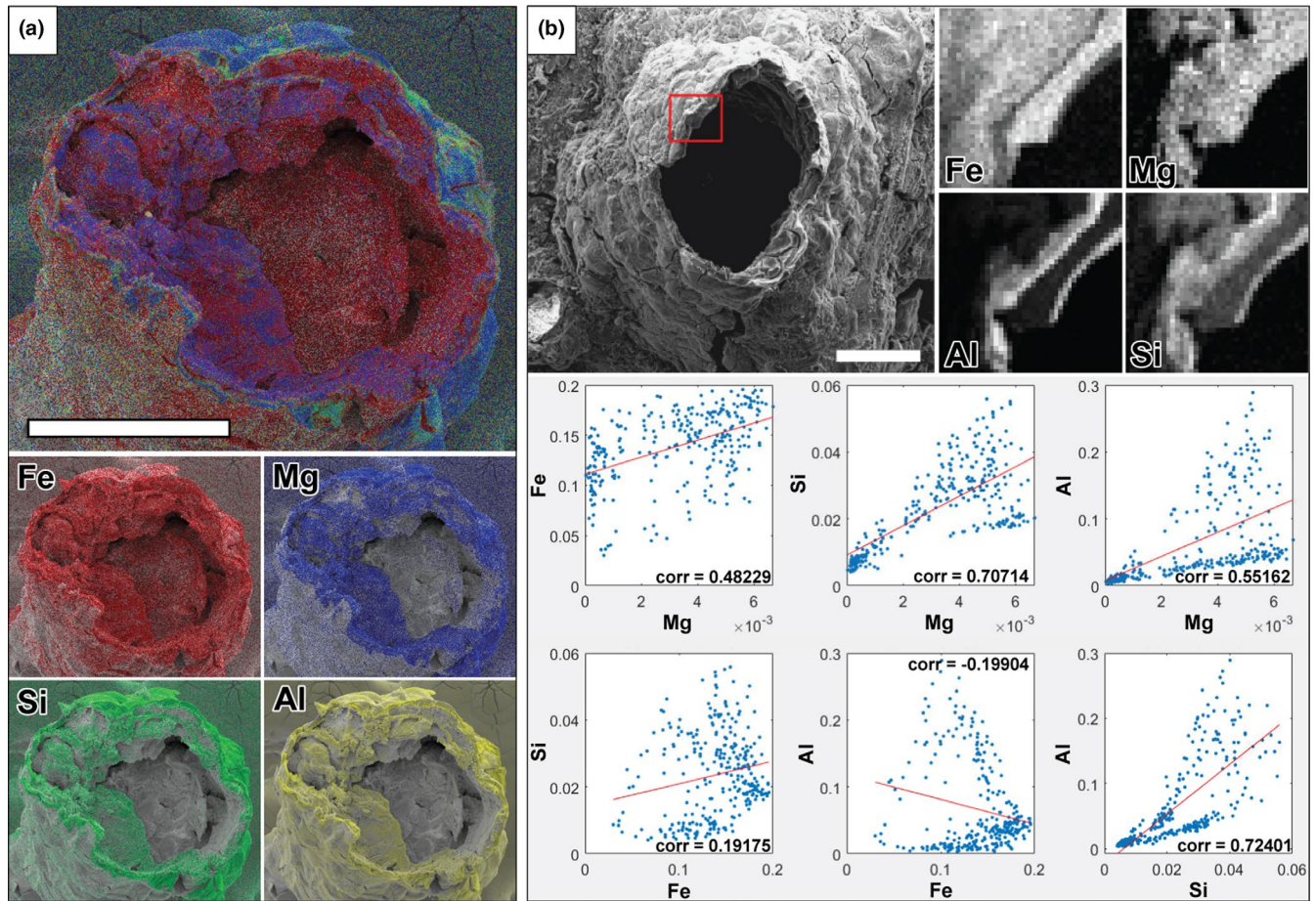
FIGURE 6 Element distributions in experimental chemical gardens produced from polymetallic seed salts. (a) EDS maps of Fe, Mg, Si and Al overlaid on SEM image of chemical garden tube. Note that the innermost precipitates are dominated by Fe, while Mg, Si and Al are present in layers in the wall. Scale bar = 250 \mu\text{m} . (b) Associations between elements in a chemical garden tube wall. Top-left: SEM image (scale-bar = 250 \mu\text{m} ) of an experimental chemical garden tube; red box shows region of element maps (scale-bar = 25 \mu\text{m} ). Note multi-layer structure different from that shown in Figure S3. Top right: coarsened, normalized element maps show the boxed region. These were used to calculate correlation coefficients; each pixel provides one point in the scatterplots, below
