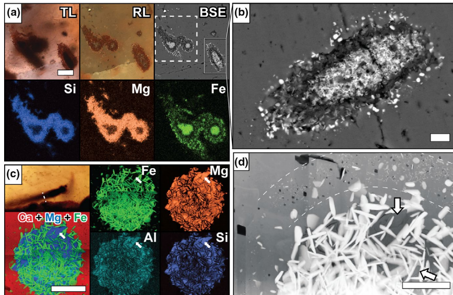
FIGURE 3 Optical and electron microscopy and energy-dispersive X-ray spectroscopy of filaments in calcite veins (Locality 1). (a) Thick filaments intersecting the surface of a polished thin section, imaged in transmitted light ("TL"), reflected light ("RL") and by means of backscattered electron microscopy ("BSE"), revealing a concentric structure that is typical of most filaments at both localities. Element maps obtained by energy-dispersive X-ray spectroscopy show the distribution of Fe (present as hematite), and Mg + Si (probably talc) within the filaments. Al is also slightly enriched in the Mg + Si phase (not shown). (b) Close-up of the BSE image in (a), showing the slightly diffuse, microcrystalline nature of the filaments and their biminerale structure. This filament is dissected obliquely by the thin section surface. (c) A filament subjected to FIB-milling to extract an ultrathin wafer, shown in transmitted light (with dashed line indicating line of FIB section) and in element maps of Mg, Al, Si and Fe show that the first three of these elements are present in the same mineral while Fe occurs in a different mineral. Arrows indicate a prominent group of lath-shaped Al-bearing Mg-silicate crystals also visible in (d). (d) A scanning transmission electron micrograph view of the filament shown in (c). Arrows indicate lath-like Mg-silicate crystals, which show dark grey against the white platy hematite crystals. Dashed lines enclose a diffuse outer halo of hematite. Scale bars: 25 \mu\text{m} (a), 5 \mu\text{m} (b, c), 2.5 \mu\text{m} (d)
