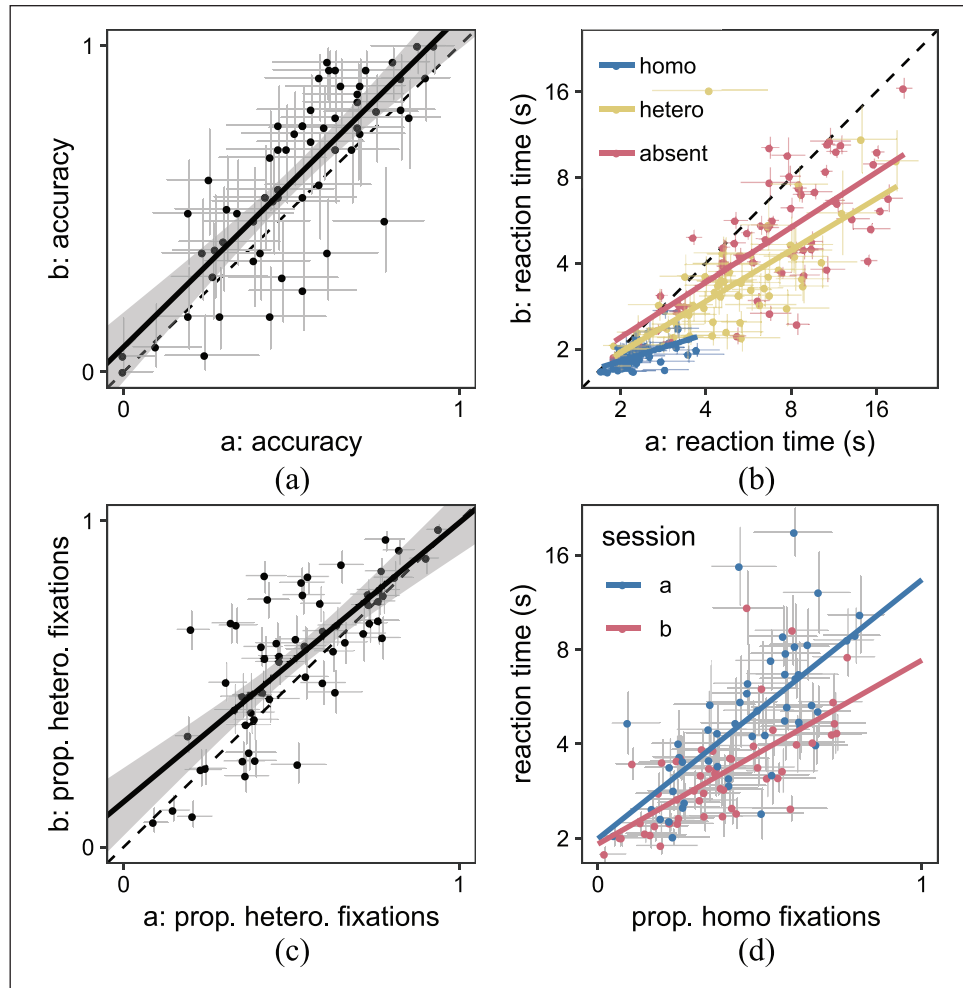
Figure 2. Correlation between the two sessions of the SHLS paradigm for (a) accuracy (TP-heterogeneous trials only), (b) reaction times, and (c) search strategy (TA trials only). (d) Initial search strategy correlates with reaction times in both sessions. Each point represents a participant and the error bars indicate 95% confidence intervals.
