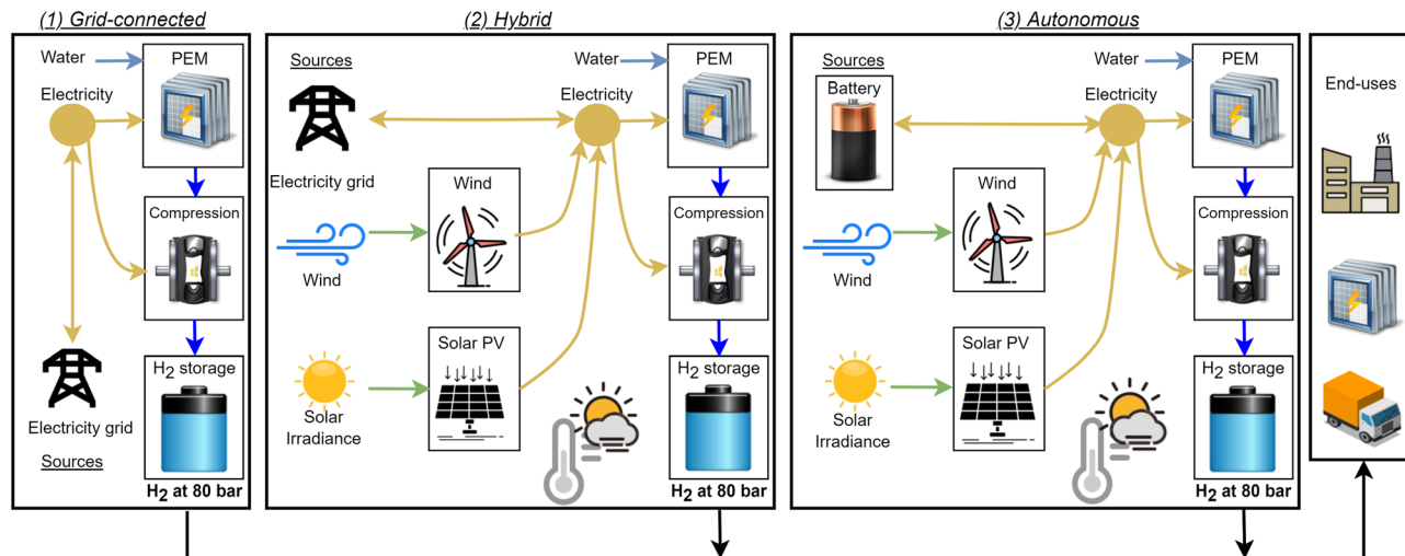
Fig. 2 Simplified illustration of the system boundaries of the three considered hydrogen production configurations: (1) grid-connected, (2) hybrid, and (3) autonomous, from left to right. Potential end uses are visualized, but are not considered in our system boundaries. For simplicity, desalination and deionisation of water are not visualized here, but are considered in our cost quantification and environmental LCA.
