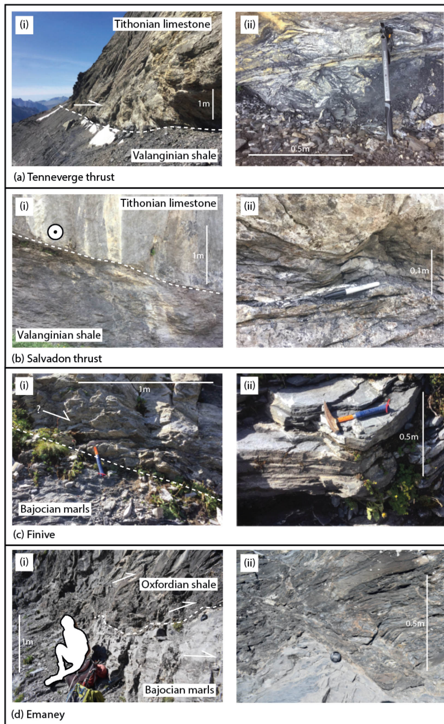
Figure 2. “Strained” localities. (a) Tenneverge thrust, showing (i) Tithonian limestone in the hanging wall thrust at a low angle over Valanginian shale, and (ii) a close-up of the thrust surface, showing penetration of the fault zone into the footwall shales. (b) Salvadon thrust, showing (i) the thrust surface at outcrop scale, with Tithonian limestone thrust over Valanginian shales, and the direction of displacement obliquely out of the page; (ii) a close-up view of the thrust surface, showing a clear step change in lithology and small undulations in the surface. (c) Finive shear zone and thrust splay, with (i) the fault exhibiting displacement on a 1 to 10 m scale, occupying the apparent geometry of a low-angle normal fault; (ii) ductile fabrics of the surrounding shear zone. (d) Emaney shear zone, demonstrating (i) the partitioning of strain into the overlying shales, evident in the differing fabric intensities; (ii) a close-up of the boundary between the two units.
