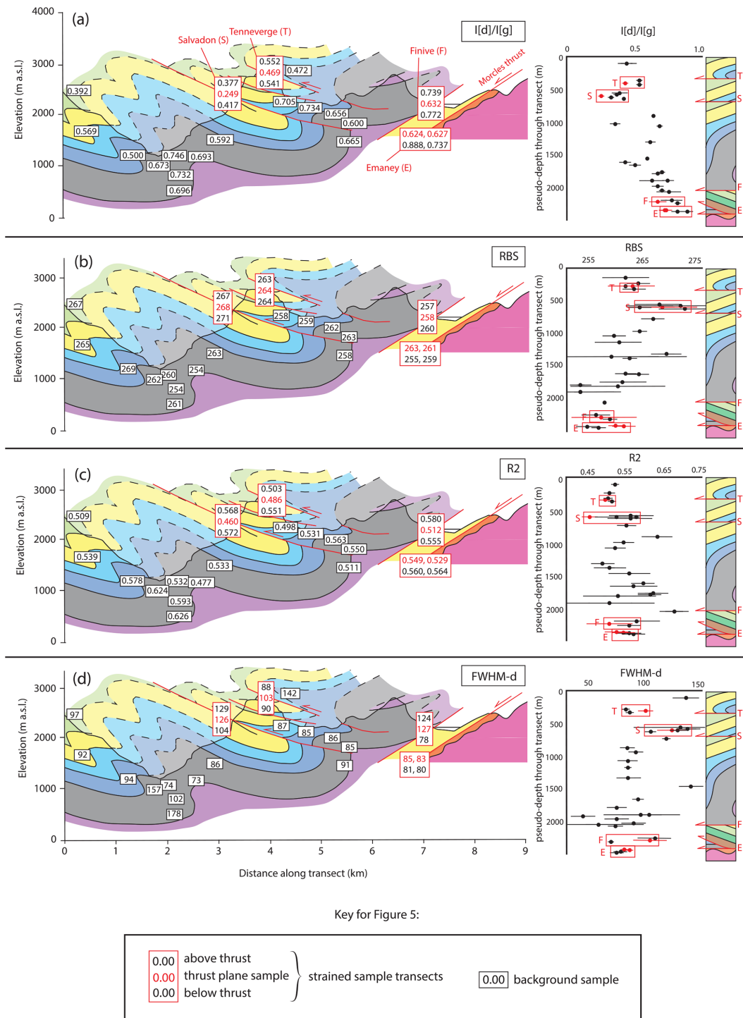
Figure 5. Cross-sections and depth transects showing values of (a) I_D/I_G , (b) Raman band separation, (c) area ratio R^2 , and (d) D-peak width. Labelled values on cross-sections indicate the approximate position of samples, with numbers in black boxes representing “background” samples and those in red boxes indicating samples through “strained” localities. Within strained localities, red numbers represent fault plane or shear zone samples. The depth transects on the right of each panel are accompanied by a simplified stratigraphic column for reference. Strained localities are highlighted by red boxes labelled with a corresponding letter (T: Tenneverge, S: Salvador, F: Finive, E: Emaney), with the thrust plane or shear zone sample indicated by a red dot. Horizontal lines on transects are error bars (standard deviation for all spectra and deconvolutions for that sample).
