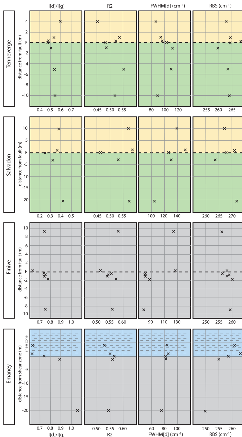
Figure 6. Plots showing the four main Raman parameters in this study ( I_D/I_G , R^2 , FWHM[d] , and RBS ) for each of the four “strained localities” (Tenneverge, Salvadon, Finive, and Emaney), with height in metres above (and below) each thrust plane or shear zone labelled on the y axis of each panel. Note that the scale for each plot within a column is the same, but the bounds of the x axis may change. Within each row, lithology is represented by colour, corresponding to the rest of the paper (grey: Bajocian, blue: Oxfordian, yellow: Tithonian, green: Valanginian). Additionally, black dotted lines indicate the presence of a thrust at that height, while grey dashes indicate a shear zone.
