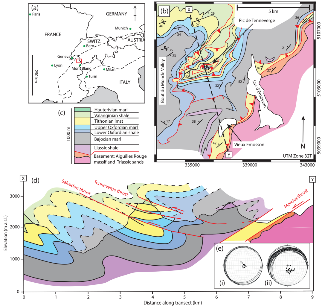
Figure 1. Geology of the Haut Giffre. (a) Location of the Haut Giffre region (red box) within the Alpine chain (dashed lines) on the French–Swiss border. (b) Simplified geological map of the eastern Haut Giffre, including major thrust faults and regional dips. Significant geographic features are labelled. The cross-section line x – y is indicated by a dashed line. (c) Main lithological units outcropping in the Haut Giffre. (d) NNW–SSE cross-section as indicated by line x – y in (a) . (e) Stereonets showing cleavage and poles to cleavage at the (i) highest stratigraphic levels (lower Oxfordian and above, limited to Pic de Tenneverge massif) and (ii) lowest stratigraphic levels (within 1 km of the Morcles thrust).
