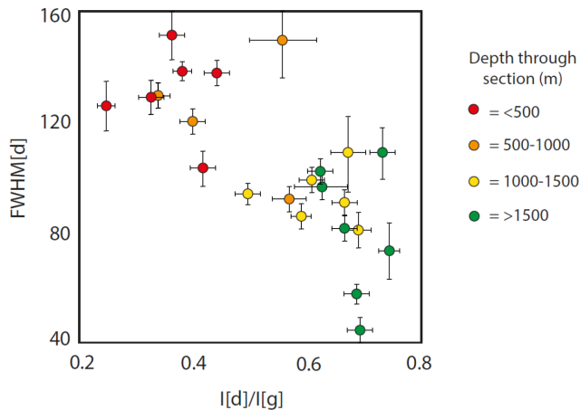
Figure 7. D-peak width (FWHM[d]) plotted against intensity ratio ( I_D/I_G ), with points coloured by depth through the overall transect.
