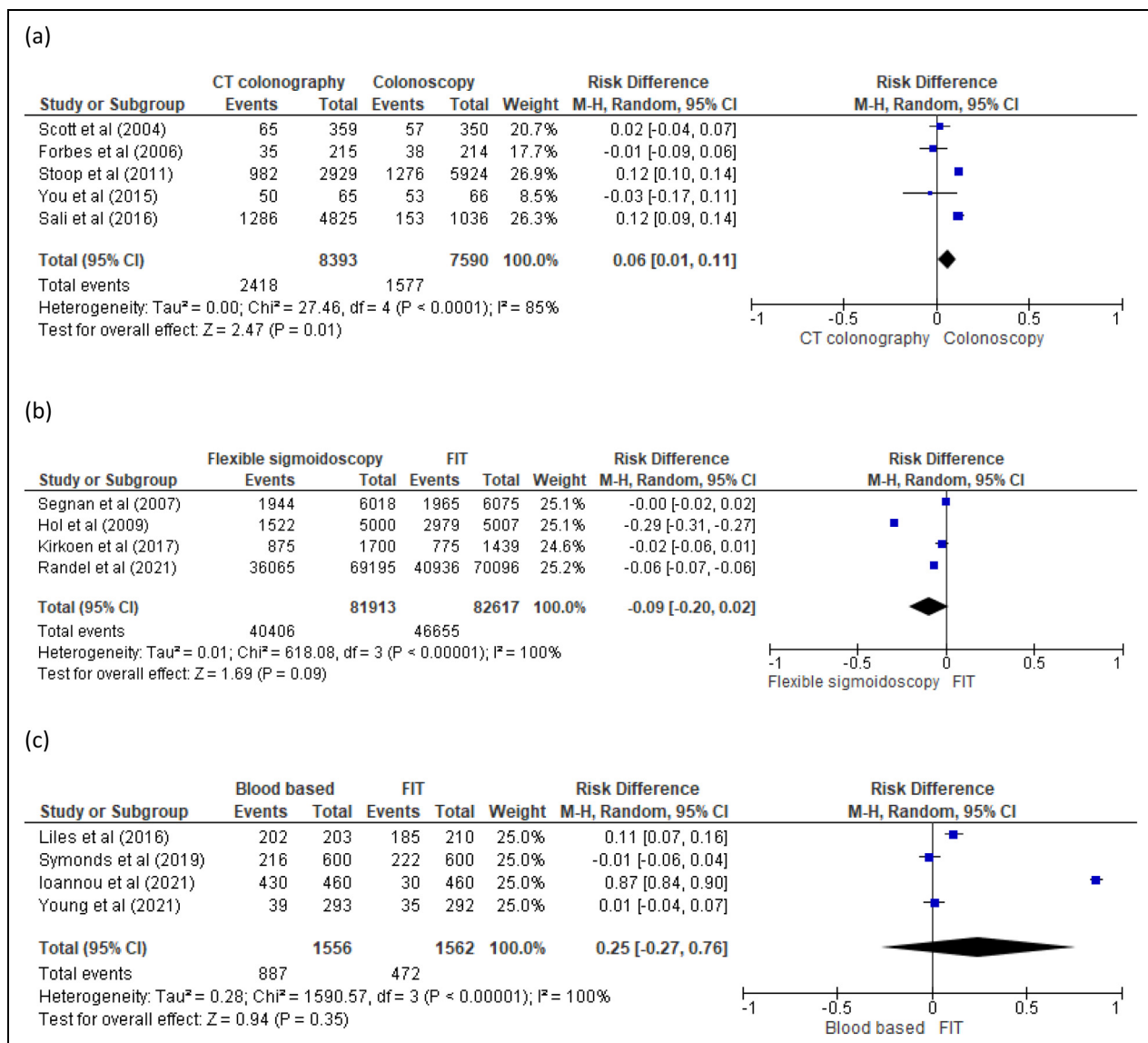
Figure 2. (a) Pooled results of uptake for computed tomography (CT) colonography and colonoscopy. (b) Pooled results of uptake for flexible sigmoidoscopy (FS) and FIT. (c) Pooled results of uptake for blood based and faecal immunochemical test (FIT).
