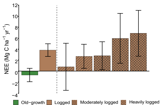
Fig. 3. Net ecosystem \text{CO}_2 exchange (NEE) estimated by biometric ground-based methods. Left of the dashed line show the mean ( \pm SE) of six unlogged forest plots (green) and five logged plots (brown) with error bars representing variation across the plots. Right of the dashed line show the logged plots individually: two moderately logged plots (striped; Left to Right: SAF-03, SAF-04), and three heavily logged plots (hatched; Left to Right: SAF-01, SAF-02, SAF-05) with error bars representing within-plot uncertainty, estimated by propagation of SEs of the individually measured components of productivity and respiration. Positive values indicate a net source of \text{CO}_2 to the atmosphere.
