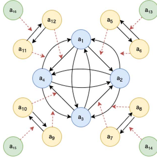
Fig. 1. Argumentation graph corresponding to stag hunt game.
