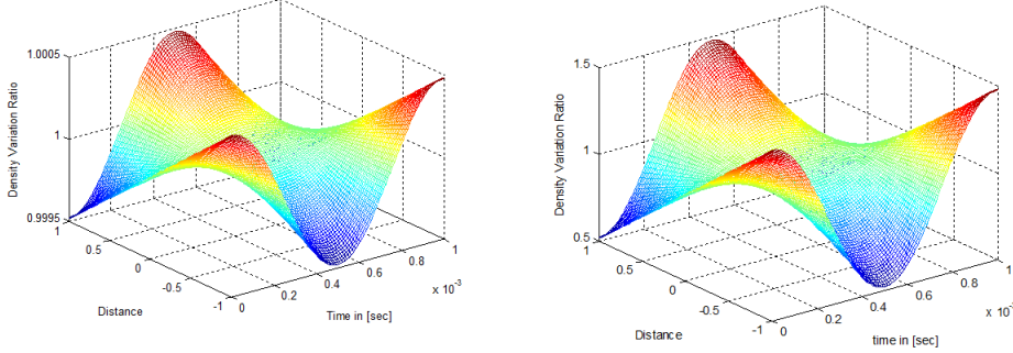
FIGURE 2. Density ratio variation with 1kHz, 1 cm amplitude, N_0 = 1000 (left), and N_0 = 10^6 (Right)
