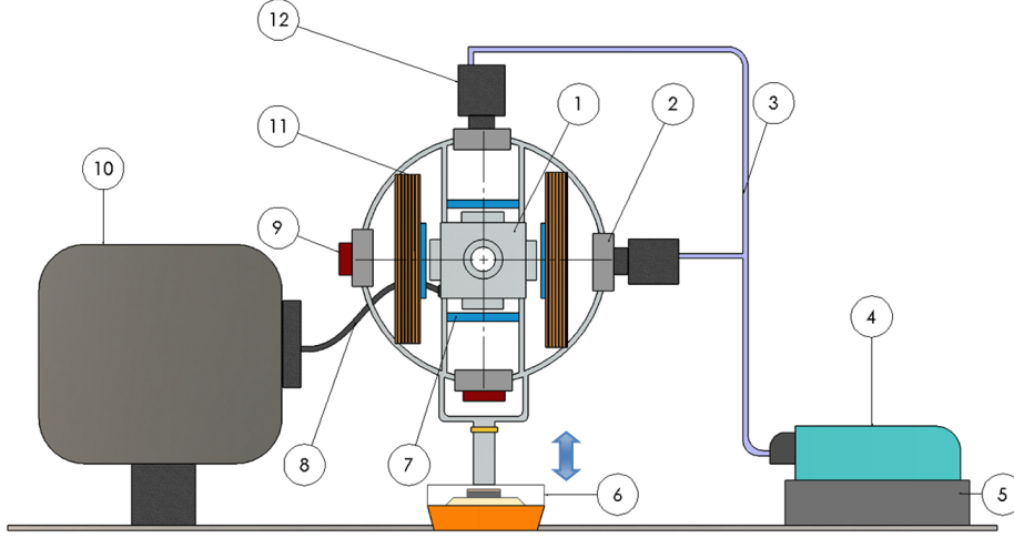
FIGURE 1. Experiment setup, 1- trap, 2- quarter wave plate, 3- fibre optics, 4- tuneable laser, 5- electro-acoustic vibrator drive, 6- electro-acoustic vibration generator, 7- TOP magnetic coils, 8- flexible vacuum pipe, 9- mirror, 10- ion pump, 11- trap magnetic coils (MOT), 12- telescope
