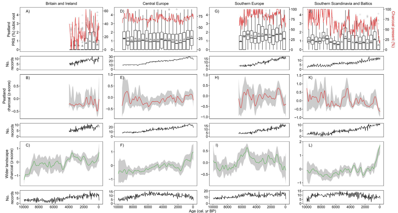
Fig. 4. Peatland and wider landscape burning trends by European sub-region. The distribution of proportionally relatively scaled (PRS) charcoal values (cubic root transformed) in 500-year bins for A) Britain and Ireland, D) Central Europe, G) Southern Europe and J) Southern Scandinavia and Baltics; box heights represent the upper and lower quartiles, central lines indicate medians, hollow triangles represent means, whiskers extend to 1.5 times the interquartile range beyond the upper and lower quartiles, and hollow circles represent any values outside the range of these whiskers. Trends in the proportion of records (%) with charcoal present within 50-year bins indicated by the red line. Biomass burning trends for peatlands in B) Britain and Ireland, E) Central Europe, H) Southern Europe and K) Southern Scandinavia and Baltics and wider landscape biomass burning for C) Britain and Ireland, F) Central Europe, I) Southern Europe and L) Southern Scandinavia and Baltics – all with a 500-year smoothing window and showing 95% bootstrap confidence intervals (1000 cycles). The x-axis units (cal. yr BP) represent years before 1950 CE. For each panel the number of sites corresponds to 50-year time steps.
