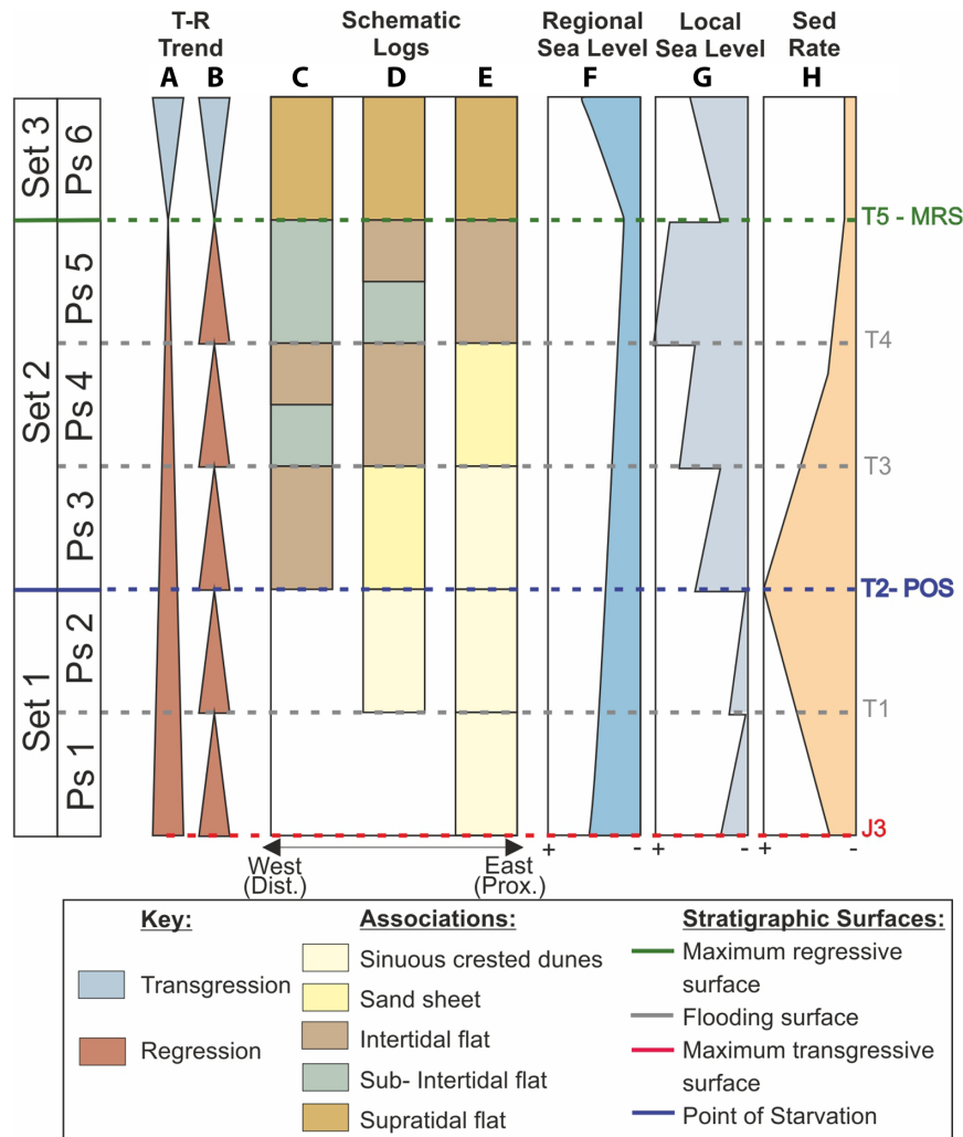
FIGURE 9 Cyclicity and sequence stratigraphy within the studied Curtis–Summerville formations. The left-hand side separates the interpreted units into parasequences. (A) Broad-scale transgressive-regressive sequence from the maximum transgressive surface of the J-3 to the maximum transgressive surface within the Summerville. Red represents regression, blue represents transgression. (B) Smaller scale transgressive and regressive events. Red represents regression and blue represents transgression. (C–E) Schematic logs of the associations identified from the distal setting with tide-dominated shallow-marine deposits, through to the proximal setting with continental aeolian deposits. (F) Regional sea-level fluctuation associated with the broad-scale transgressive-regressive sequence. (G) Local-scale sea-level fluctuations associated with the smaller-scale transgressive and regressive events. (H) Interpreted sedimentation rate curve across the margin, note the rate of sedimentation increases to the point of starvation and then decreases towards the maximum regressive surface.
