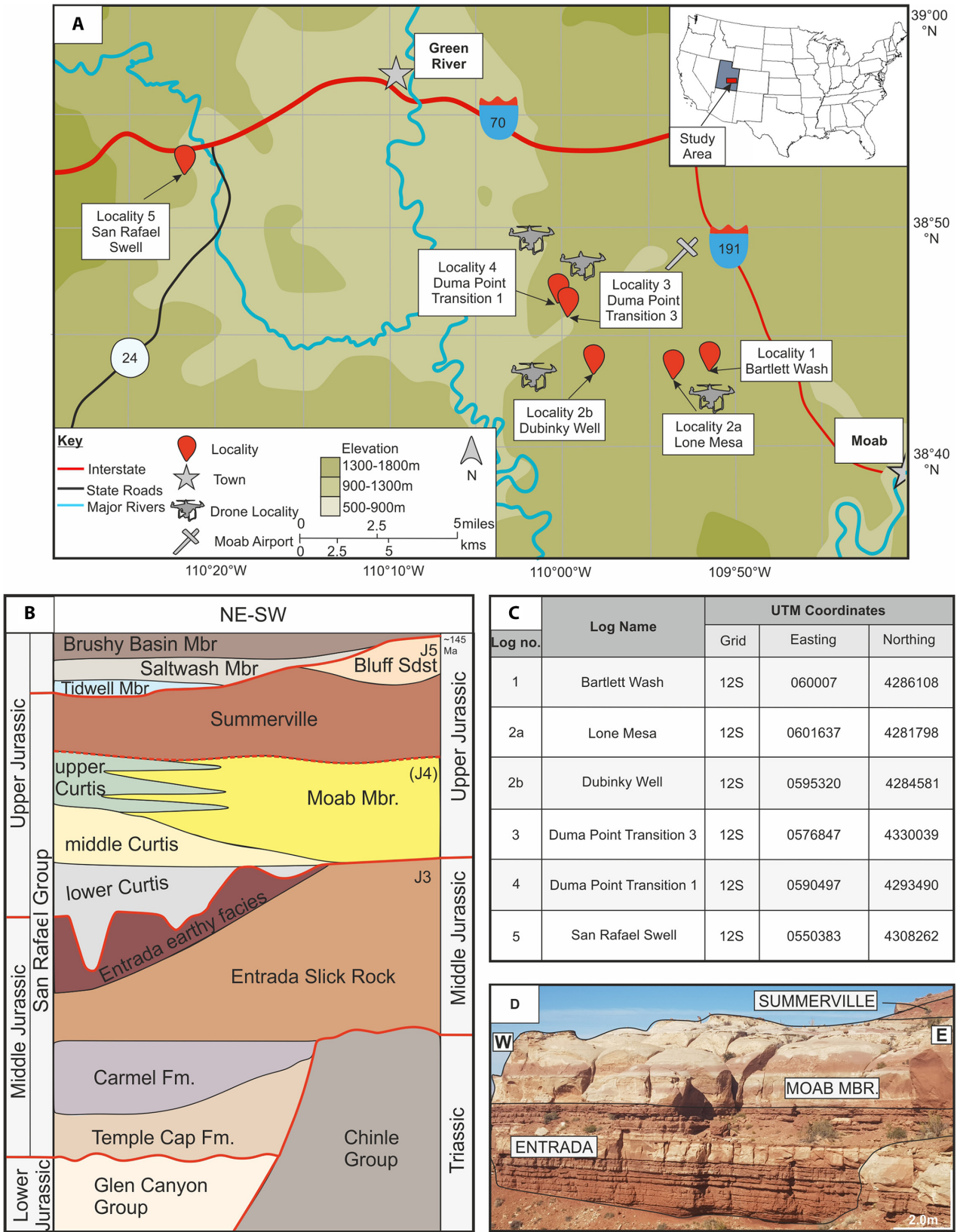
FIGURE 1 (A) Map of the study area, documenting the localities taken across the study area. Locations where a drone survey was conducted is indicated with a drone symbol. Top right contains a map of the United States of America, the state of Utah and the study area highlighted within. (B) Schematic lithostratigraphic column showing correlation between late Triassic and Jurassic deposits between Central Utah and Northern New Mexico (after, Zuchuat, et al., 2019a, 2019b). (C) Logs and locations taken across the study area. (D) Representative field photograph showing the relationship between formations analysed by this study.
