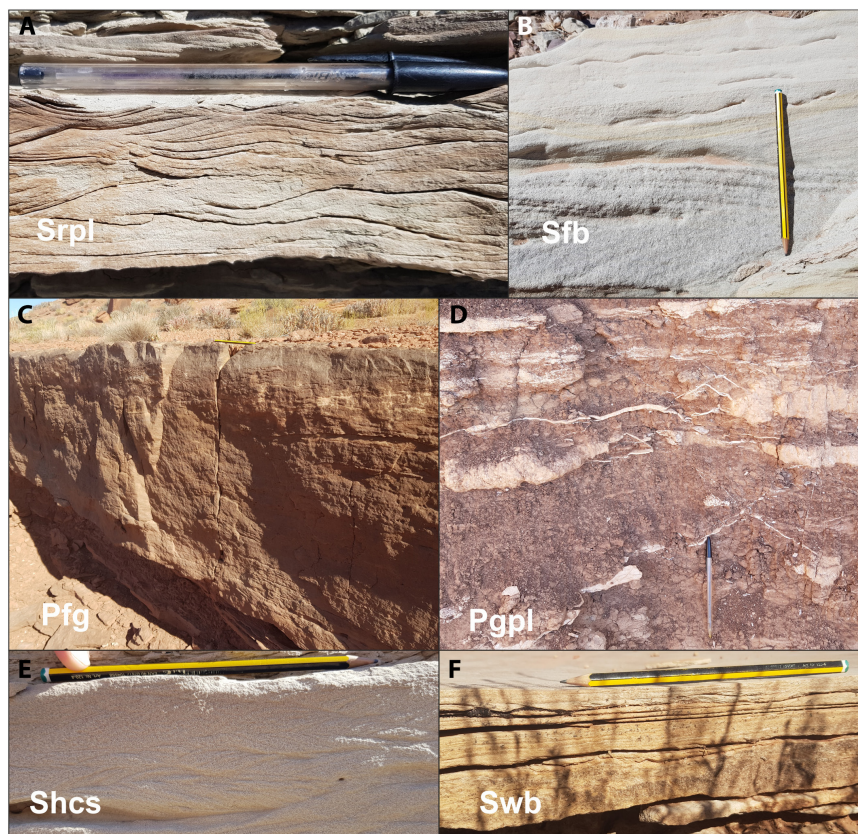
FIGURE 4 (A) Wavy ripple laminated sandstones at 5: San Rafael Swell, note the round-crested ripples and internal lamination indicating relatively deep water with a high sediment load. (B) Flaser bedded sandstones at 5: San Rafael Swell, cavities in the ripple peaks are the result of erosion of finer-grained material, a clear indicator of a tidal environment. (C) Ferric gley soil preserved at 3: Duma Point Transition 3, vertical burrows and evidence of rooting are visible. (D) Vein and laminar beds of gypsum within the parallel laminated gypsisol facies at 5: San Rafael Swell, note the vein gypsum bisects the bedded gypsum and is therefore likely to be a secondary feature. (E) Herringbone cross-stratified sandstone facies at 5: San Rafael Swell, the bidirectional preserved ripples are a clear indicator of a tidal environment. (F) Wavy bedded sandstone at 4: Duma Point Transition 3, round-crests and some immature ripple development indicates very shallow water with low sediment supply.
