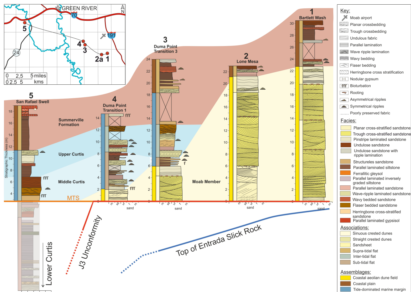
FIGURE 2 (A) Map of localities where sedimentary logging was conducted, transect line is marked. (B) Sedimentary logs at each locality, coloured by facies with the associations and assemblages represented down the left side of each log. Sedimentary structures of note are shown on the right-hand side. Where outcrops were inaccessible, the depth has been estimated and marked with a cross.
