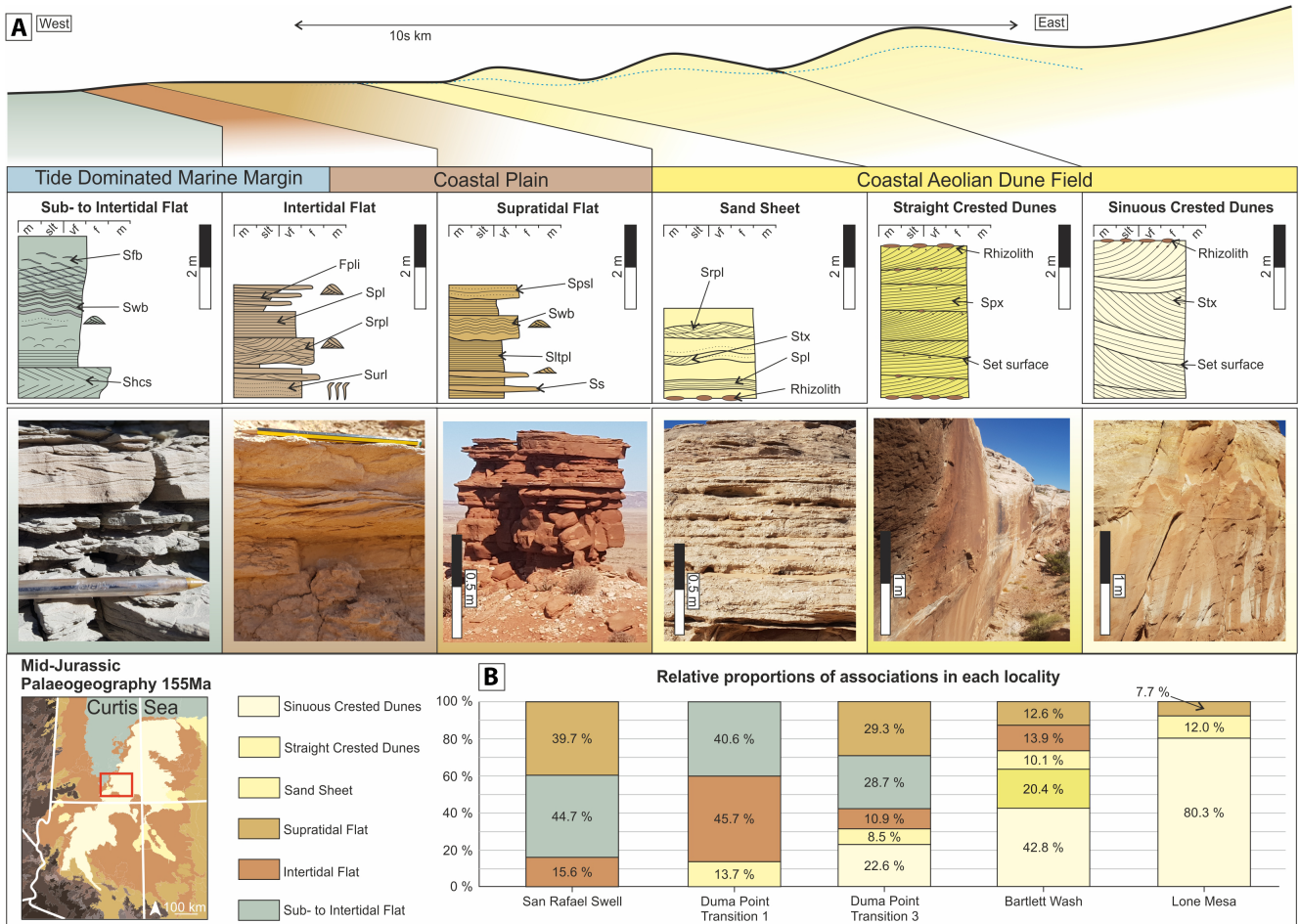
FIGURE 5 (A) Schematic diagram showing the spatial transition between associations east to west across the study area. Sinuous-crested dunes transition into smaller sinuous-crested and straight-crested dunes before deflating into a sandsheet. The supratidal flat expands both landward and seaward grading into an intertidal flat, and once the water depth becomes significant enough, a subtidal-intertidal flat. (B) Relative proportions of each association at each locality.
