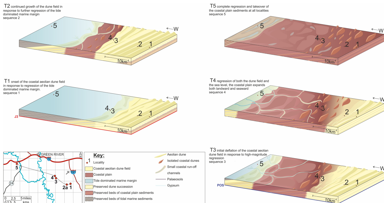
FIGURE 8 Depositional environment models for the temporal translation of assemblages. T1 represents the regression of the Curtis Sea and the development of the Moab Member dune field following the major transgressive event preserved within the J-3. T2 marks continued development of the dune field, with dune size and complexity increasing with continued fall in sea level. T3 represents the point of starvation, after which the dune field begins to deflate and the coastal plain begins to expand both landward and seaward. T4 shows the inability of the dune field to recover from this high-magnitude, rapid regression, shutting down sediment supply and preserving small dune forms and sand sheets. T5 marks the final shut down of all aeolian processes in the east of the study area and the complete takeover of the coastal plain sediments of the Summerville Formation.
