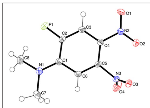
Scheme 12. The molecular structure of compound 12 showing 50% displacement ellipsoids.
