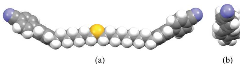
Figure 11. (Colour online) (a) Space filling model for CB7S9CB and (b) viewed along the spacer.
