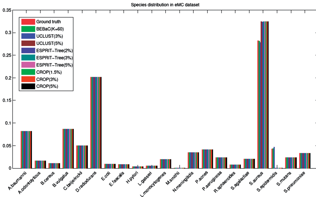
Figure 4. Reconstructed species distributions given by different software. BEBaC( K = 60 ) and UCLUST(3%) is almost the same as the ground truth, whereas the other software fails to detect the proportions of S. aureus and S. epidermidis . C. albicans is not detected by any software, thus we did not show it in this figure. M. smithii is correctly detected by all software, although this OTU only contains 14 sequences.
