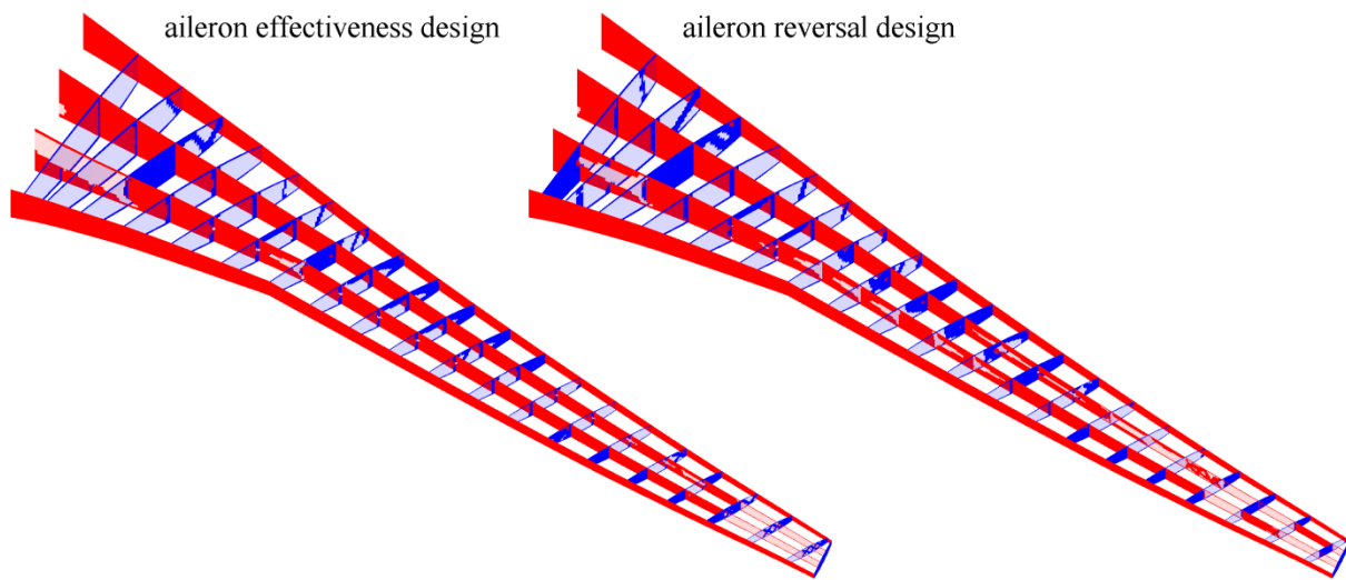
Figure 15. Optimal topologies considering aileron rolling metrics.
