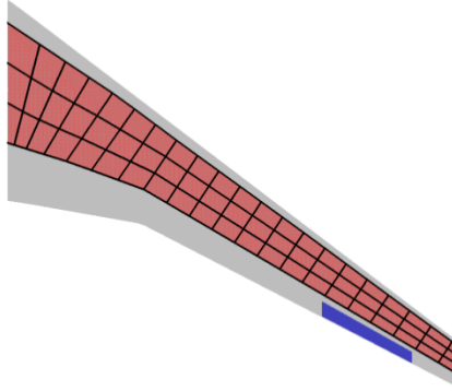
Figure 13. Outboard aileron placement and geometry.
