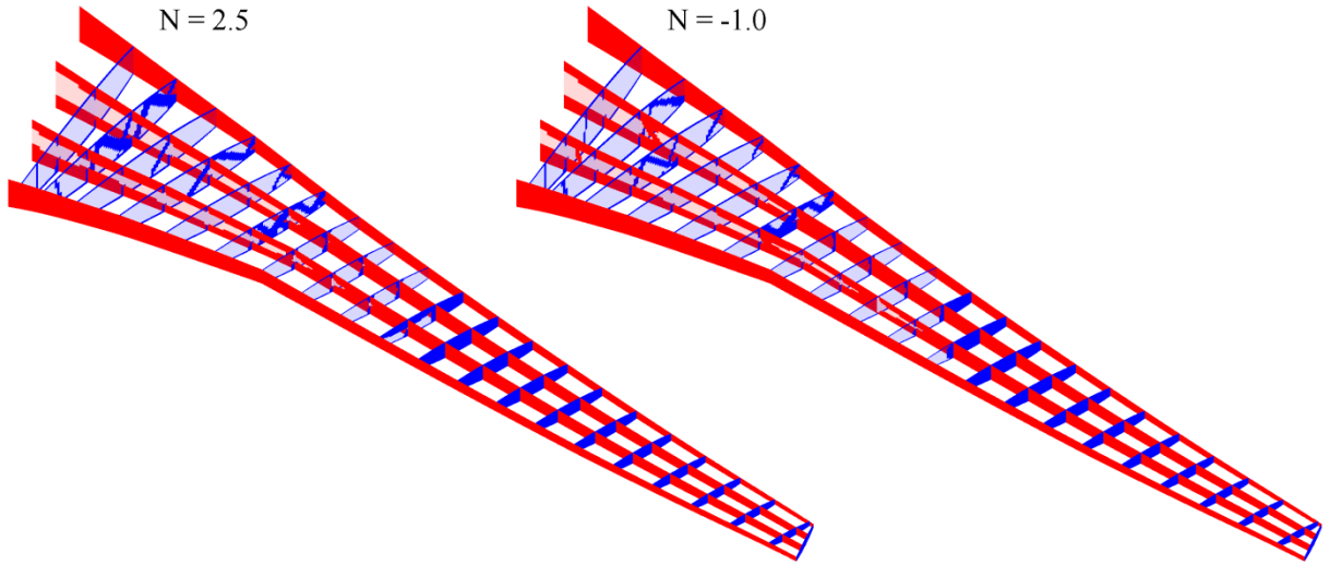
Figure 4. Dependence of compliance-optimal topology upon load factor.
