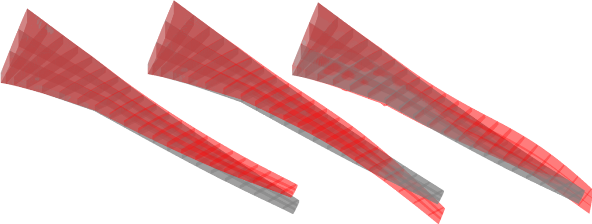
Figure 19. First bending (1B), second bending (2B) and first torsional (1T) mode shapes of the baseline topology.
