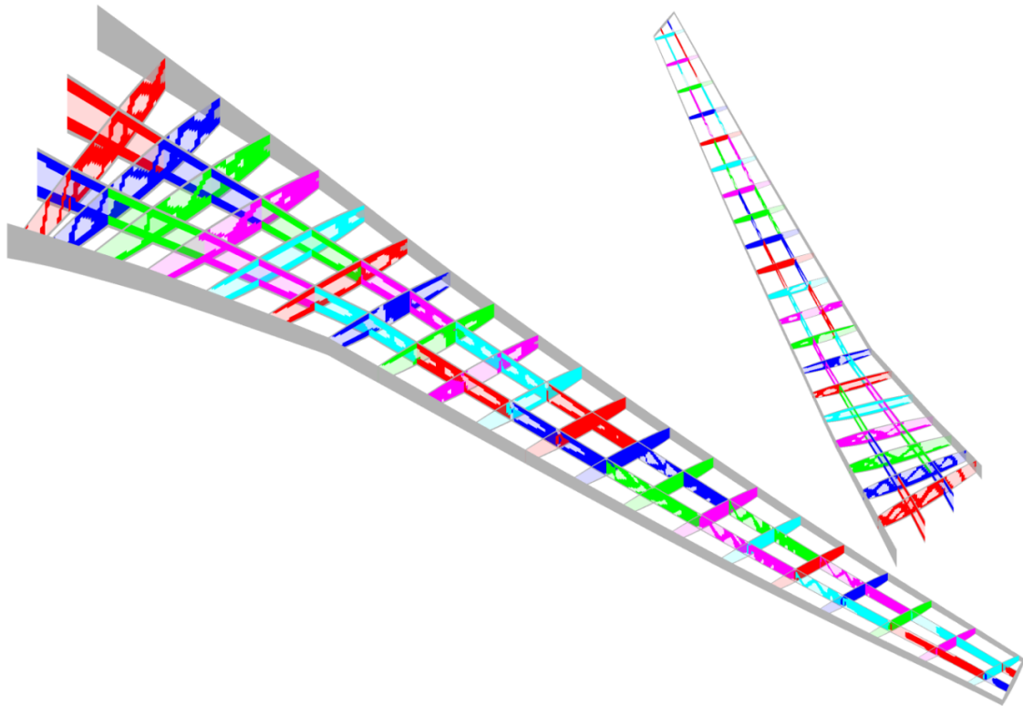
Figure 5. Compliance-optimal topology obtained with multiple volume constraints.
