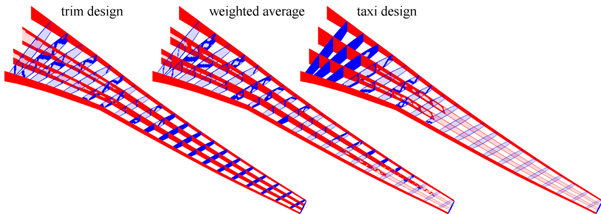
Figure 6. Compliance-optimal topology for aeroelastic trim loads (left), for taxi bump loads (right), and a compromise between the two (center).
