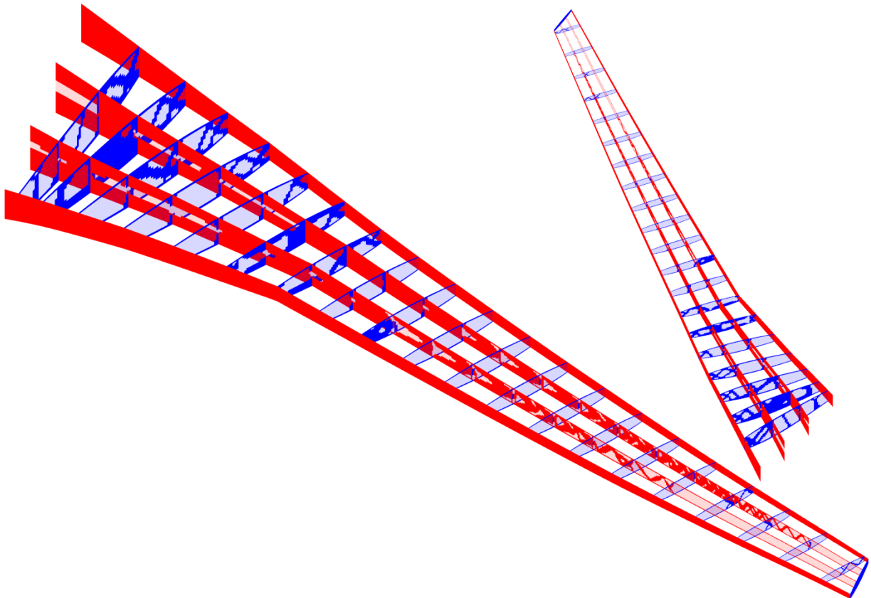
Figure 3. Compliance-optimal topology of the CRM wing box without self-weight loads.
