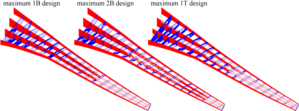
Figure 18. Wing topologies which maximize a specified natural frequency.
