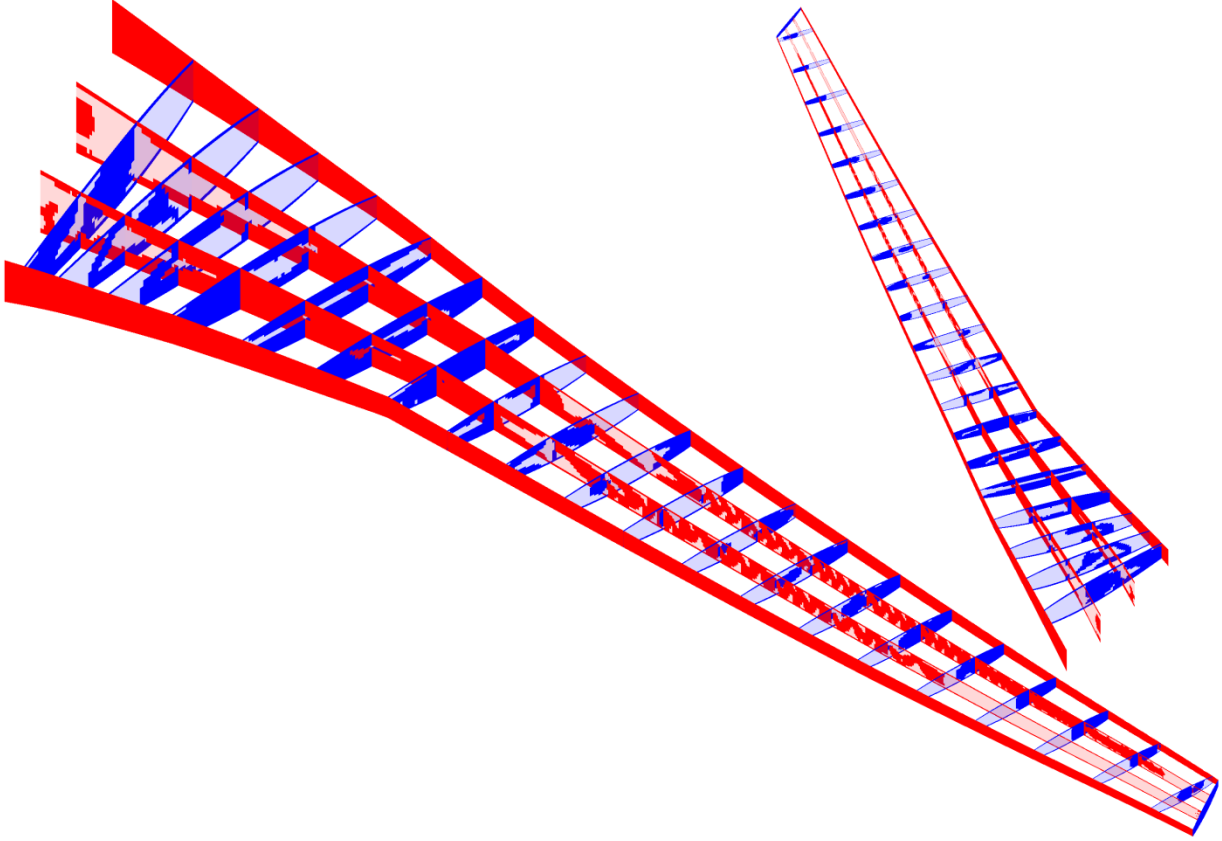
Figure 9. Stress-optimal topology of the CRM wing box.
