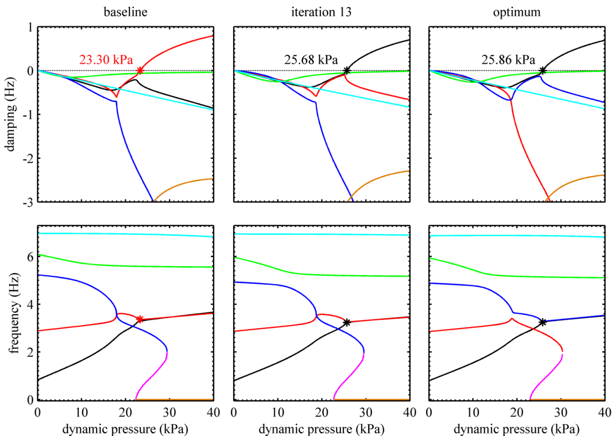
Figure 22. Modal damping (top row) and frequency (bottom row) migration at three different iterations of Figure 21.
