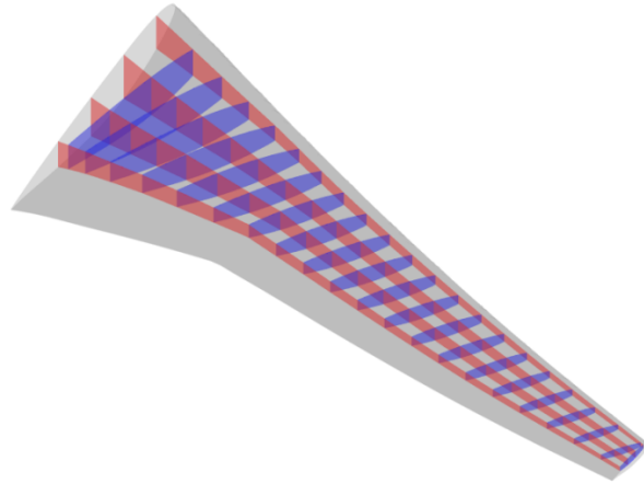
Figure 1. Proposed wing box within the Common Research Model [18].
