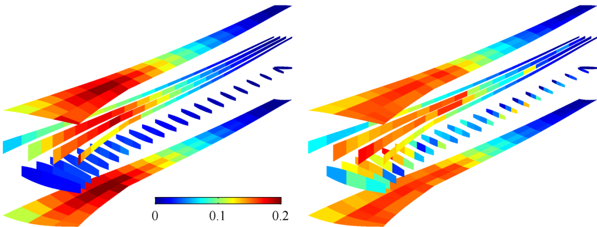
Figure 11. Exploded view of the baseline (left) and optimal (right) p-norm stress measures.
