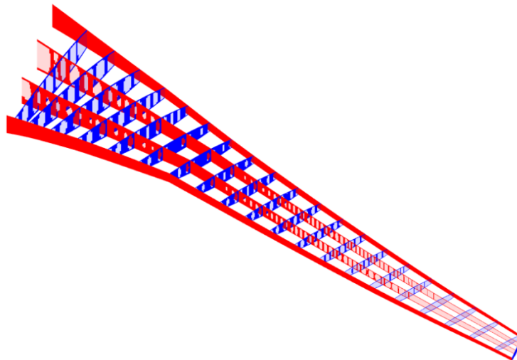
Figure 12. Compliance-optimal topology when only crushing loads are considered.
