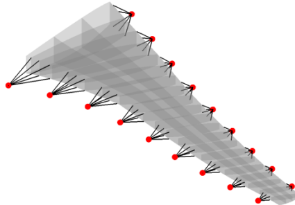
Figure 17. Lumped masses attached to the leading and trailing edges of the wing box.
