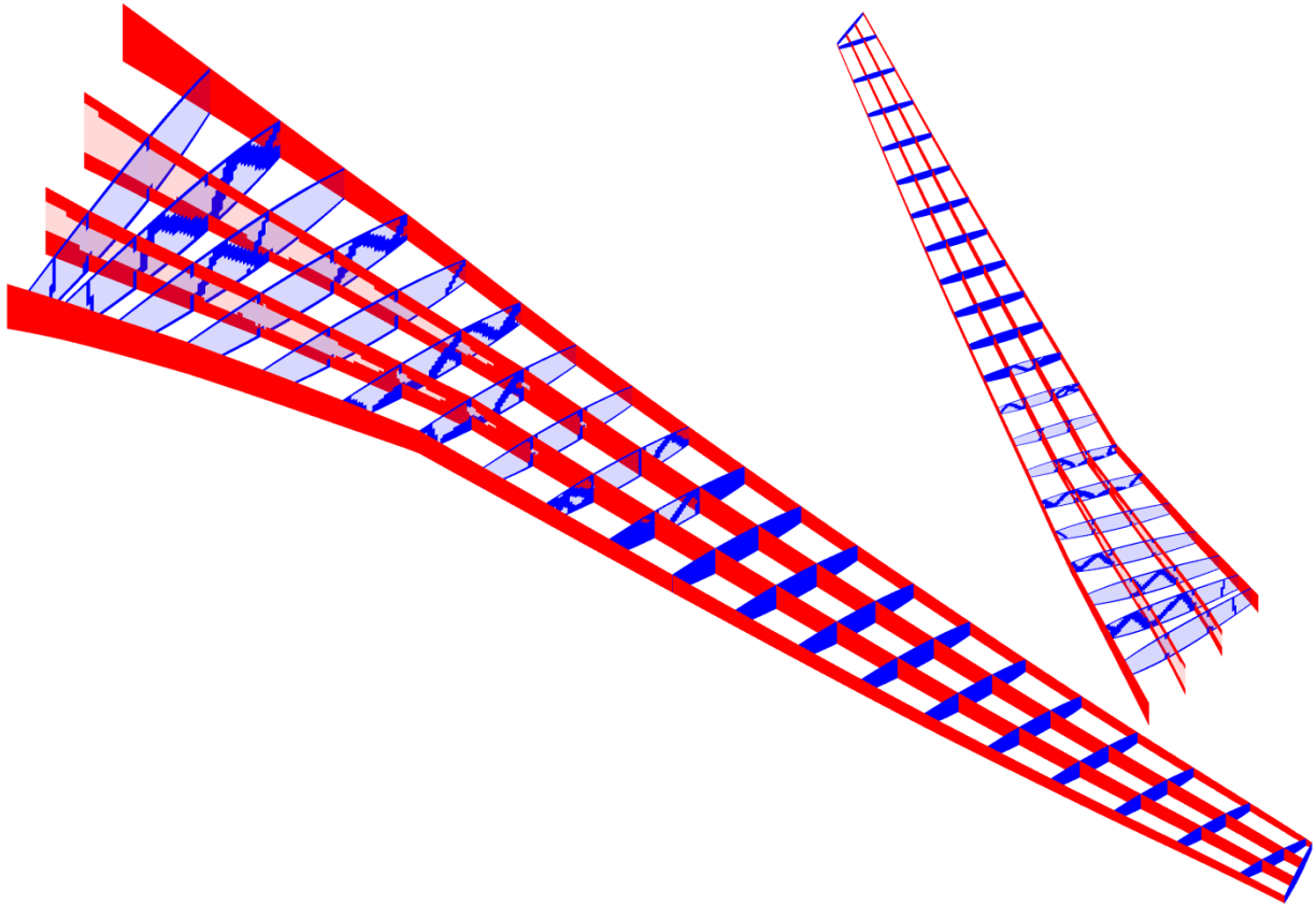
Figure 2. Compliance-optimal topology of the CRM wing box.
