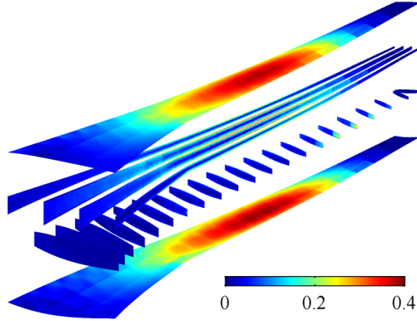
Figure 14. Typical wing stress distribution under a constant roll rate.
