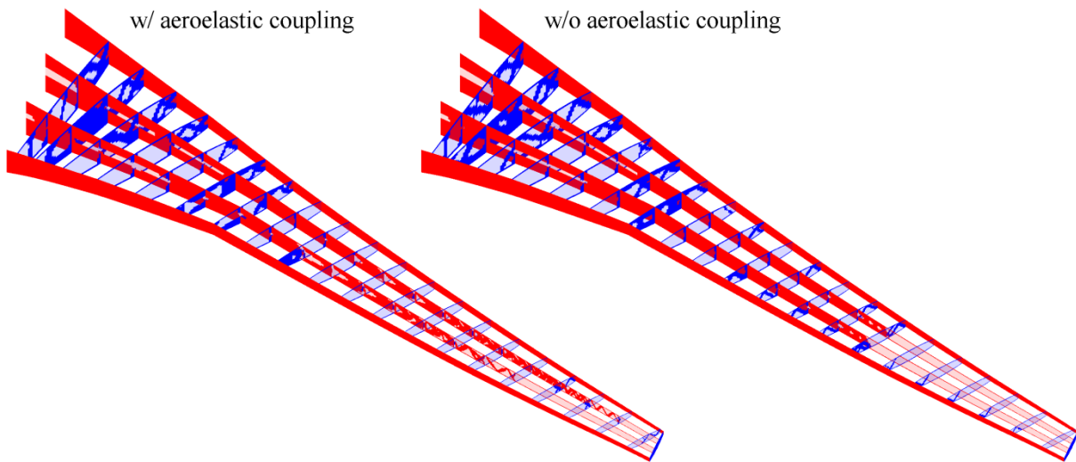
Figure 8. Compliance-optimal topologies with (left) and without (right) aeroelastic coupling.
