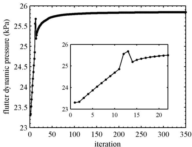
Figure 21. Convergence history of the topology in Figure 20.
