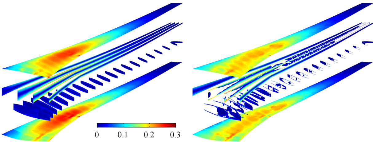
Figure 10. Exploded view of the baseline (left) and optimal (right) von Mises failure indices.
