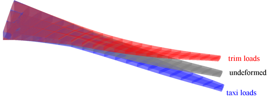
Figure 7. Deformed configurations for the wing topology in Figure 2.
