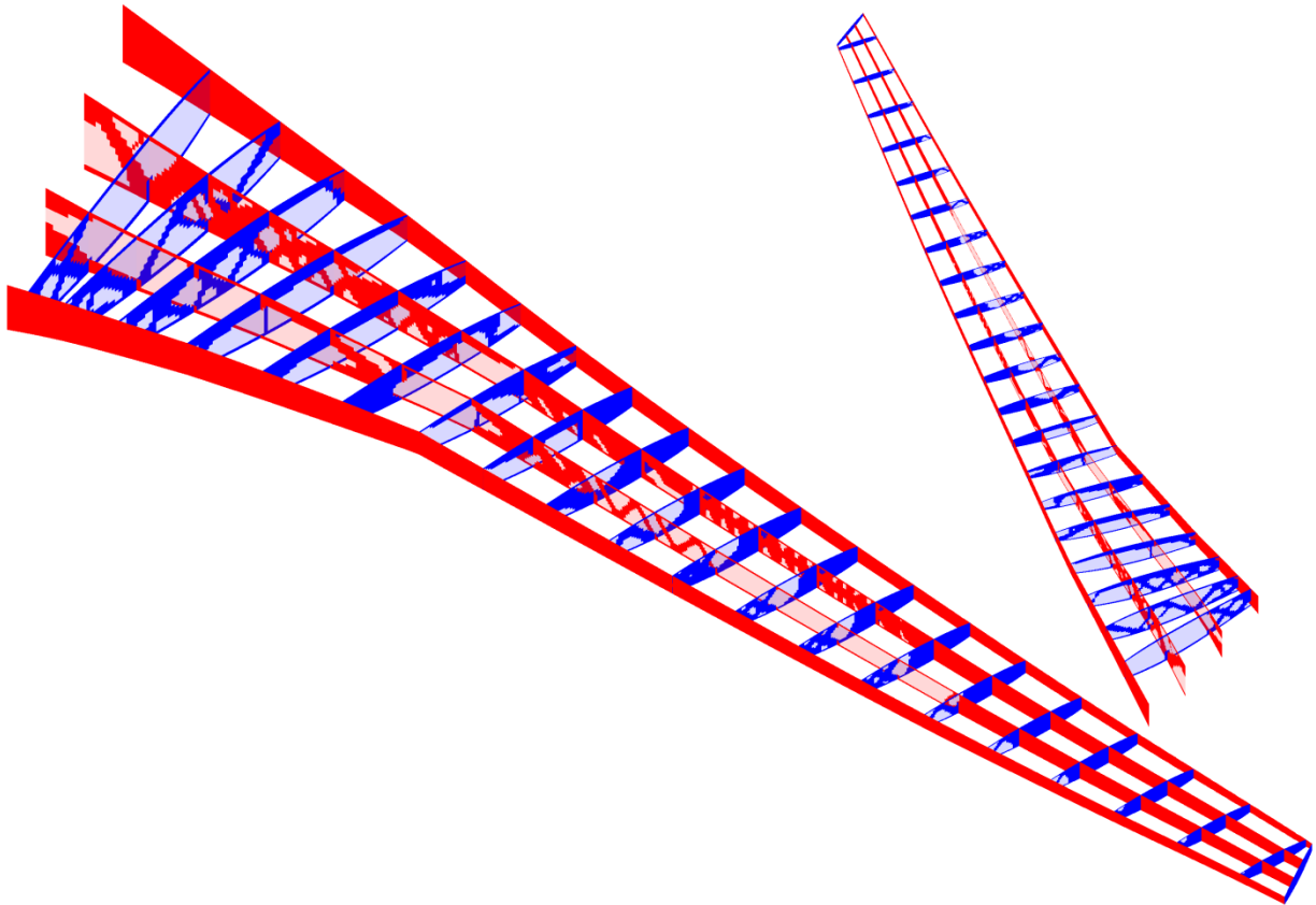
Figure 20. Flutter-optimal topology of the CRM wing box.
