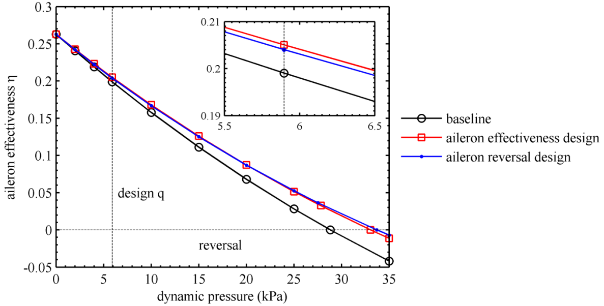
Figure 16. Aileron effectiveness with increasing dynamic pressure.
