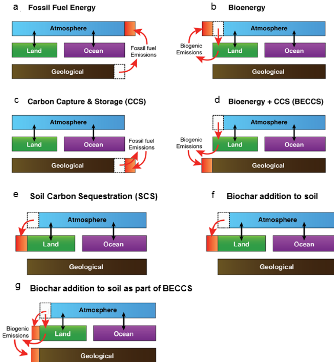
Figure 1. The main flows of carbon among atmospheric, land, ocean and geological reservoirs for fossil fuel combustion (a), BE (b), CCS (c), and the altered carbon flows for BECCS (d), for SCS (e), for biochar addition to soil (f) and for biochar addition to soil as part of BECCS (g). Adapted from Smith et al. (2015).
