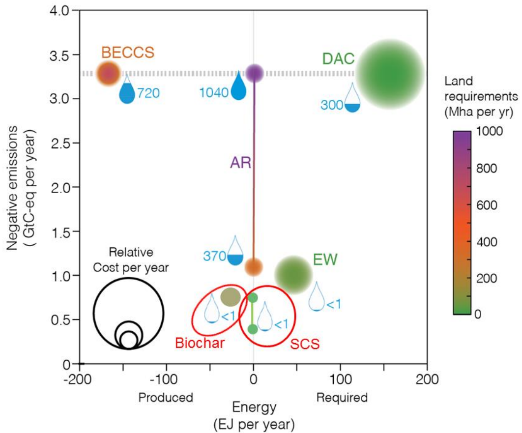
4 5 Figure 3. Comparison of the global impacts of SCS and biochar and other NETs on land use, 6 water, nutrients, albedo, energy and cost. NETs to which SCS and biochar are compared are 7 BECCS, DAC, EW and AR as assessed by Smith et al. (2015). Water requirement shown as 8 water drops with quantities in km 3 /yr; all other units are indicated on the figure. Adapted 9 from Smith et al. (2015).
