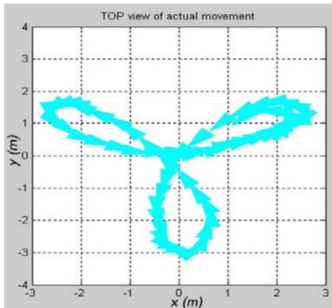
Figure 13 Actual trajectories of the excavator base under various data rates.
