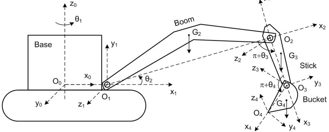
Figure 2 Schematic diagram of an excavator [4]
