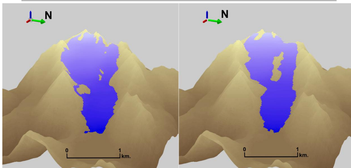
Figure 6. Comparison between the real Griesseglescher surface (left) and the one modelled with user-defined cross-sections (see Figure 15 and text) and IDW interpolation.
