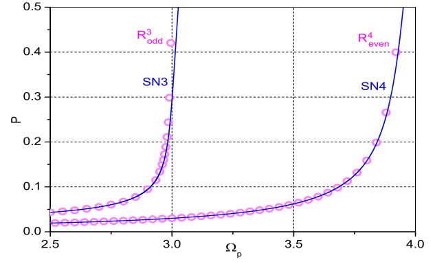
FIG. 5. (Color online). A zoom into the parameter space of the tilted parametric pendulum, representing the red dashed rectangle region indicated in Fig. 3. Melnikov thresholds R_{\text{odd}}^3 and R_{\text{even}}^4 (empty circles) agree finely with the borders of resonance regions SN3 and SN4 (full lines), respectively.
