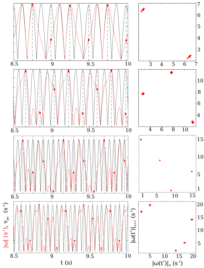
FIG. 2. (Color online). On the left column, from the top to the bottom, we display sampled experimental time series for fixed amplitude A = 2.02\text{cm} illustrating period-2 ( f_p = 4.05 Hz), period-3 ( f_p = 5.35 Hz), period-4 ( f_p = 7.5 Hz), and period-5 ( f_p = 8.55 Hz) oscillations. Full red lines represent the modulus of the pendulum angular velocity, |\omega| , and full black lines the time series for the modulus of perturbation velocity normalized with respect to the maximum value of |\omega| , v_{pm} . Full red circles are the values of the pendulum velocity each time the perturbation completes a full cycle. On the right column we have the corresponding stroboscopic maps for each time series.
