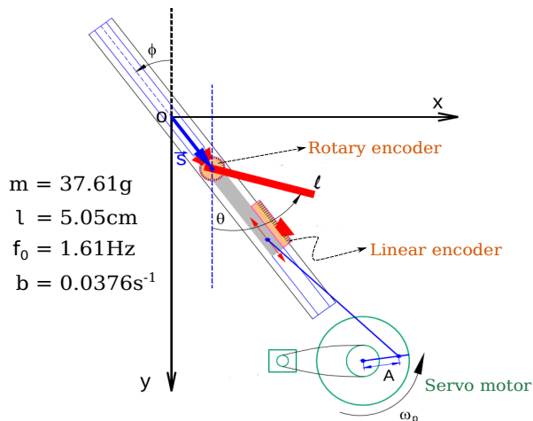
FIG. 1. (Color online). Diagram of the experimental apparatus of a planar simple pendulum parametrically excited along an arbitrary direction. The pendulum pivot axis is attached to a sliding car that is forced to oscillate with amplitude A and frequency f_p , with the help of a crank and a servo motor. We can measure simultaneously the absolute value of the pivot speed v_p , with a linear encoder system in the laboratory reference frame, and the absolute value of the pendulum angular velocity |\omega| , with a rotary encoder system attached to the pendulum.
