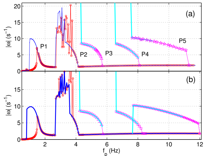
FIG. 4. (Color online). Bifurcation diagrams at A = 2.02 cm obtained (a) experimentally and (b) numerically. Frequency of the excitation was spanned both forward (line with empty circles) and backwards (full line). Periodic oscillations P3, P4, and P5 are excited by manually setting up initial conditions of the pendulum and are displayed in triangles, squares, and stars, respectively, for forward frequency sweeping and in full lines for backward sweeping.
