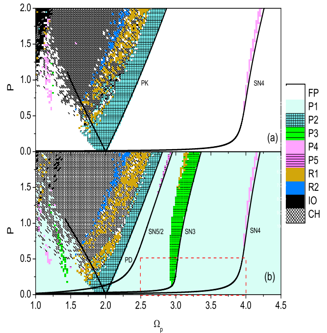
FIG. 3. (Color online). Parameter spaces for (a) vertical ( \phi = 0 ) and (b) tilted ( \phi = \pi/8 ) excitations. FP denotes fixed point; Pm and Rm, period- m [42] oscillation and rotation, respectively; IO periodic inverted oscillations; and CH persistent tumbling chaos [27]. Full lines represent the loci of saddle-node (SN), pitchfork (PK), and period-doubling (PD) bifurcations and were obtained with the software AUTO 07p [54, 55]. See the Supplemental for the numerical code [56].
