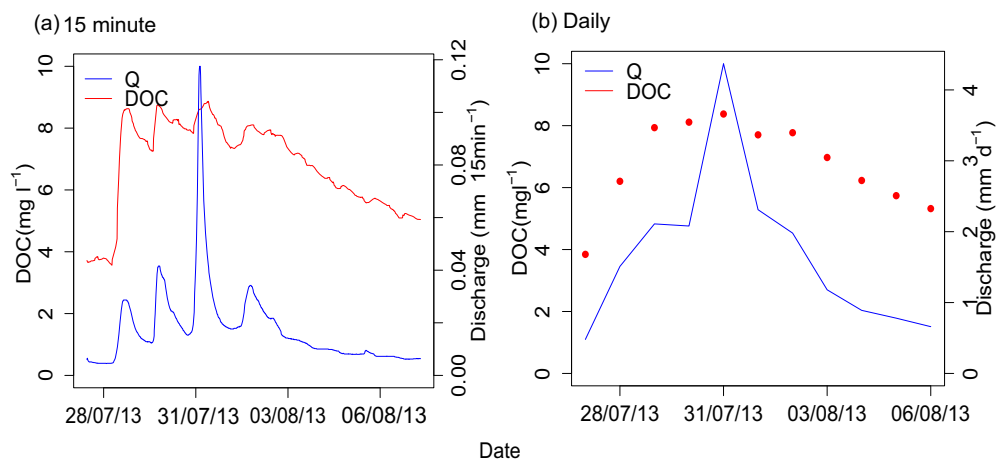
Figure 5. Time series of DOC and discharge for (a) 15 min data and (b) daily data, during an event following a 10 year return period drought at the end of July 2013.
