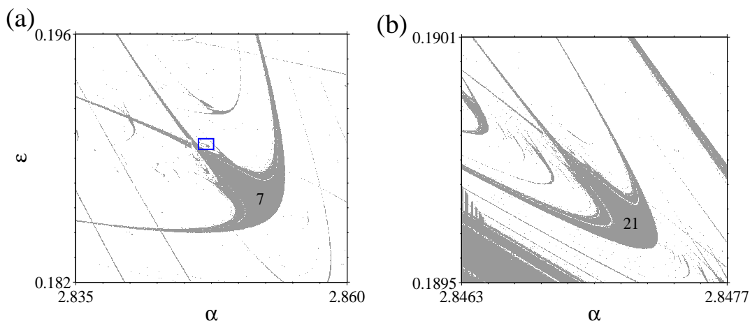
Figure 6: (Color online) (a) Parameter plane diagram showing magnification of the periodic structure with period 7 plotted in black in Fig. 4(a). (b) Magnification of box in blue shown in (a).
