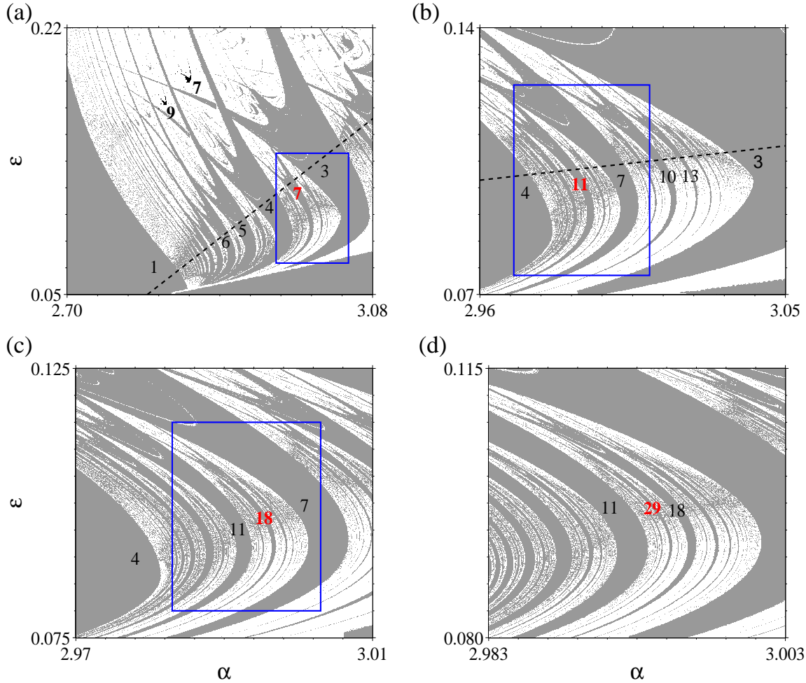
Figure 4: (Color online) (a) Parameter plane diagram for \varepsilon versus \alpha . Periodic solutions are plotted in light gray. (b)-(d) Successive magnifications of boxes in blue shown in (a,b,c).
