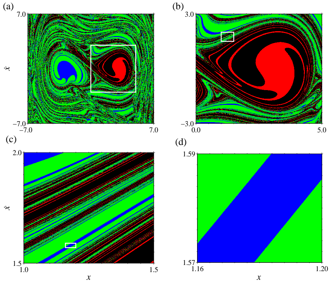
Figure 8: (Color online) Basins of attraction for the attractors shown in Fig. 7 and successive magnifications of boxes in white for the parameters \alpha = 3.25 and \varepsilon = 0.13 , varying initial conditions \dot{x} and x with \dot{\varphi} = 0.0 and \varphi = 0.0 .
