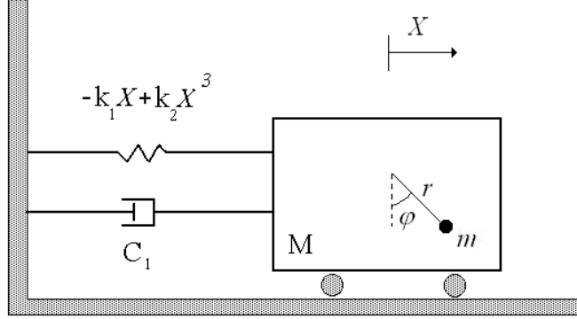
Figure 1: Schematic model of the non-ideal oscillator.
