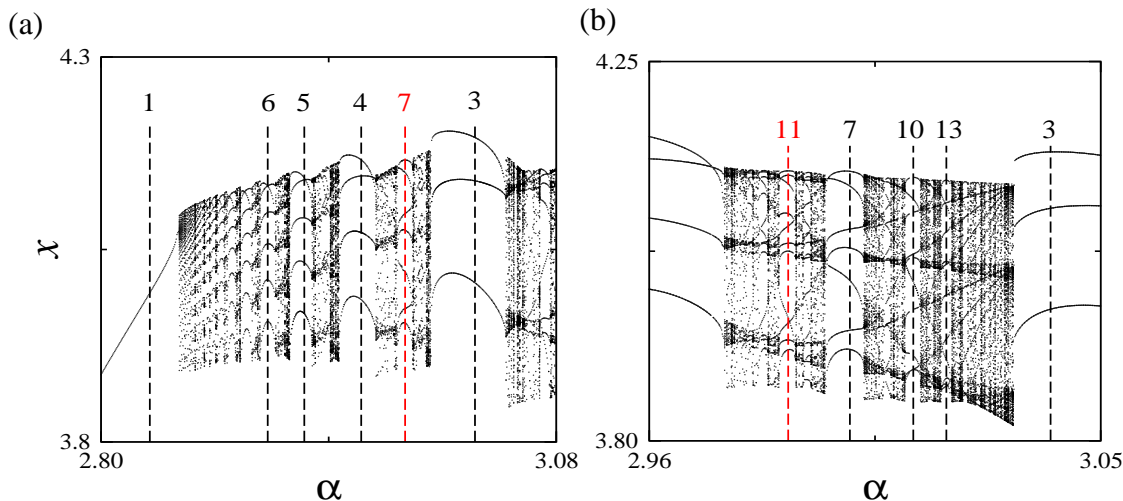
Figure 5: (Color online) Bifurcation diagrams for x in terms of \alpha with (a) \varepsilon = 0.4\alpha - 1.08 (dashed line shown in Fig. 4a) and (b) \varepsilon = 0.1\alpha - 0.196 (dashed line shown in Fig. 4b).
