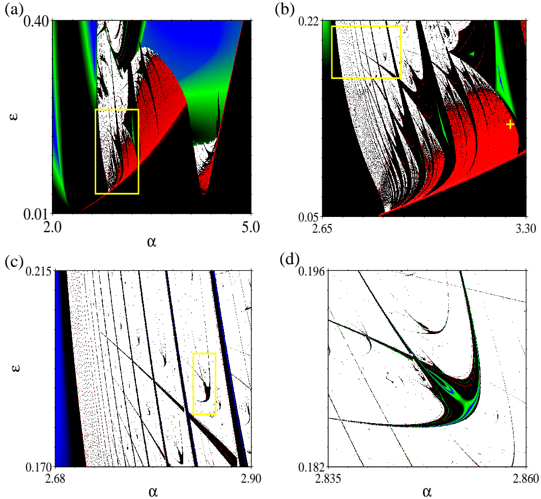
Figure 3: (Color online) (a) Parameter plane diagram for \varepsilon versus \alpha . Periodic solutions are plotted in blue, green and black scale ranges, quasi-periodic in red, and chaotic in white. (b)-(d) Successive magnifications of boxes in yellow shown in (a,b,c).
