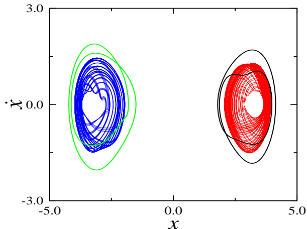
Figure 7: (Color online) Phase portrait of velocity versus displacement of four coexisting attractors for the parameters \alpha = 3.25 and \varepsilon = 0.13 . Two periodic attractors plotted in green and black, two quasi-periodic in blue and red.
