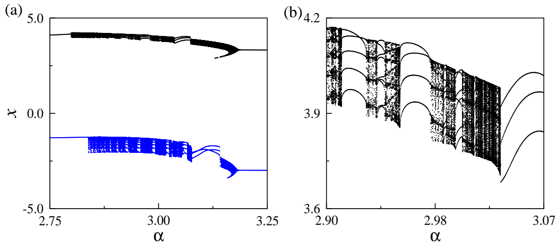
Figure 2: (Color online) (a) Bifurcation diagram showing coexisting attractors for x in terms of \alpha with \varepsilon = 0.09 . (b) Magnification of bifurcation diagram for the attractors plotted in black.
