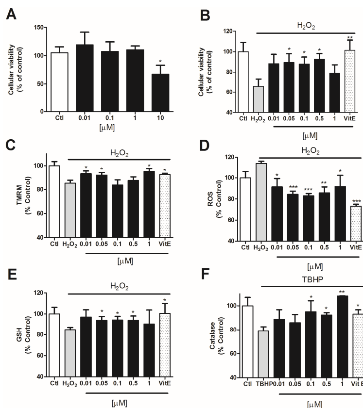
Figure 5. Makaluvamine J (5) effect over SHSY5Y cells pretreated with H 2 O 2 . Vitamin E was added as a positive control. (A) Cytotoxicity of compound 5 over neuroblastoma cells; (B) Neuroprotective effect of compound 5 in the presence of 150 μM H 2 O 2 after 6 h incubation; (C) Effect of compound 5 co-incubation on ΔΨ m measured by TMRM assay; (D) Compound 5 inhibition of ROS release versus H 2 O 2 treated cells; (E,F) Evaluation of GSH and catalase activity after 6 h incubation with 150 μM H 2 O 2 . GSH levels measured by ThiolTracker Violet (E) and catalase activity measured by Catalase Amplex Red kit (Invitrogen) (F). The values are presented in percentage versus non-treated control cells and compared to cells treated with 150 μM H 2 O 2 alone. * p < 0.05 and ** p < 0.01.
