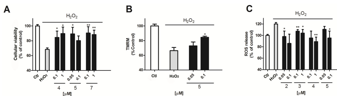
Figure 3. Effect of makaluvamines over H_2O_2 toxicity and ROS release (A) Neuroprotective effect of compound 4 and 5 in the presence of 200 \mu M H_2O_2 after 12 h incubation; (B) Effect of Compound 5 co-incubation over \Delta\Psi_m measured by tetramethylrhodamine (TMRM) assay; (C) Compounds 2, 3, 4, and 5 at \mu M concentrations (0.05, 0.1 and 1 \mu M ) inhibited ROS release versus H_2O_2 treated cells. The values are presented in percentage versus non-treated control cells, but the statistical comparison is made versus H_2O_2 treated cells. * p < 0.05 and ** p < 0.01 . Data are mean \pm SEM of three or more independent experiments performed in triplicate.
