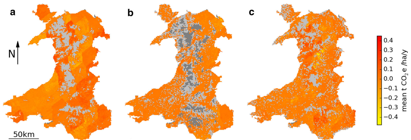
Fig. 4 Simulated change in annual GHG flux (effective \text{t CO}_2\text{e ha}^{-1} \text{y}^{-1} ) from Welsh fertilized grassland (a), fertilized arable (b) and forest (c) between baseline and high climate change scenario. Light grey areas show zero change; dark grey areas show zero land cover
