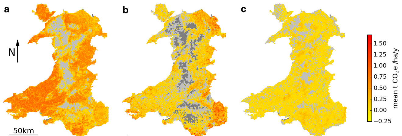
Fig. 2 Simulated mean annual net GHG fluxes (effective t CO 2 e ha -1 y -1 ) from Welsh fertilized grassland ( a ), fertilized arable land ( b ) and forest ( c ), at baseline climate (1961–1990). Results are for emissions per hectare of the specified land cover in each grid cell,
